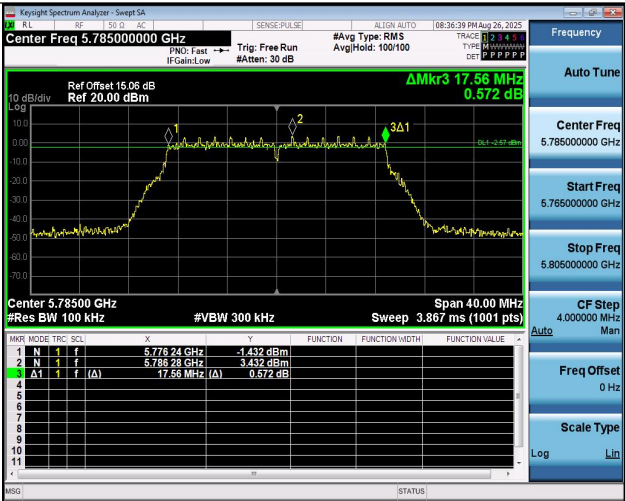
11N20MIMO-Ant2-5785-PASS
