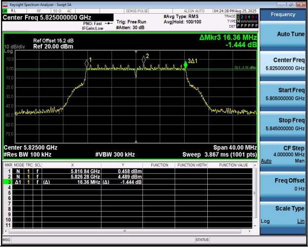
11A-Ant2-5825-PASS
