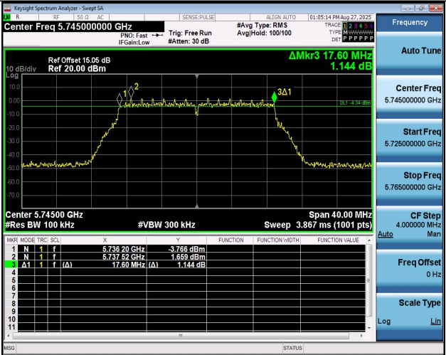
11AC20MIMO-Ant2-5745-PASS
