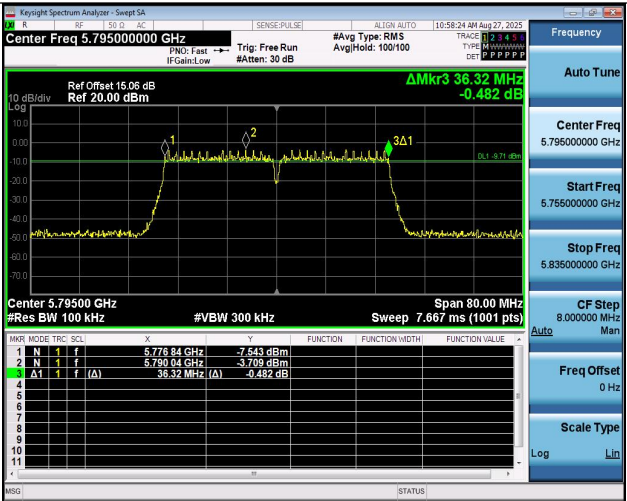
11N40MIMO-Ant2-5795-PASS
