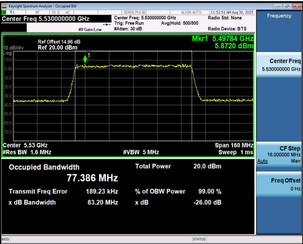
11BE80MIMO-Ant2-5530
