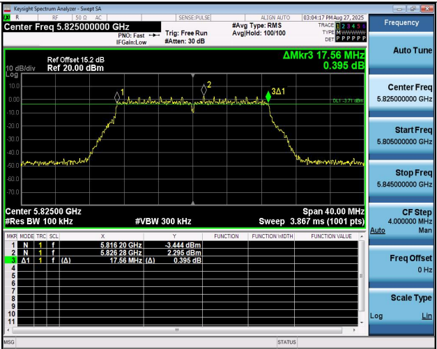
11AC20MIMO-Ant2-5825-PASS
