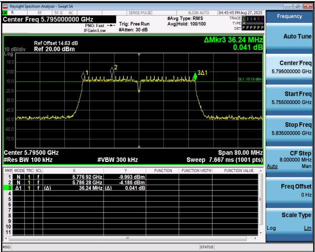
11AC40MIMO-Ant1-5795-PASS
