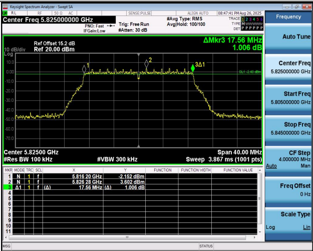
11N20MIMO-Ant2-5825-PASS
