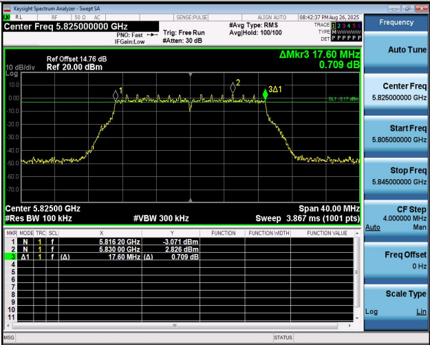
11N20MIMO-Ant1-5825-PASS
