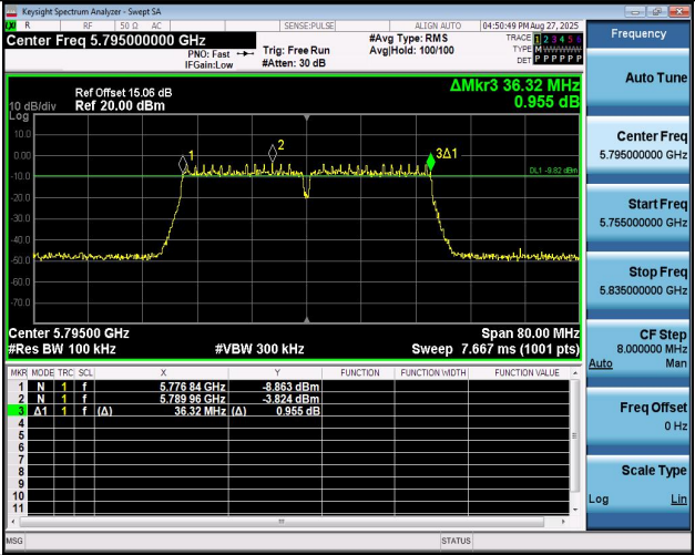
11AC40MIMO-Ant2-5795-PASS
