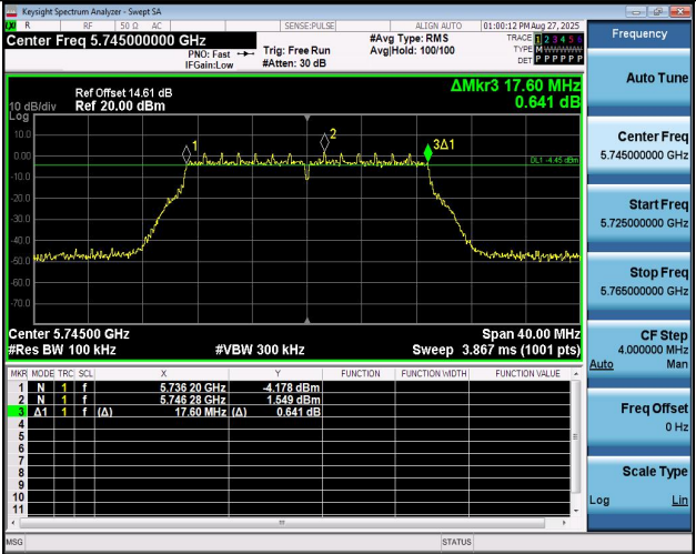
11AC20MIMO-Ant1-5745-PASS
