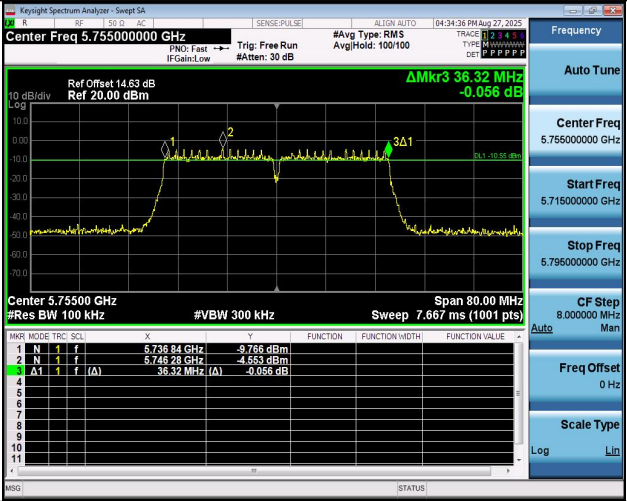
11AC40MIMO-Ant1-5755-PASS
