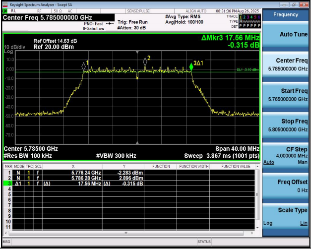
11N20MIMO-Ant1-5785-PASS
