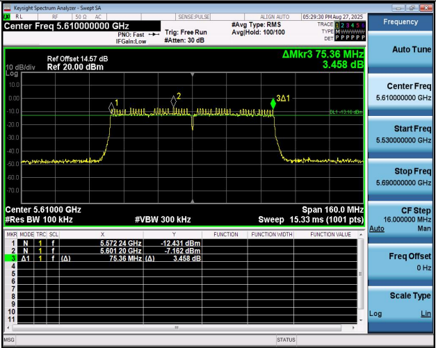
11AC80MIMO-Ant1-5610-PASS
