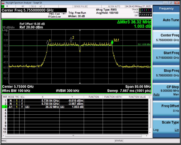
11AC40MIMO-Ant2-5755-PASS
