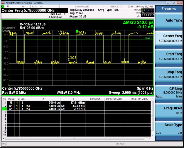
NTNV-11A-Ant1-5785
