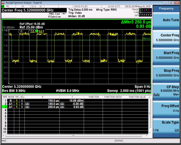
NTNV-11N20MIMO-Ant2-5320
