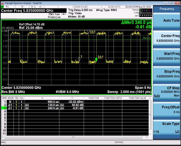
NTNV-11A-Ant1-5825
