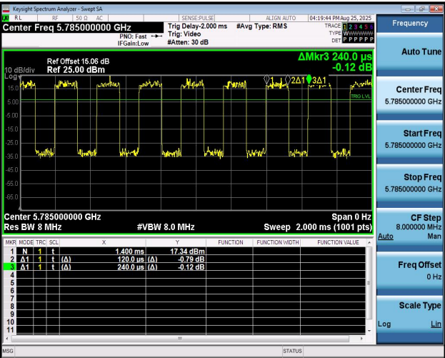
NTNV-11A-Ant2-5785
