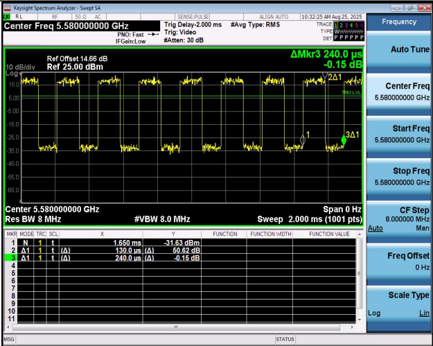
NTNV-11A-Ant1-5580
