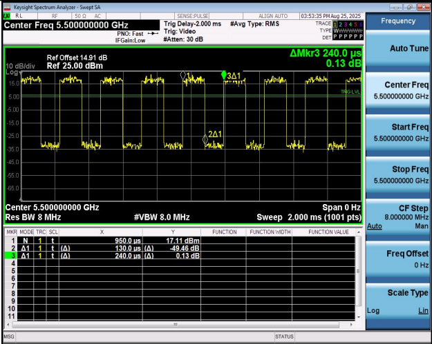
NTNV-11A-Ant2-5500
