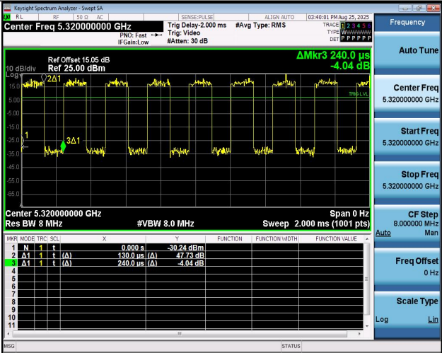
NTNV-11A-Ant2-5320
