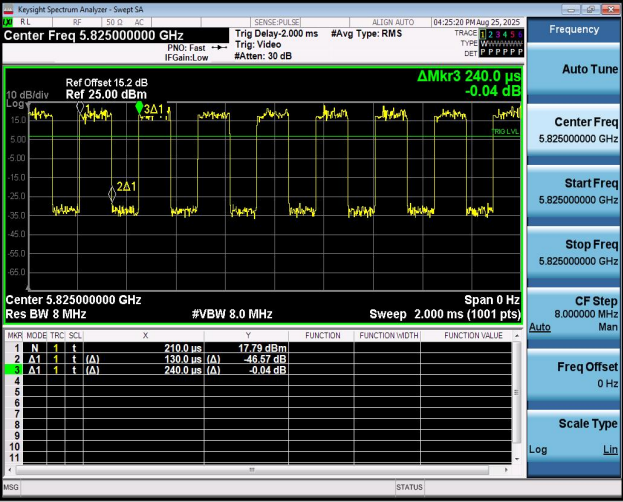
NTNV-11A-Ant2-5825
