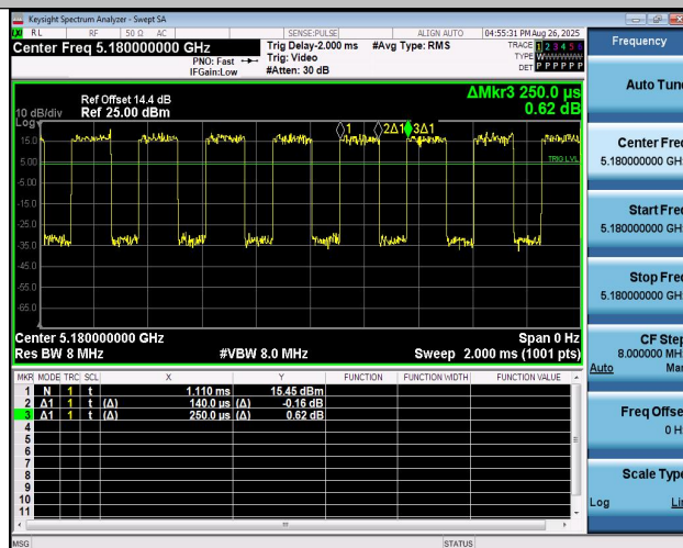
NTNV-11N20MIMO-Ant2-5180
