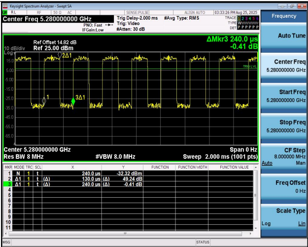
NTNV-11A-Ant2-5280
