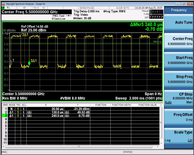
NTNV-11A-Ant1-5500
