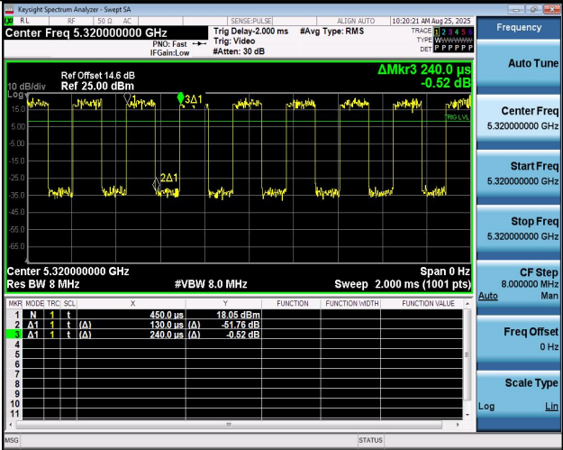
NTNV-11A-Ant1-5320
