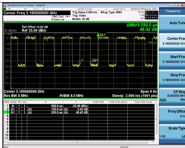
NTNV-11N20MIMO-Ant1-5180
