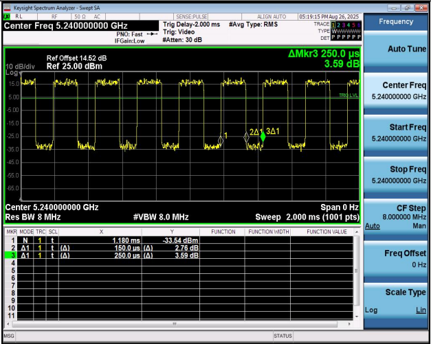
NTNV-11N20MIMO-Ant2-5240
