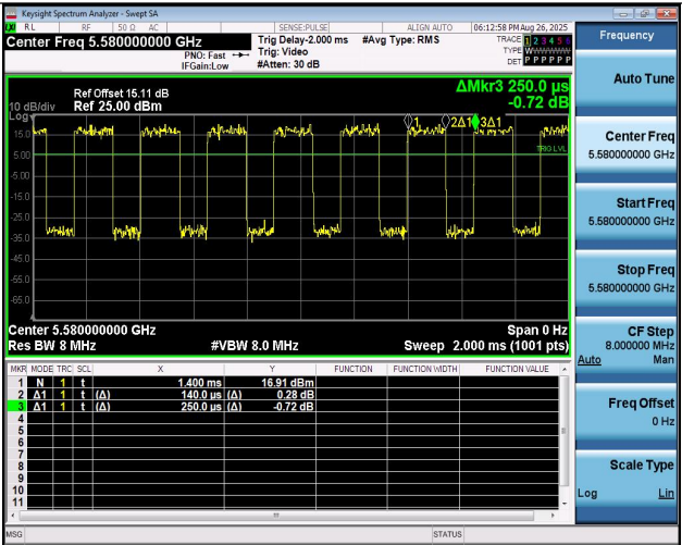
NTNV-11N20MIMO-Ant2-5580
