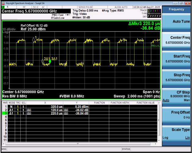
NTNV-11N40MIMO-Ant2-5670
