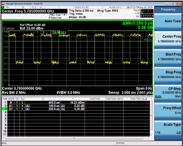
NTNV-11N20MIMO-Ant2-5785
