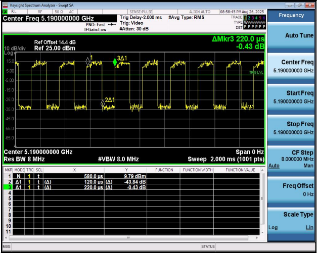
NTNV-11N40MIMO-Ant2-5190
