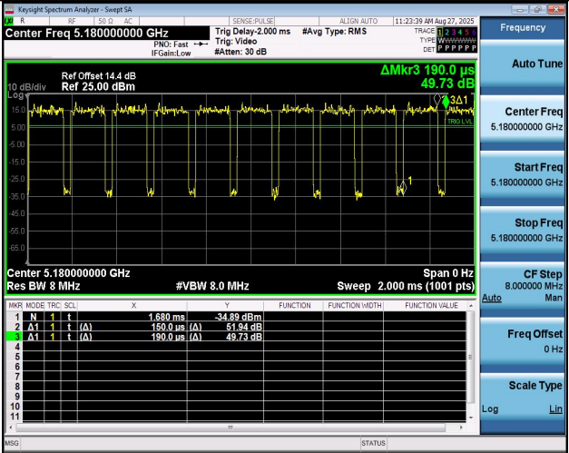
NTNV-11AC20MIMO-Ant2-5180
