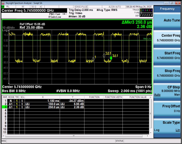
NTNV-11N20MIMO-Ant2-5745
