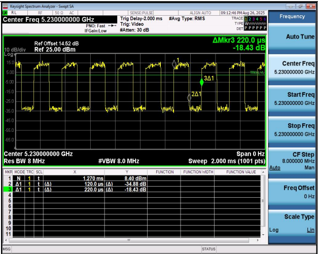
NTNV-11N40MIMO-Ant2-5230
