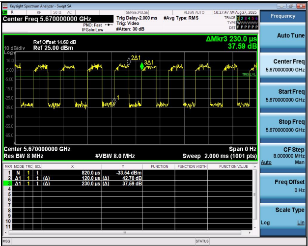
NTNV-11N40MIMO-Ant1-5670
