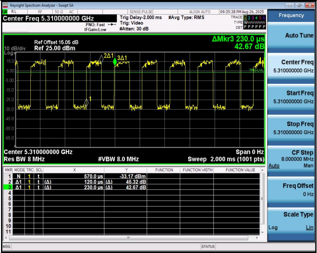
NTNV-11N40MIMO-Ant2-5310
