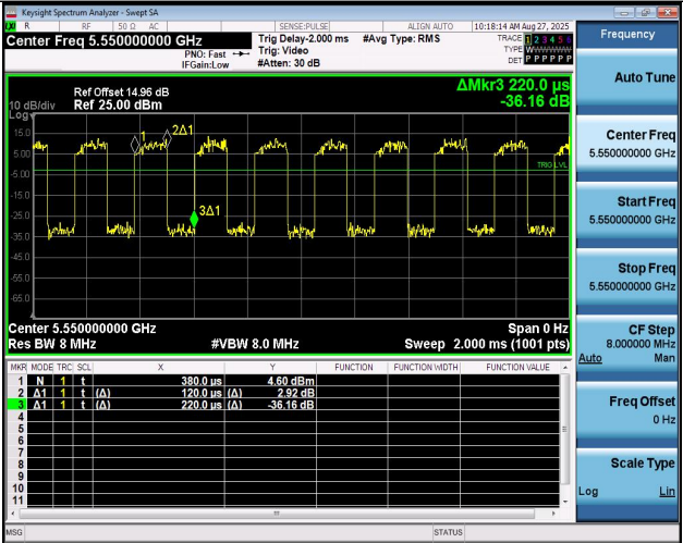
NTNV-11N40MIMO-Ant2-5550
