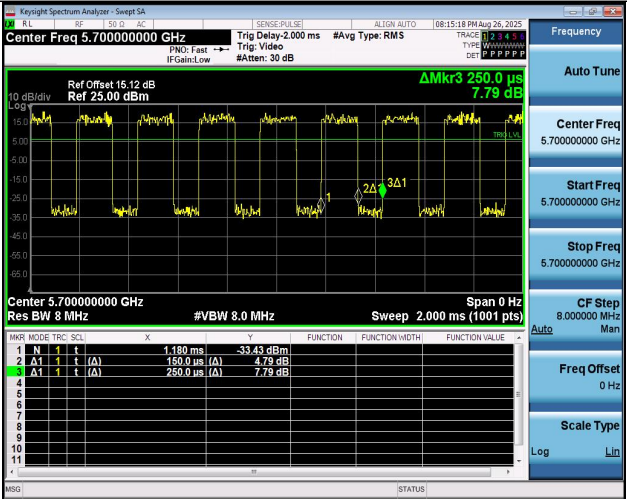
NTNV-11N20MIMO-Ant2-5700
