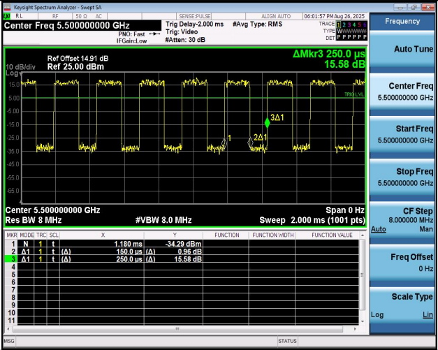
NTNV-11N20MIMO-Ant2-5500
