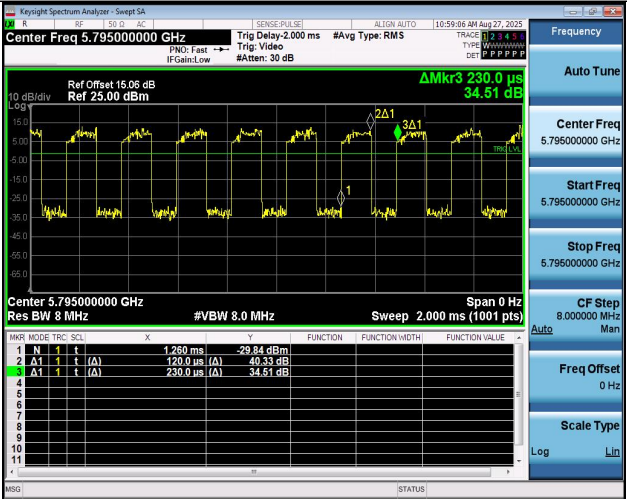
NTNV-11N40MIMO-Ant2-5795
