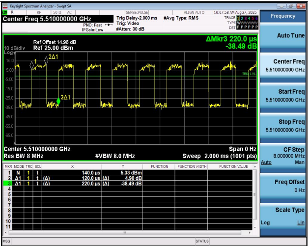
NTNV-11N40MIMO-Ant2-5510
