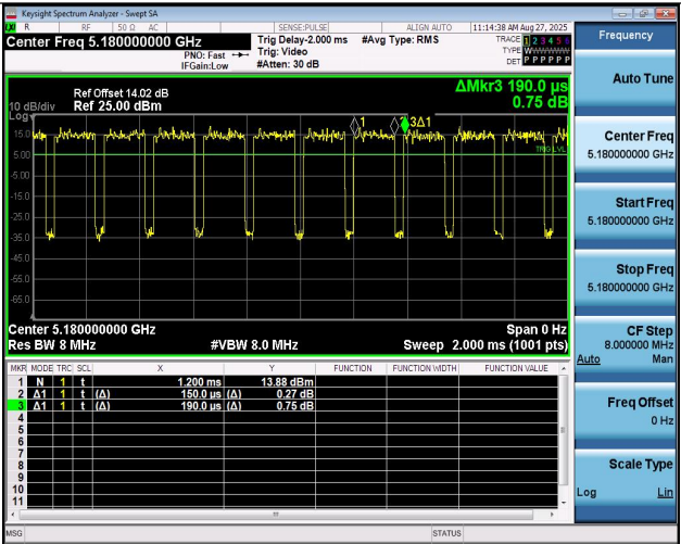
NTNV-11AC20MIMO-Ant1-5180
