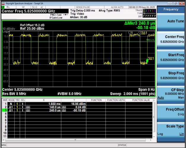
NTNV-11N20MIMO-Ant2-5825
