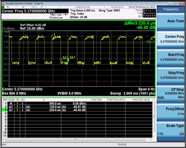
NTNV-11N40MIMO-Ant2-5270
