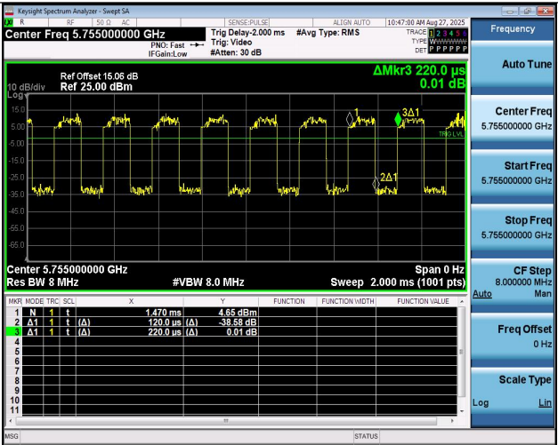
NTNV-11N40MIMO-Ant2-5755
