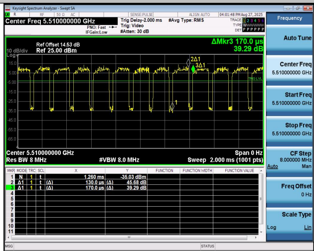
NTNV-11AC40MIMO-Ant1-5510
