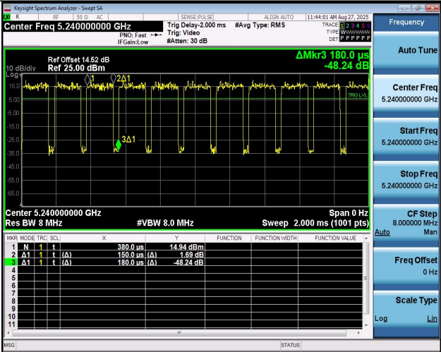
NTNV-11AC20MIMO-Ant2-5240
