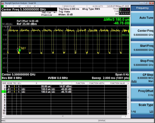
NTNV-11AC20MIMO-Ant1-5500
