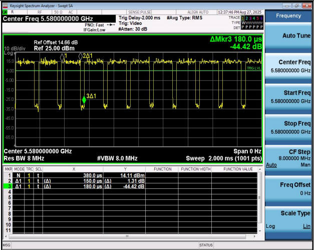
NTNV-11AC20MIMO-Ant1-5580
