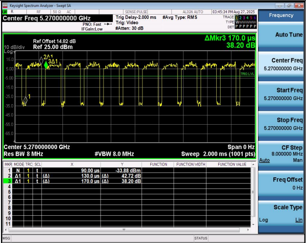
NTNV-11AC40MIMO-Ant2-5270
