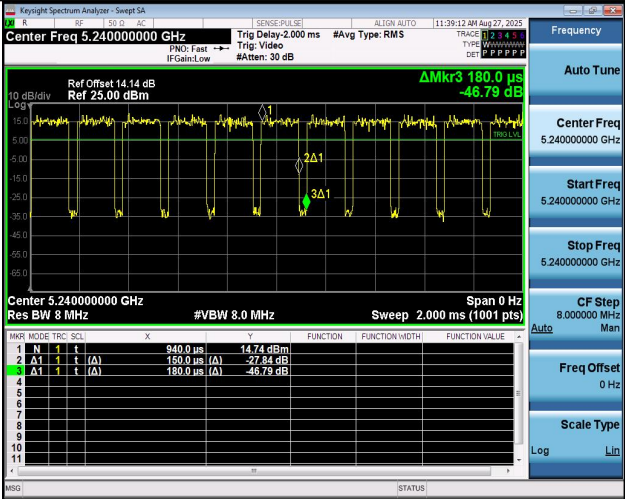
NTNV-11AC20MIMO-Ant1-5240
