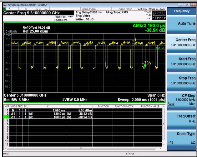
NTNV-11AC40MIMO-Ant2-5310
