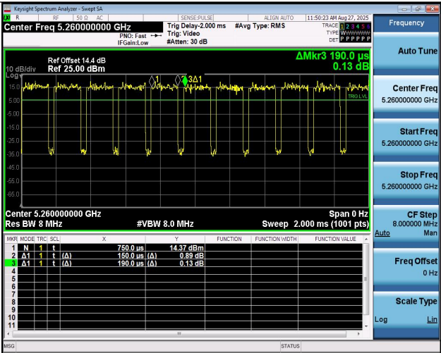
NTNV-11AC20MIMO-Ant1-5260
