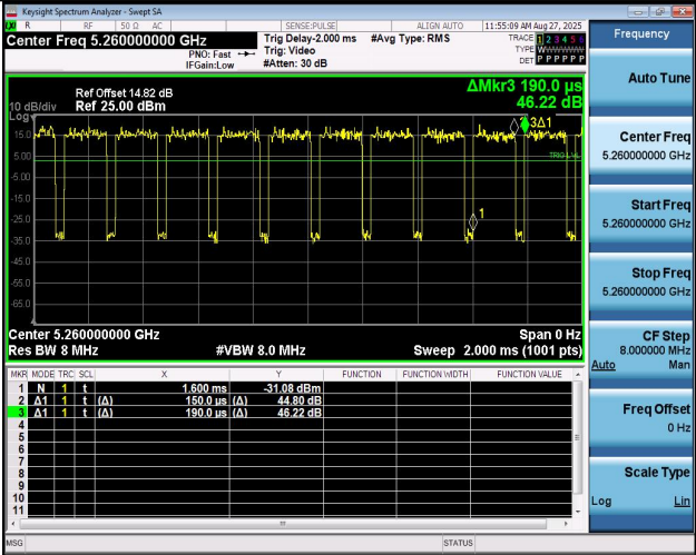
NTNV-11AC20MIMO-Ant2-5260
