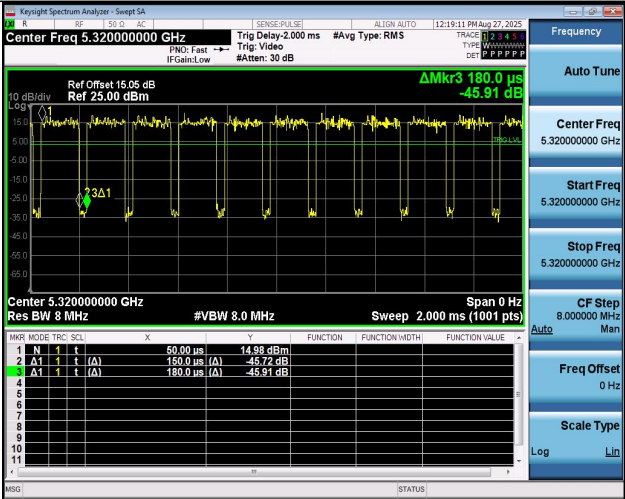
NTNV-11AC20MIMO-Ant2-5320
