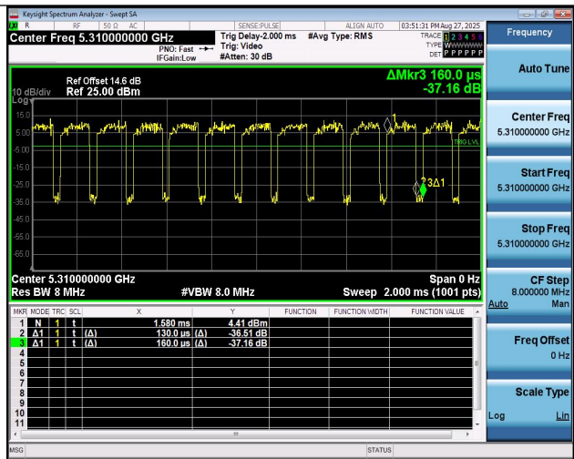
NTNV-11AC40MIMO-Ant1-5310
