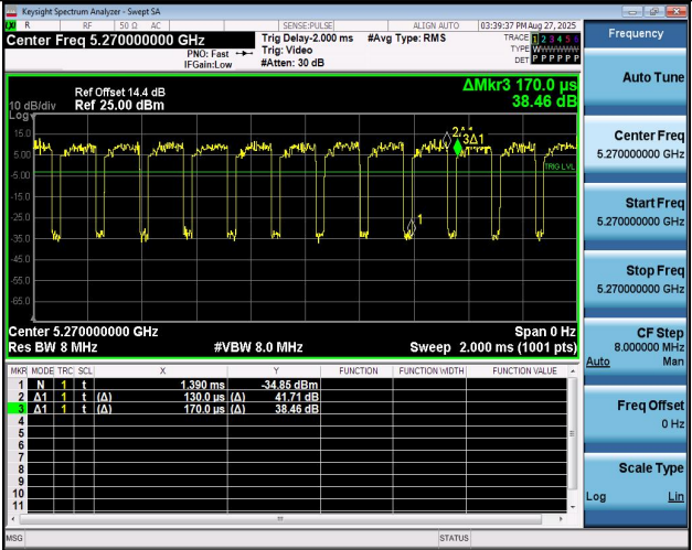
NTNV-11AC40MIMO-Ant1-5270
