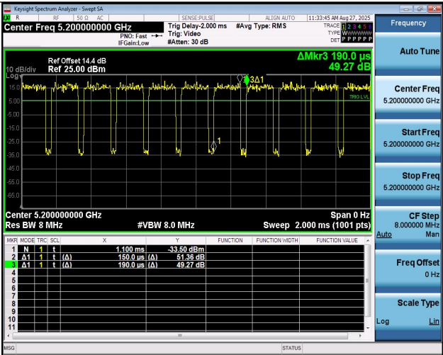
NTNV-11AC20MIMO-Ant2-5200
