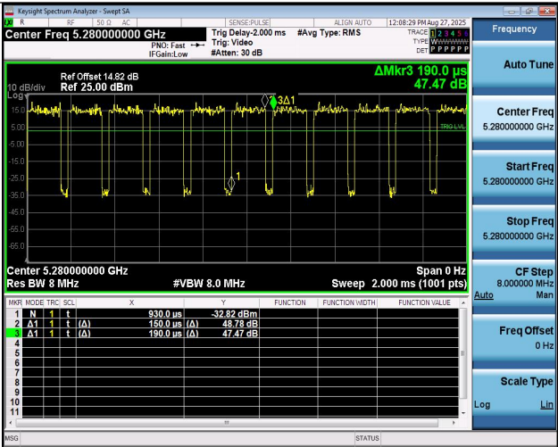
NTNV-11AC20MIMO-Ant2-5280
