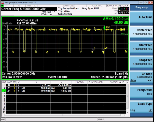
NTNV-11AC20MIMO-Ant2-5500
