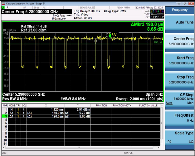
NTNV-11AC20MIMO-Ant1-5280
