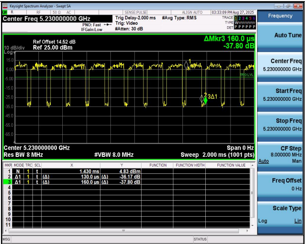
NTNV-11AC40MIMO-Ant2-5230
