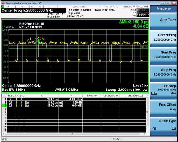
NTNV-11AC160MIMO-Ant1-5250
