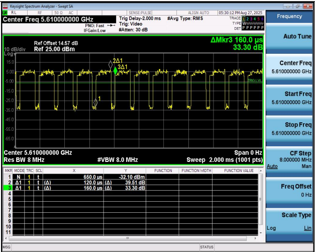
NTNV-11AC80MIMO-Ant1-5610
