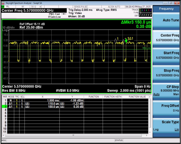
NTNV-11AC160MIMO-Ant2-5570
