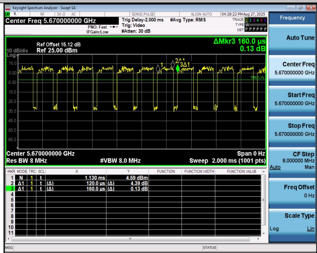
NTNV-11AC40MIMO-Ant2-5670
