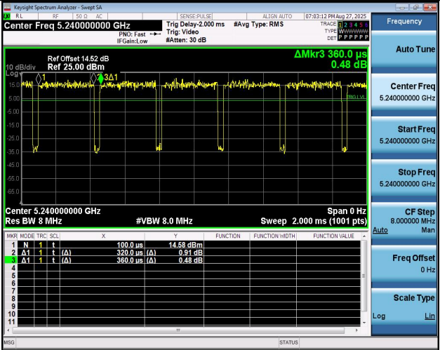
NTNV-11AX20MIMO-Ant2-5240
