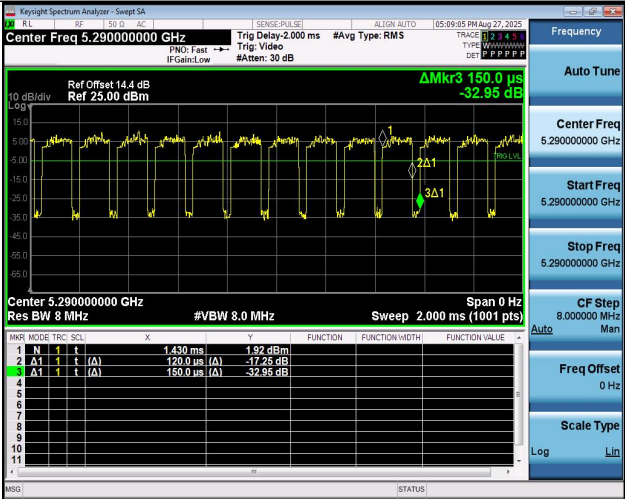
NTNV-11AC80MIMO-Ant1-5290
