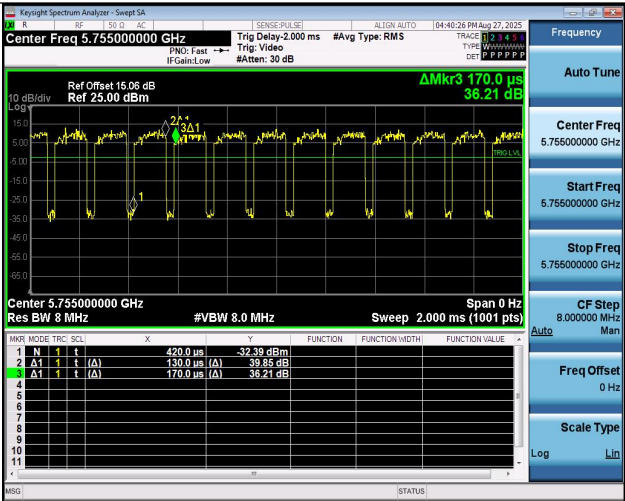
NTNV-11AC40MIMO-Ant2-5755
