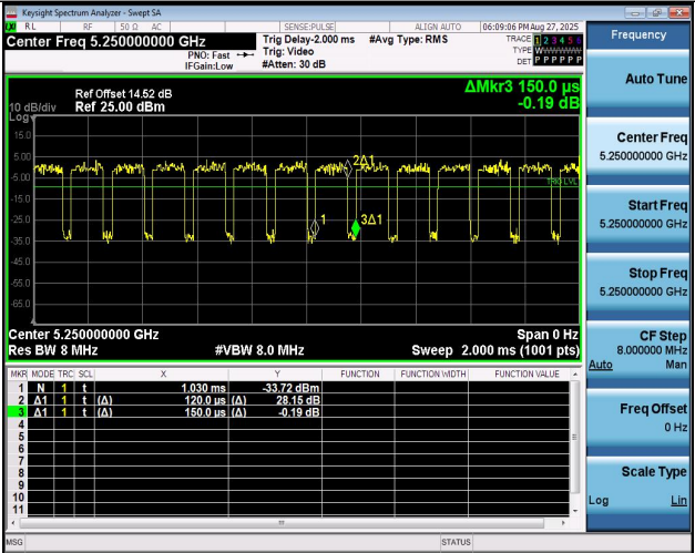
NTNV-11AC160MIMO-Ant2-5250
