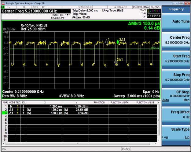
NTNV-11AC80MIMO-Ant2-5210
