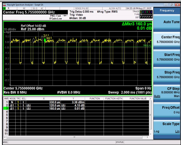
NTNV-11AC40MIMO-Ant1-5755
