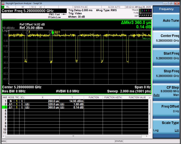
NTNV-11AX20MIMO-Ant2-5280
