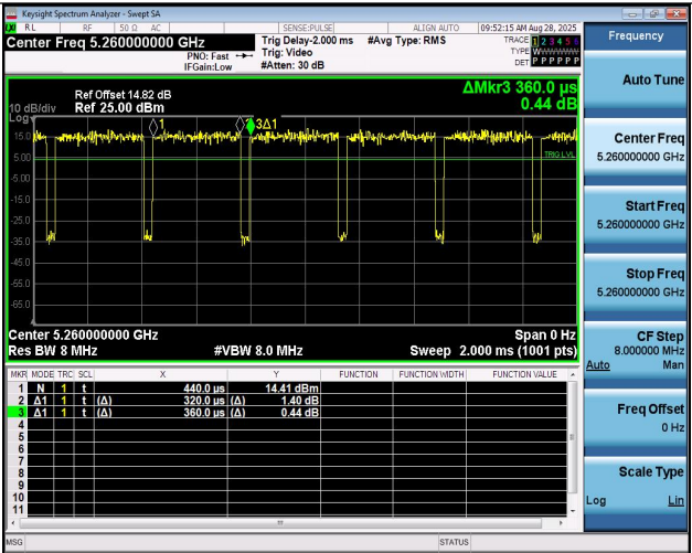
NTNV-11AX20MIMO-Ant2-5260
