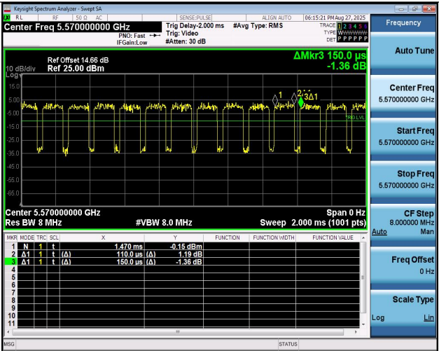
NTNV-11AC160MIMO-Ant1-5570
