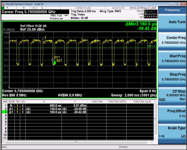
NTNV-11AC40MIMO-Ant2-5795
