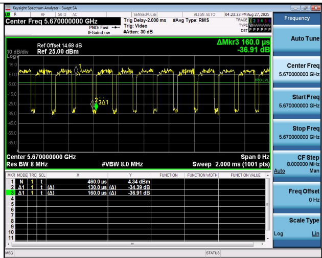
NTNV-11AC40MIMO-Ant1-5670
