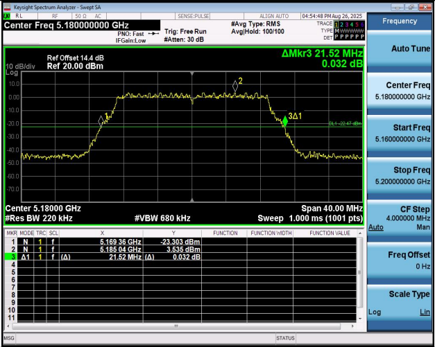
11N20MIMO-Ant2-5180
