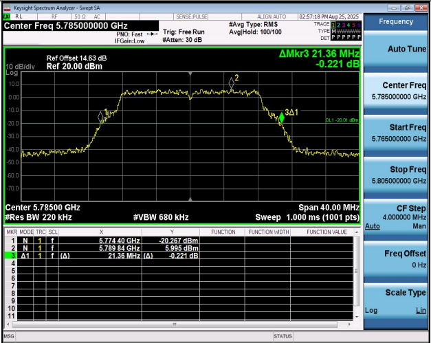
11A-Ant1-5785
