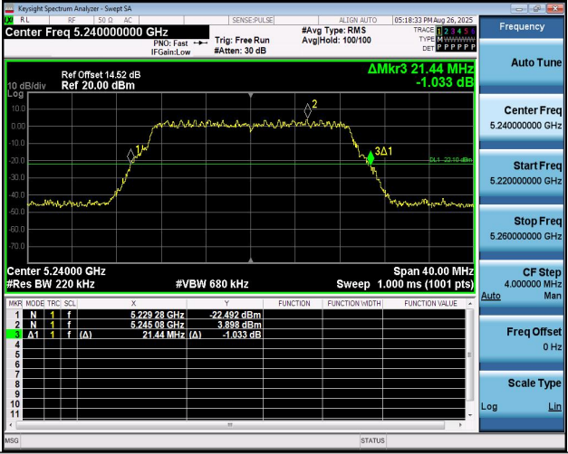
11N20MIMO-Ant2-5240
