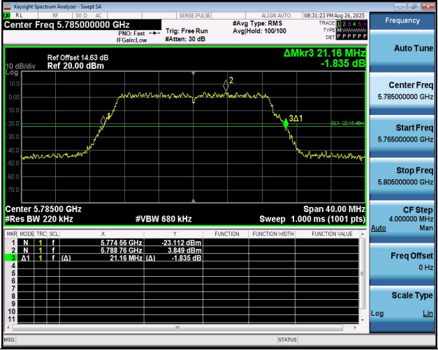
11N20MIMO-Ant1-5785
