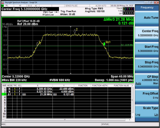
11N20MIMO-Ant2-5320
