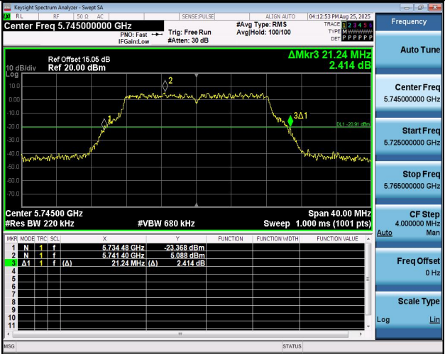
11A-Ant2-5745
