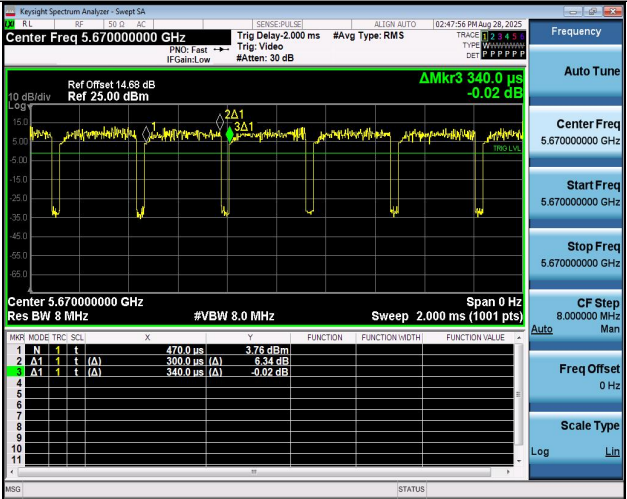
NTNV-11AX40MIMO-Ant1-5670
