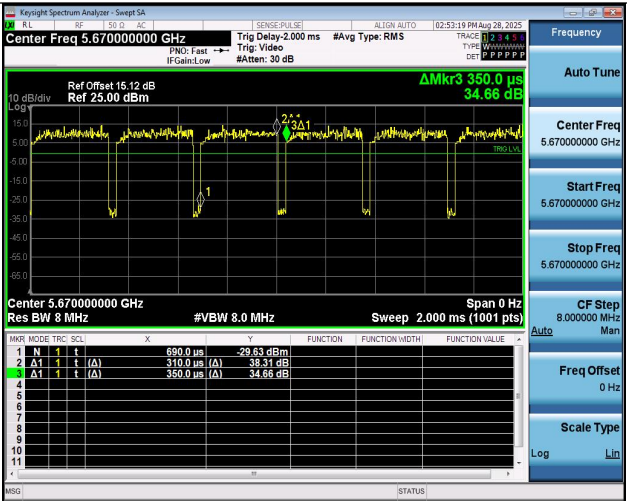
NTNV-11AX40MIMO-Ant2-5670
