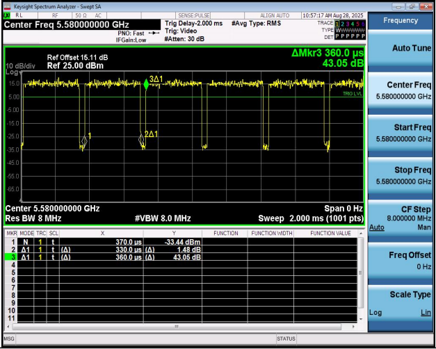
NTNV-11AX20MIMO-Ant2-5580
