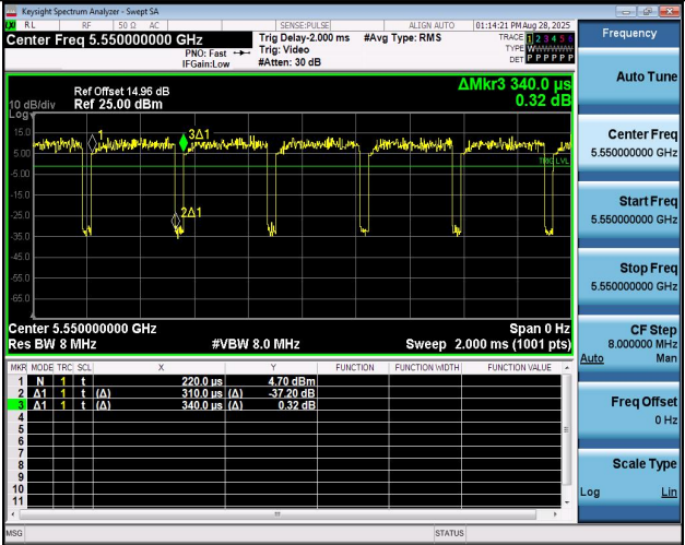
NTNV-11AX40MIMO-Ant2-5550
