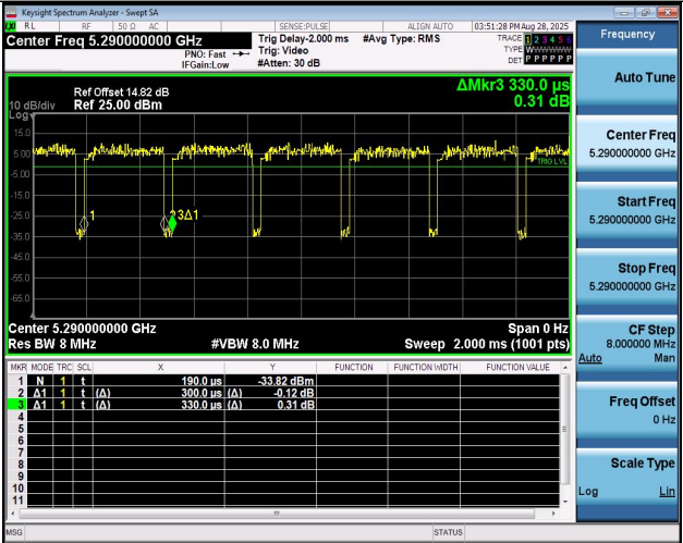
NTNV-11AX80MIMO-Ant2-5290
