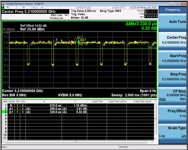
NTNV-11AX80MIMO-Ant2-5210
