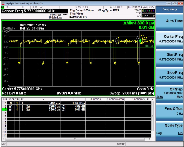
NTNV-11AX80MIMO-Ant2-5775
