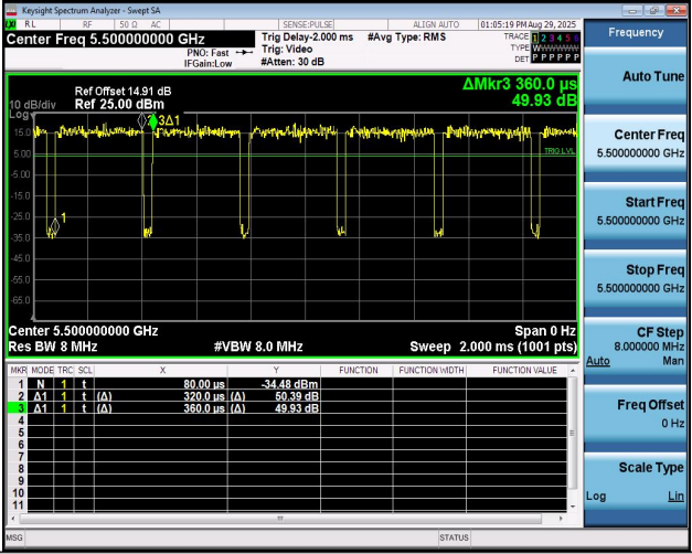
NTNV-11BE20MIMO-Ant2-5500
