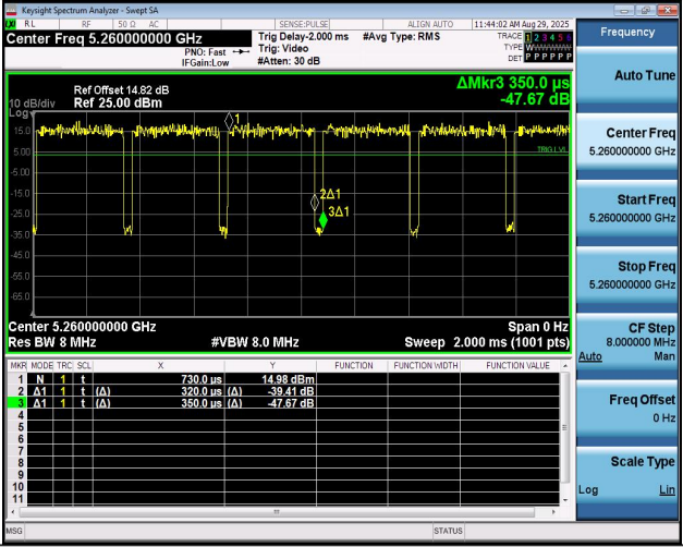
NTNV-11BE20MIMO-Ant2-5260
