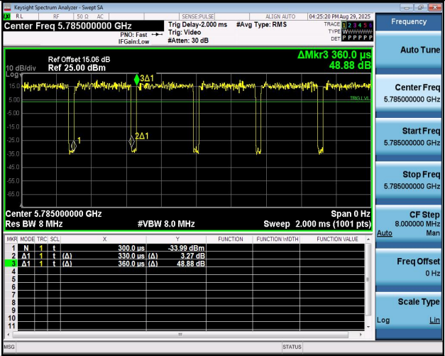
NTNV-11BE20MIMO-Ant2-5785
