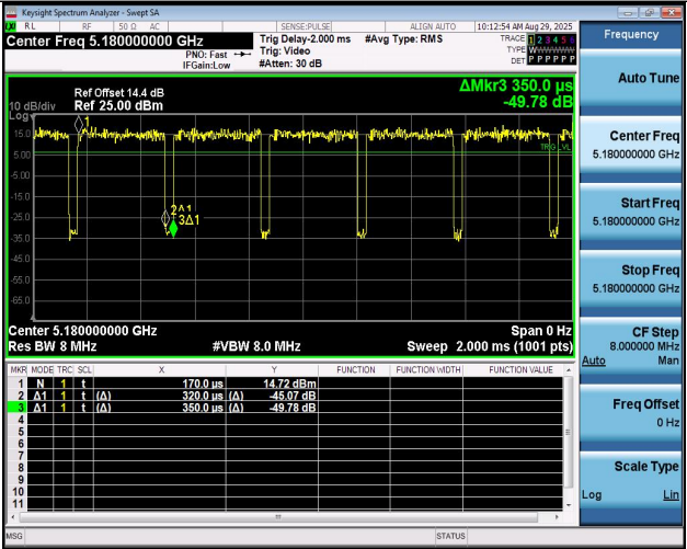
NTNV-11BE20MIMO-Ant2-5180
