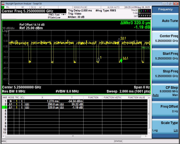
NTNV-11AX160MIMO-Ant1-5250
