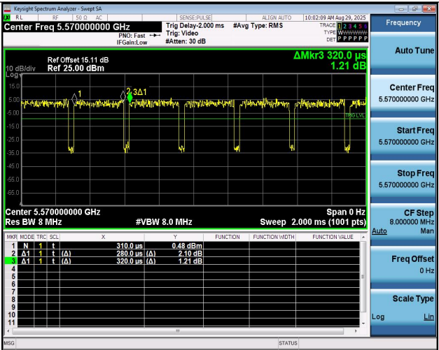
NTNV-11AX160MIMO-Ant2-5570
