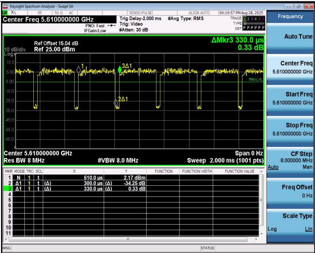
NTNV-11AX80MIMO-Ant2-5610
