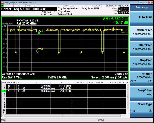
NTNV-11BE20MIMO-Ant1-5180
