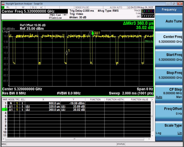
NTNV-11BE20MIMO-Ant2-5320
