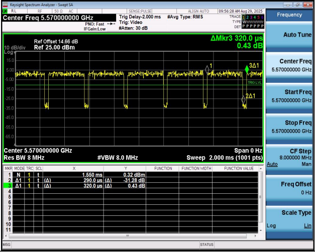
NTNV-11AX160MIMO-Ant1-5570
