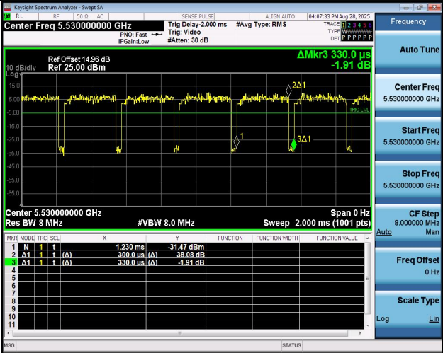
NTNV-11AX80MIMO-Ant2-5530
