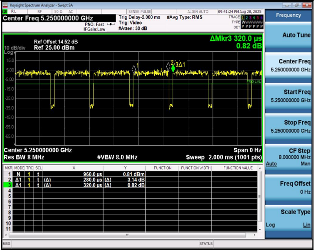
NTNV-11AX160MIMO-Ant2-5250
