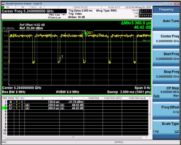
NTNV-11BE20MIMO-Ant2-5240
