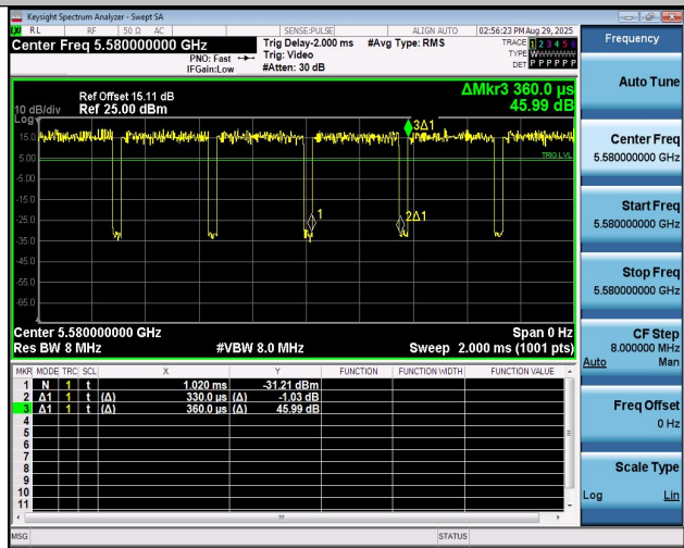
NTNV-11BE20MIMO-Ant2-5580
