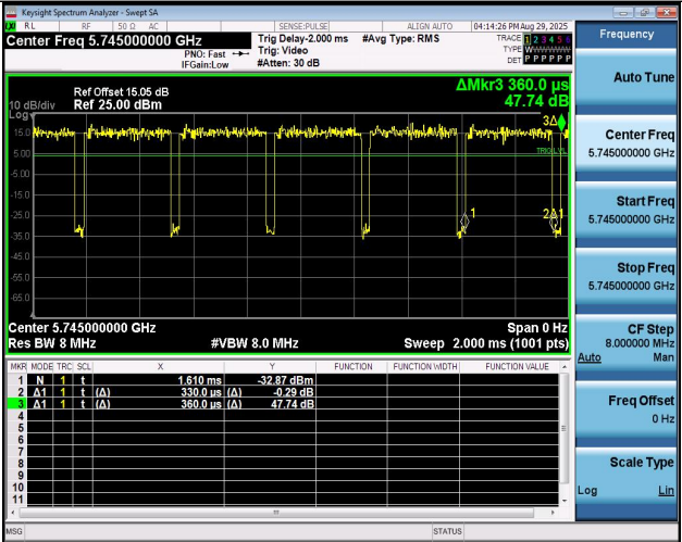
NTNV-11BE20MIMO-Ant2-5745
