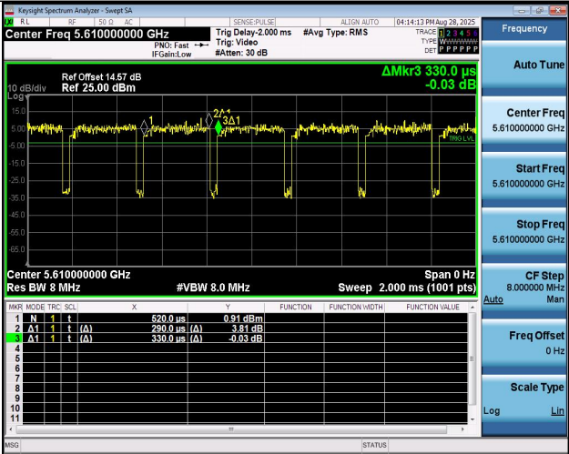
NTNV-11AX80MIMO-Ant1-5610
