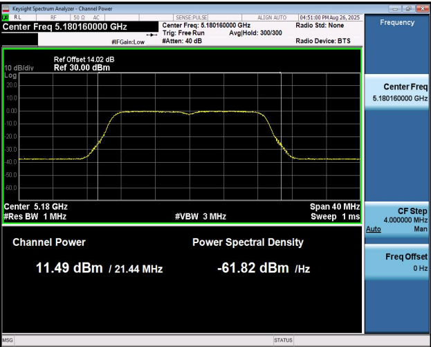
11N20MIMO-Ant1-5180-PASS
