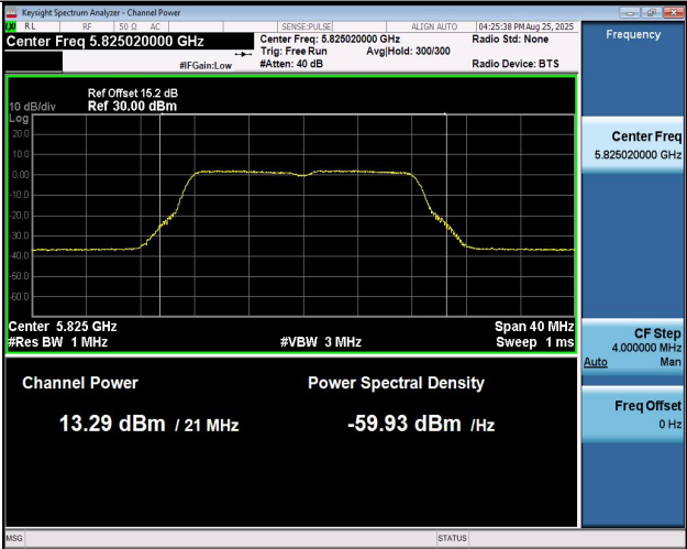
11A-Ant2-5825-PASS
