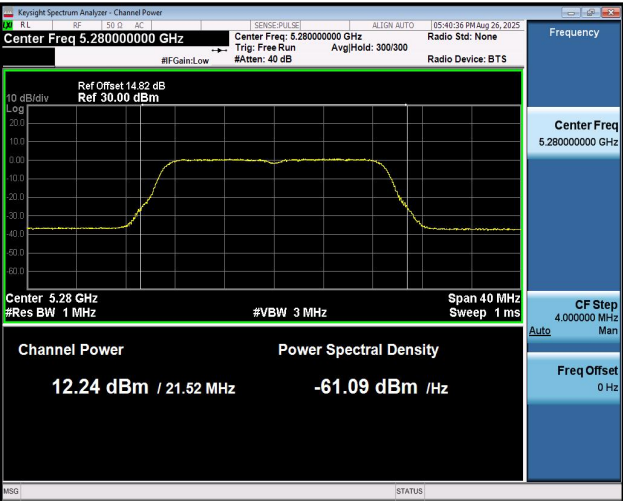
11N20MIMO-Ant2-5280-PASS
