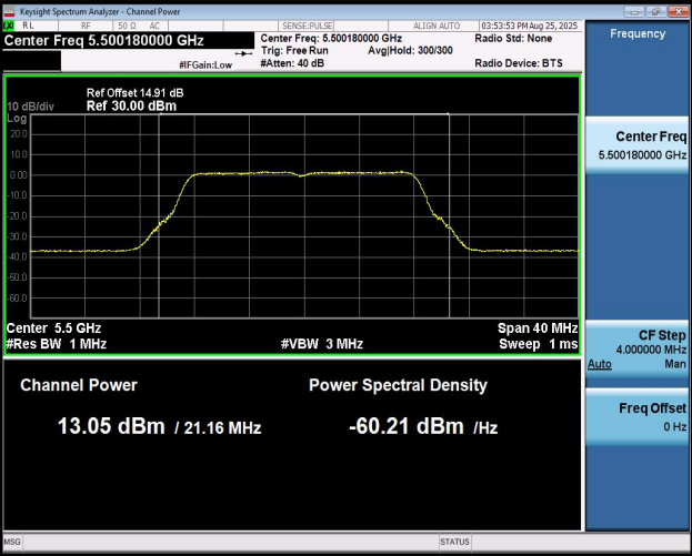
11A-Ant2-5500-PASS
