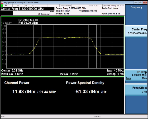
11N20MIMO-Ant1-5320-PASS
