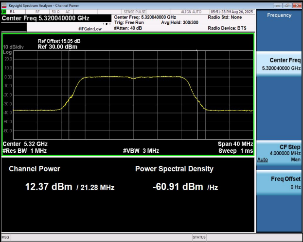
11N20MIMO-Ant2-5320-PASS
