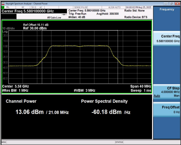
11A-Ant2-5580-PASS
