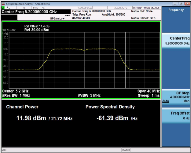
11N20MIMO-Ant2-5200-PASS
