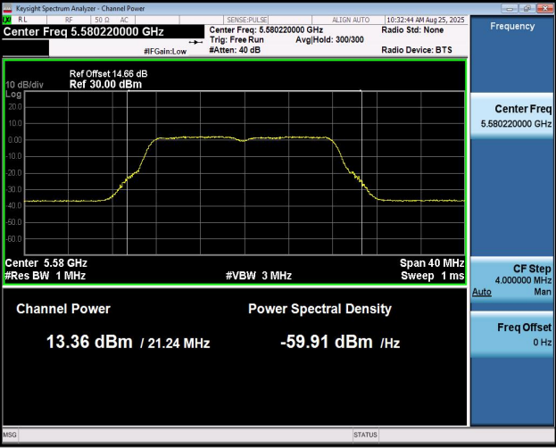
11A-Ant1-5580-PASS
