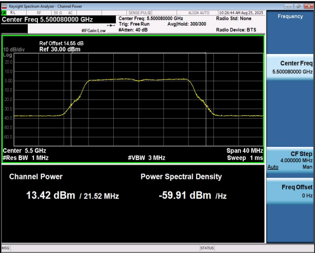
11A-Ant1-5500-PASS
