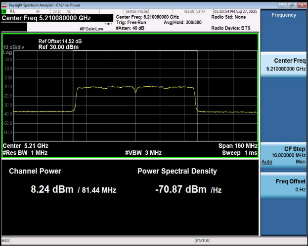
11AC80MIMO-Ant2-5210-PASS
