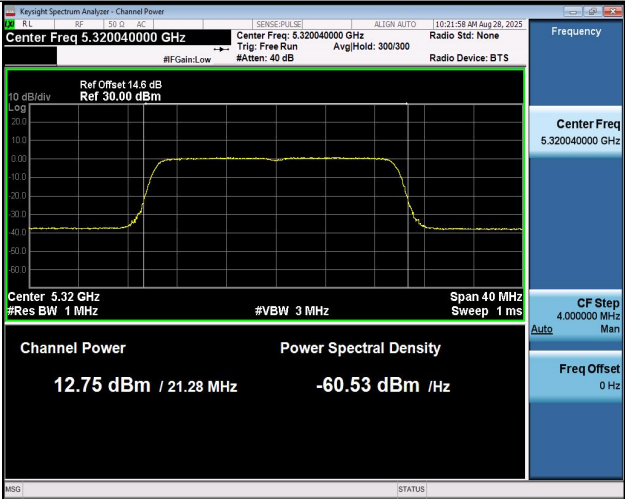
11AX20MIMO-Ant1-5320-PASS
