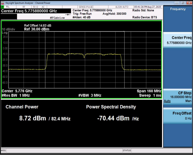
11AC80MIMO-Ant1-5775-PASS
