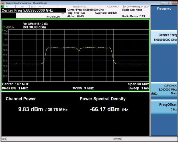
11AC40MIMO-Ant2-5670-PASS
