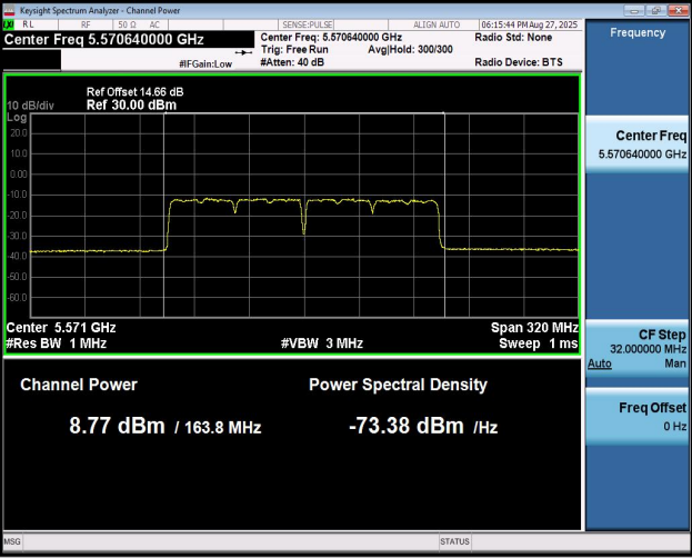
11AC160MIMO-Ant1-5570-PASS
