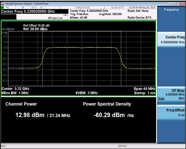
11AX20MIMO-Ant2-5320-PASS
