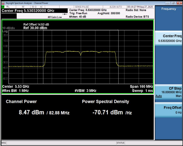
11AC80MIMO-Ant1-5530-PASS
