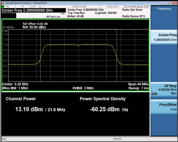
11AX20MIMO-Ant2-5280-PASS
