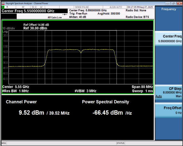
11AC40MIMO-Ant2-5550-PASS
