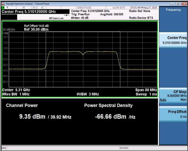
11AC40MIMO-Ant1-5310-PASS
