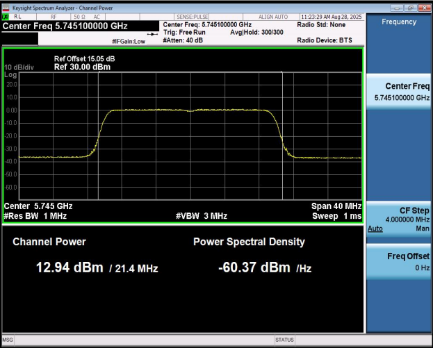
11AX20MIMO-Ant2-5745-PASS
