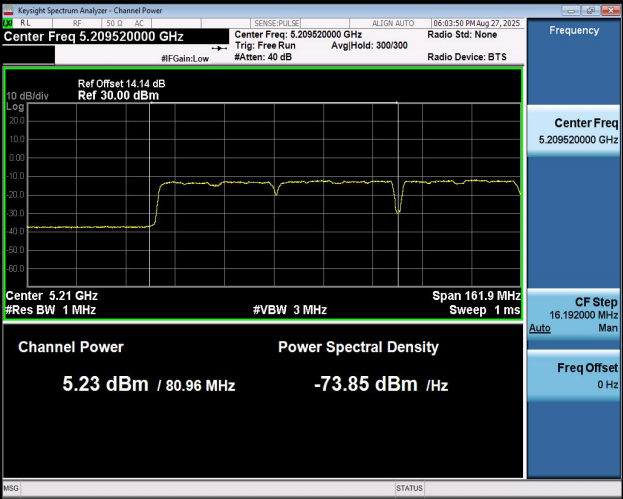
11AC160MIMO-Ant1-5250_UNII-1-PASS
