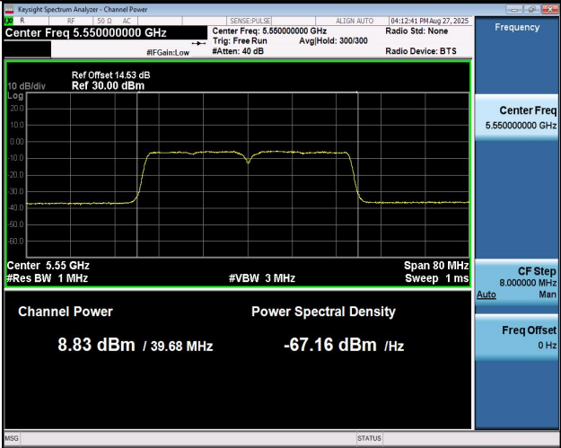
11AC40MIMO-Ant1-5550-PASS
