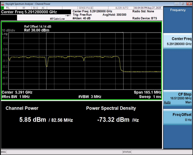
11AC160MIMO-Ant1-5250_UNII-2A-PASS
