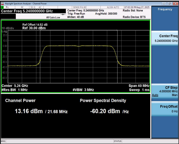
11AX20MIMO-Ant2-5240-PASS
