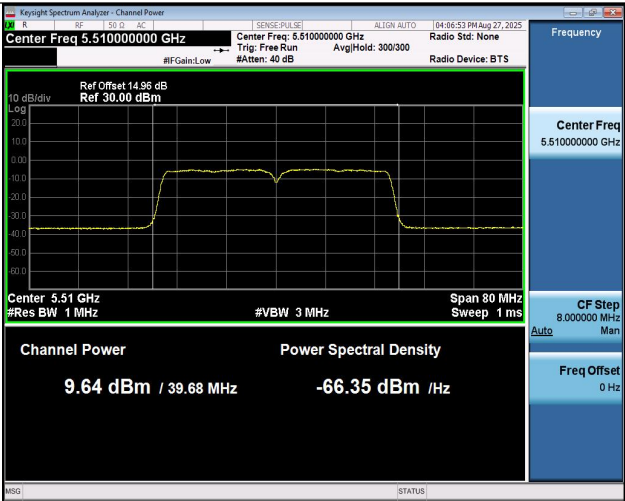
11AC40MIMO-Ant2-5510-PASS
