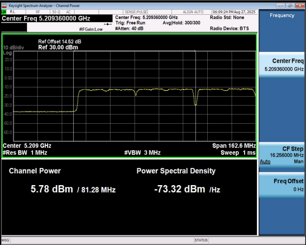
11AC160MIMO-Ant2-5250_UNII-1-PASS
