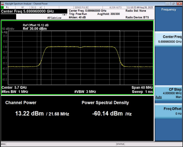
11AX20MIMO-Ant2-5700-PASS
