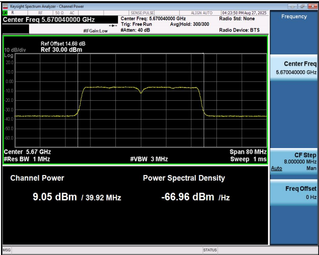
11AC40MIMO-Ant1-5670-PASS
