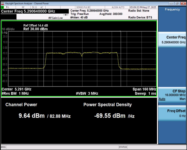
11AC80MIMO-Ant1-5290-PASS
