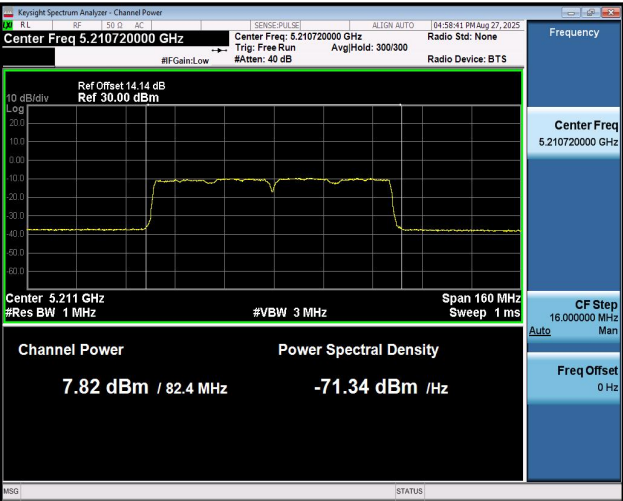
11AC80MIMO-Ant1-5210-PASS
