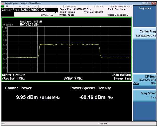
11AC80MIMO-Ant2-5290-PASS
