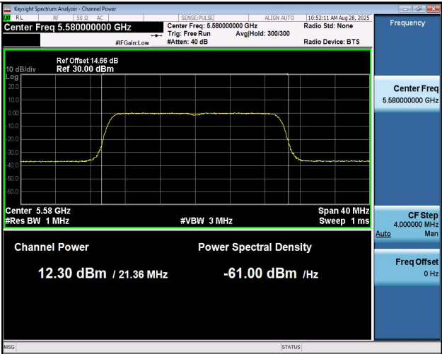
11AX20MIMO-Ant1-5580-PASS
