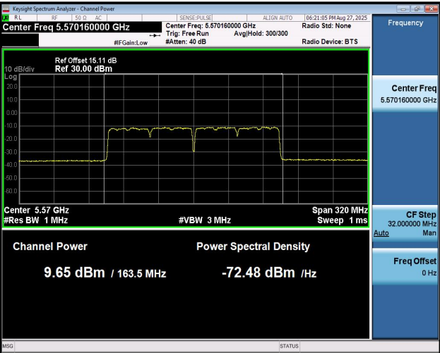
11AC160MIMO-Ant2-5570-PASS
