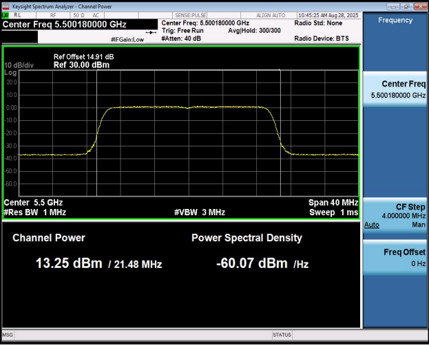
11AX20MIMO-Ant2-5500-PASS
