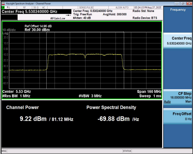
11AC80MIMO-Ant2-5530-PASS
