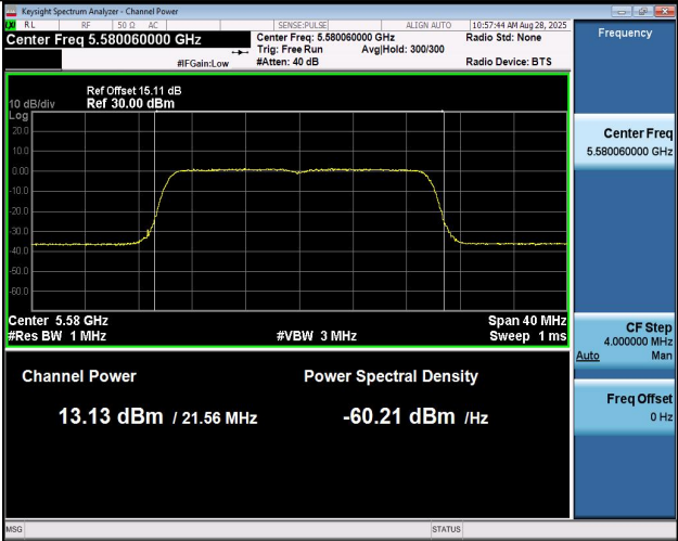
11AX20MIMO-Ant2-5580-PASS
