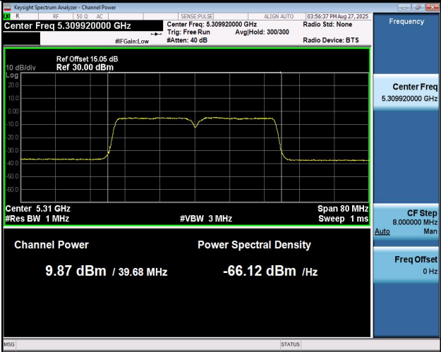
11AC40MIMO-Ant2-5310-PASS
