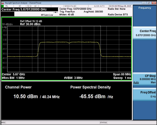
11AX40MIMO-Ant2-5670-PASS
