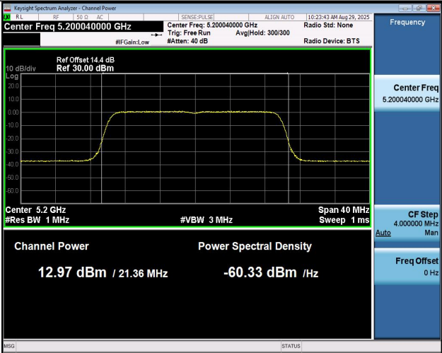
11BE20MIMO-Ant2-5200-PASS
