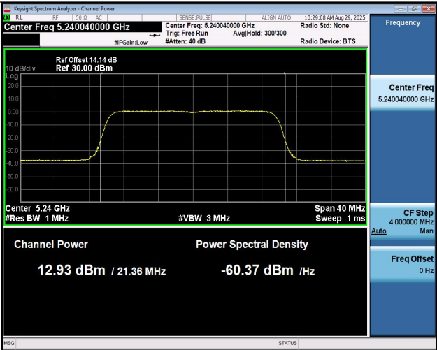
11BE20MIMO-Ant1-5240-PASS
