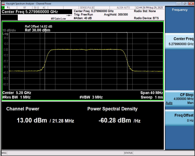
11BE20MIMO-Ant2-5280-PASS
