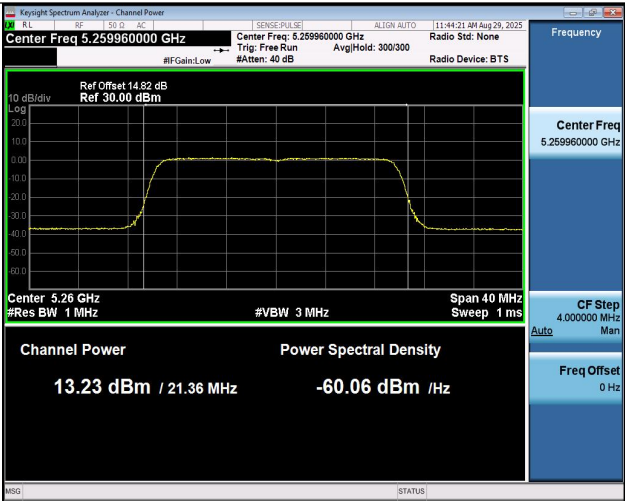
11BE20MIMO-Ant2-5260-PASS
