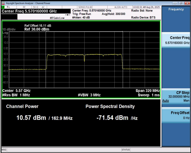
11AX160MIMO-Ant2-5570-PASS
