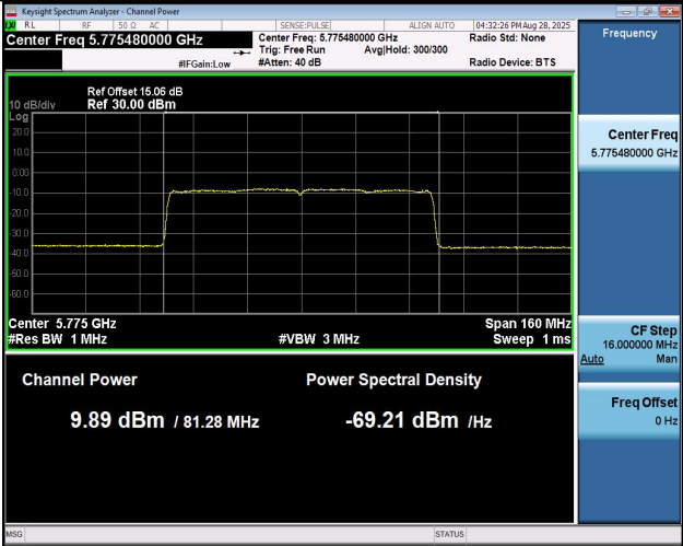
11AX80MIMO-Ant2-5775-PASS
