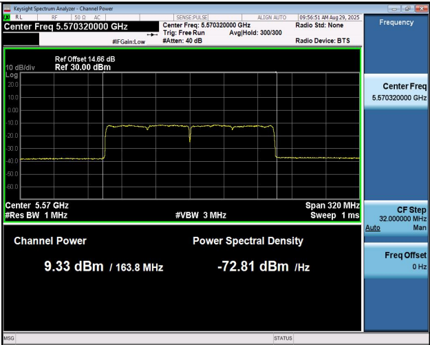
11AX160MIMO-Ant1-5570-PASS
