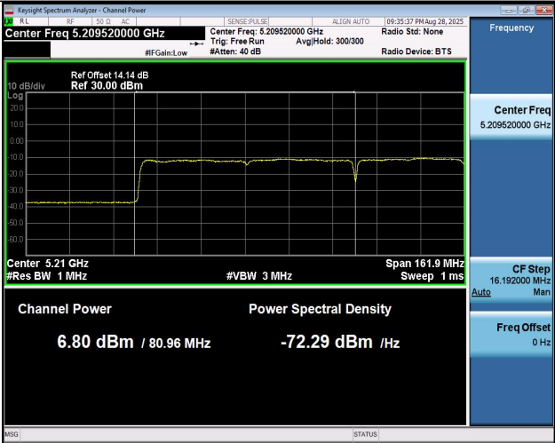
11AX160MIMO-Ant1-5250_UNII-1-PASS
