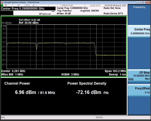
11AX160MIMO-Ant2-5250_UNII-2A-PASS
