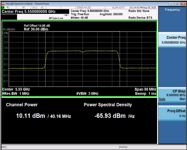
11AX40MIMO-Ant2-5550-PASS
