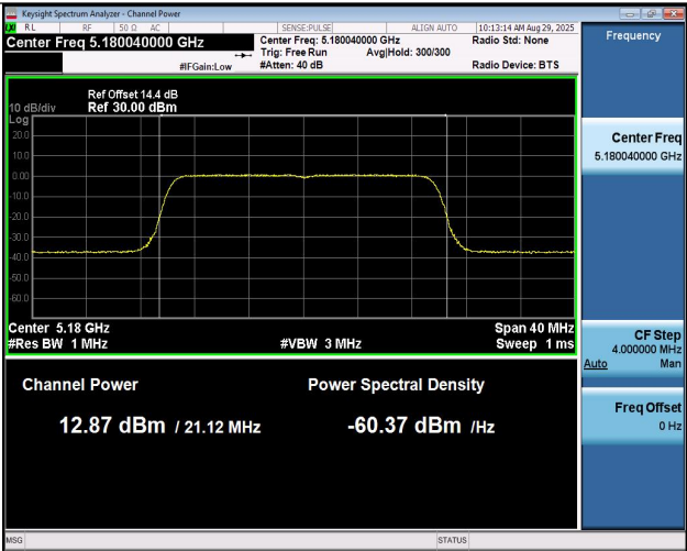
11BE20MIMO-Ant2-5180-PASS
