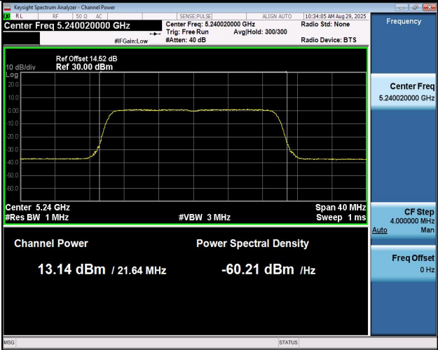
11BE20MIMO-Ant2-5240-PASS
