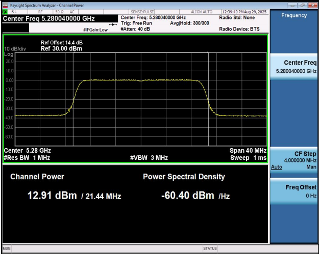
11BE20MIMO-Ant1-5280-PASS
