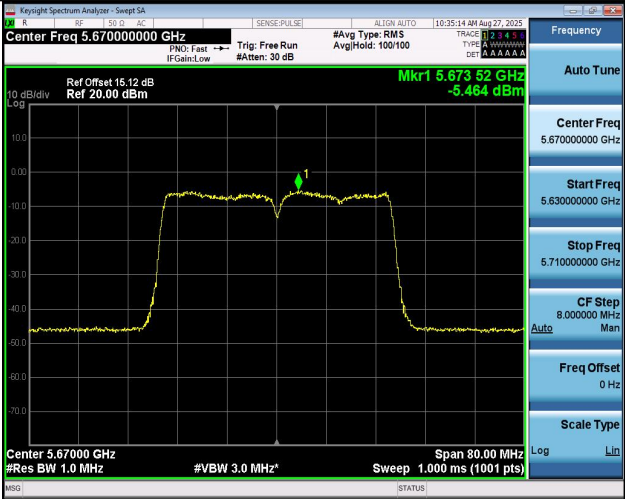
11N40MIMO-Ant2-5670-PASS
