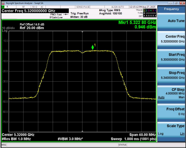
11AC20MIMO-Ant1-5320-PASS
