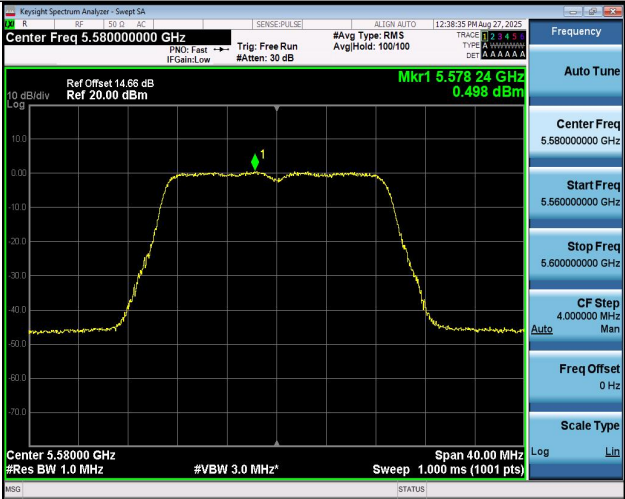
11AC20MIMO-Ant1-5580-PASS
