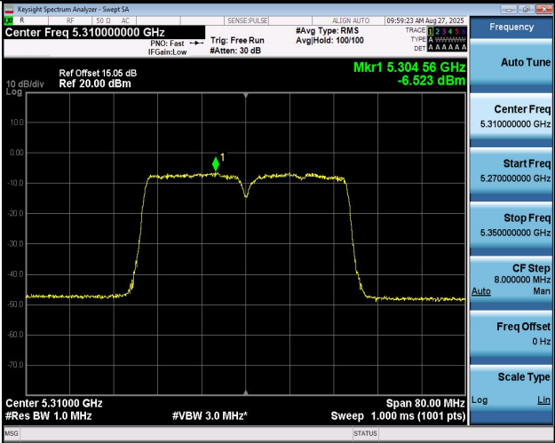
11N40MIMO-Ant2-5310-PASS
