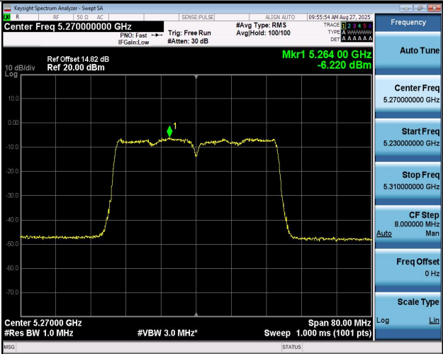
11N40MIMO-Ant2-5270-PASS
