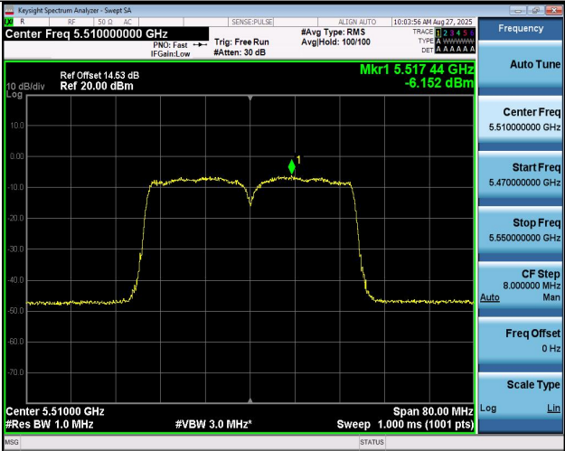
11N40MIMO-Ant1-5510-PASS
