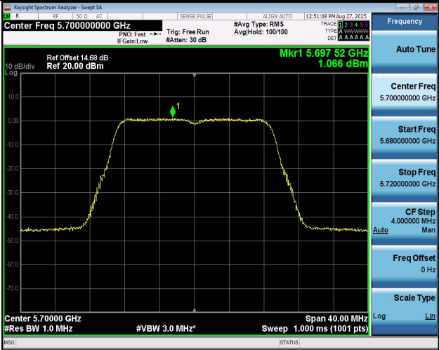
11AC20MIMO-Ant1-5700-PASS
