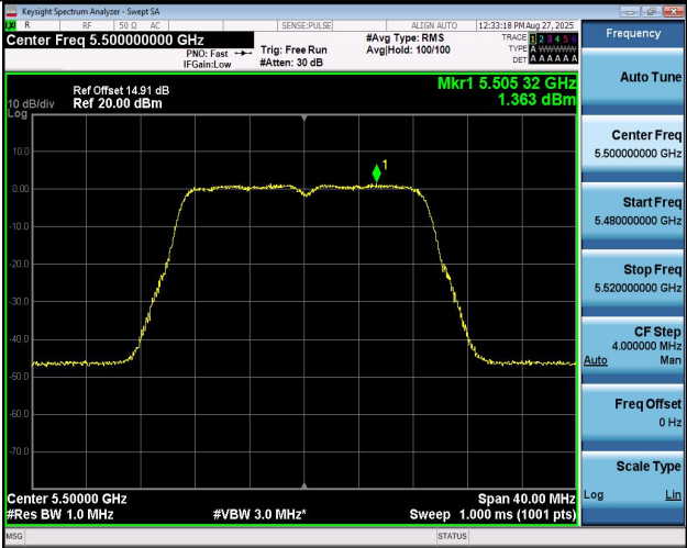
11AC20MIMO-Ant2-5500-PASS
