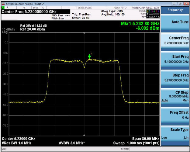
11N40MIMO-Ant2-5230-PASS
