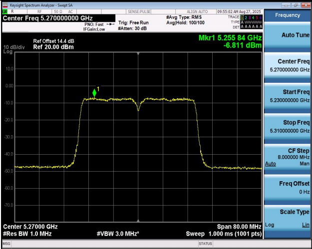
11N40MIMO-Ant1-5270-PASS
