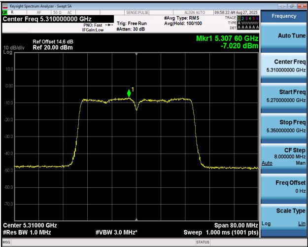
11N40MIMO-Ant1-5310-PASS
