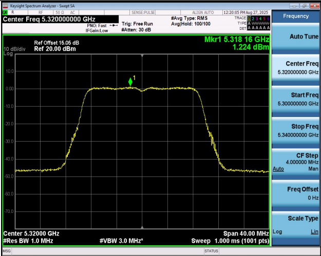
11AC20MIMO-Ant2-5320-PASS
