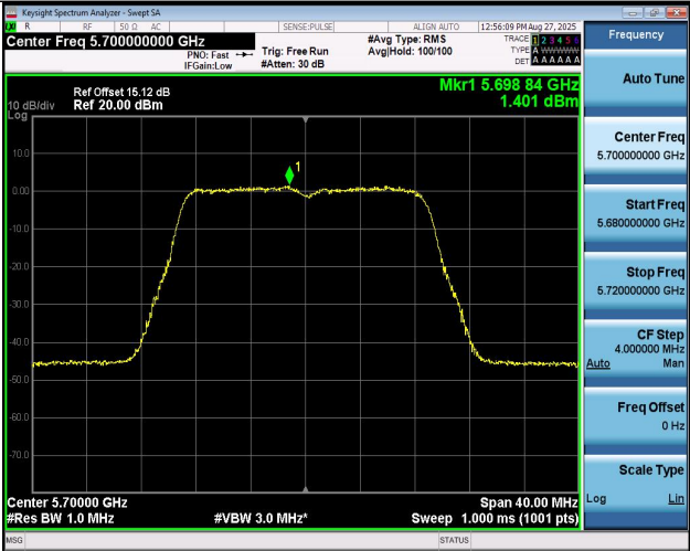
11AC20MIMO-Ant2-5700-PASS
