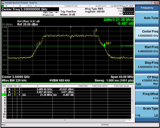
11AC20MIMO-Ant2-5500
