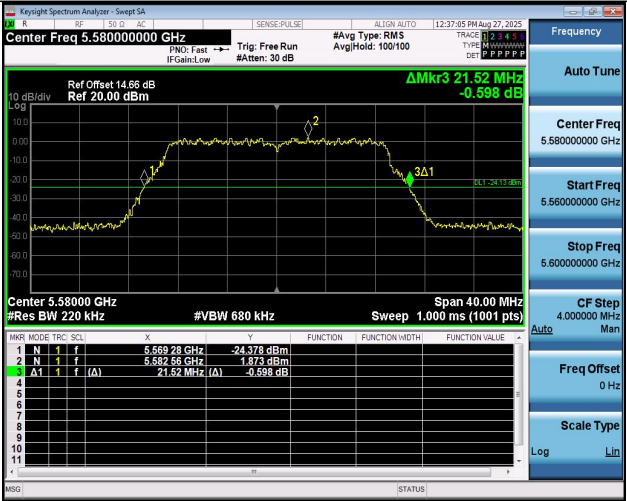
11AC20MIMO-Ant1-5580
