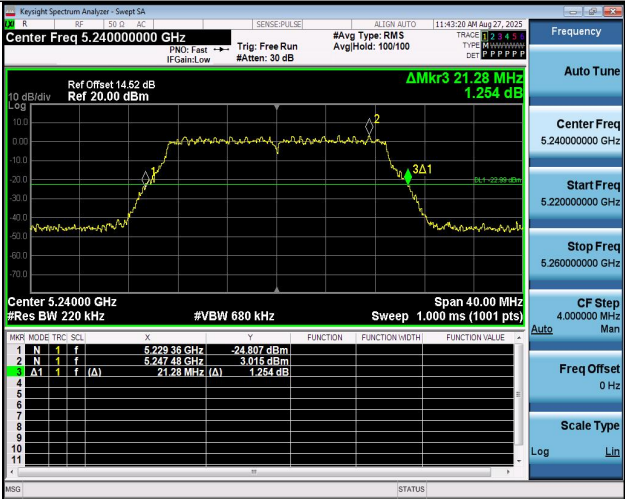
11AC20MIMO-Ant2-5240
