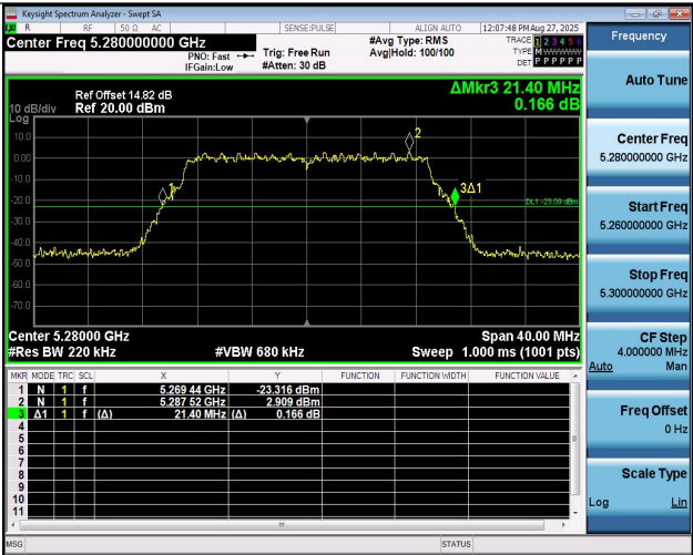
11AC20MIMO-Ant2-5280
