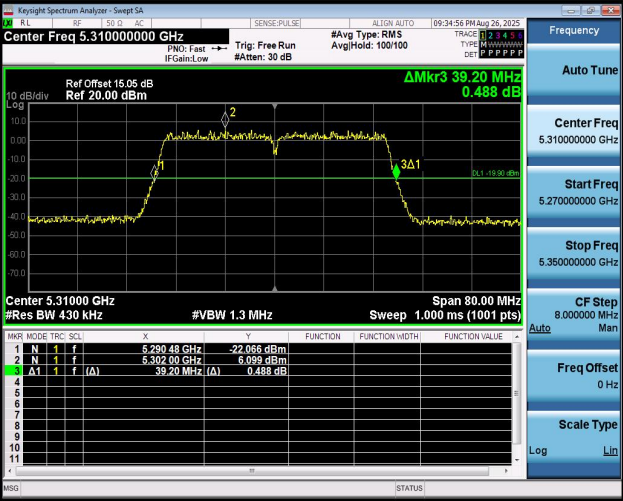
11N40MIMO-Ant2-5310
