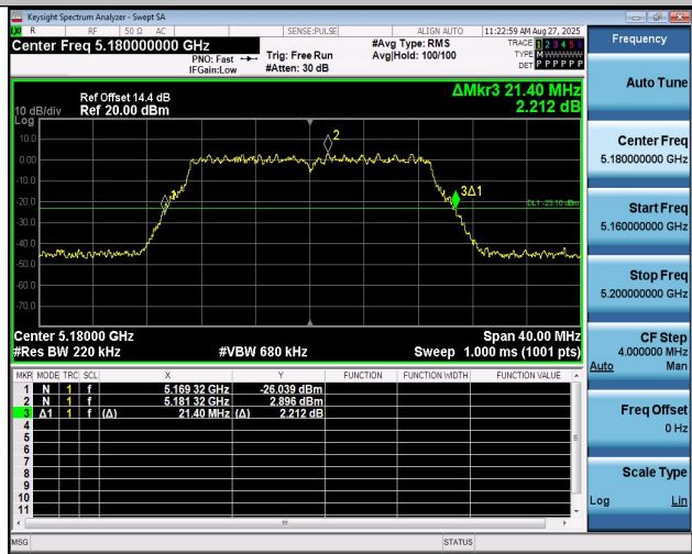
11AC20MIMO-Ant2-5180
