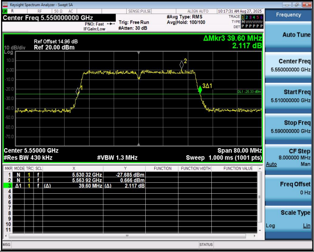
11N40MIMO-Ant2-5550
