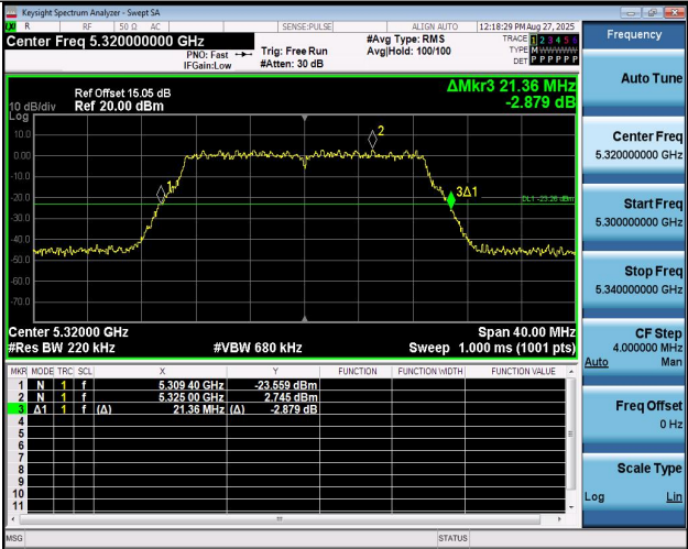
11AC20MIMO-Ant2-5320
