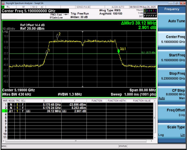
11N40MIMO-Ant2-5190
