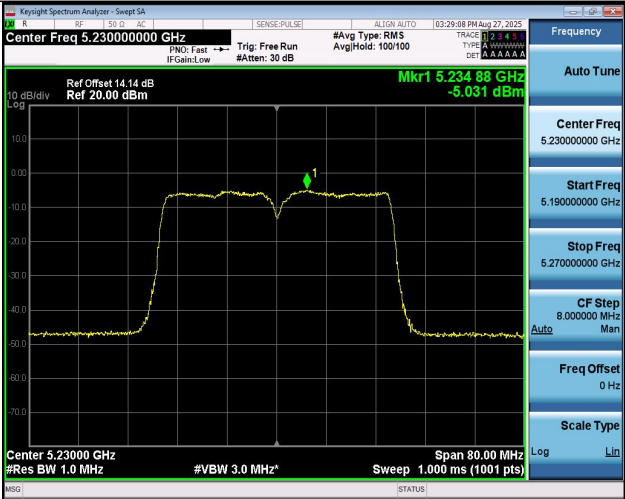
11AC40MIMO-Ant1-5230-PASS
