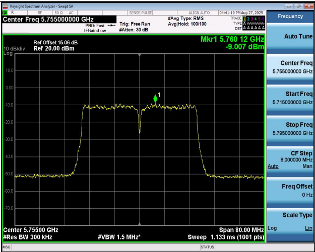
11AC40MIMO-Ant2-5755-PASS
