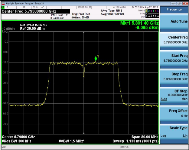
11AC40MIMO-Ant2-5795-PASS
