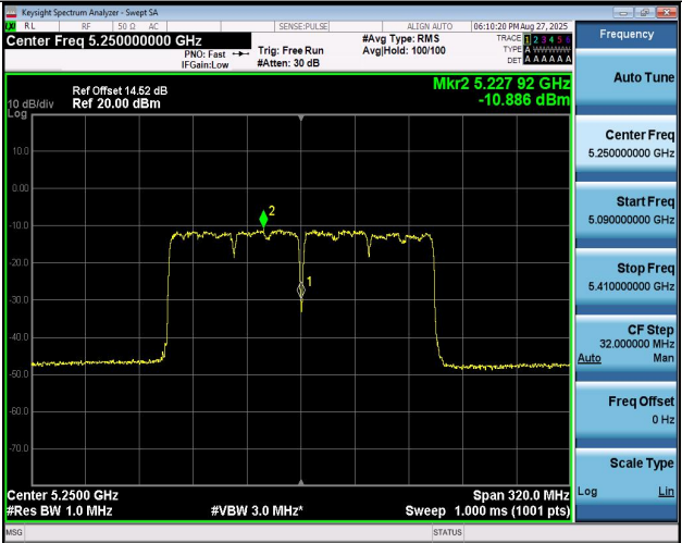
11AC160MIMO-Ant2-5250_UNII-1-PASS
