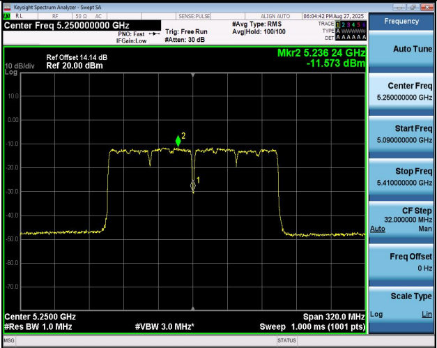
11AC160MIMO-Ant1-5250_UNII-1-PASS
