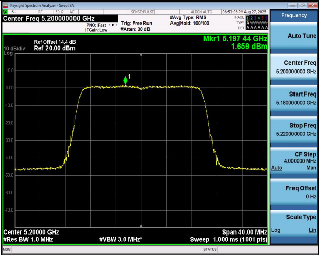
11AX20MIMO-Ant2-5200-PASS
