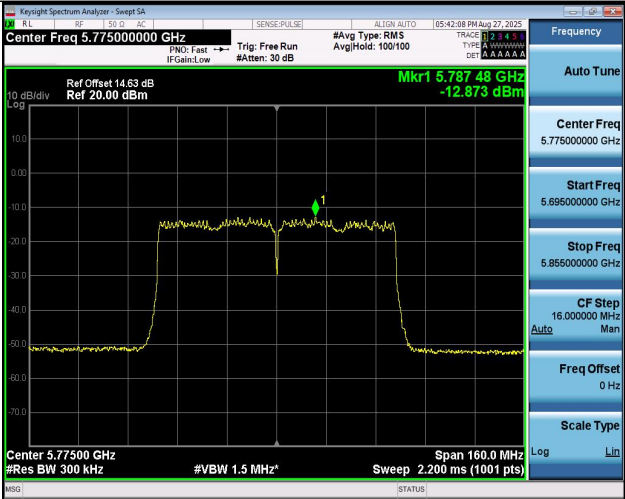
11AC80MIMO-Ant1-5775-PASS
