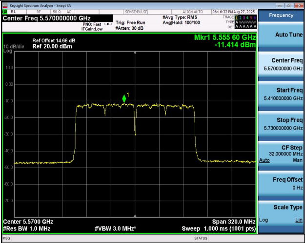
11AC160MIMO-Ant1-5570-PASS
