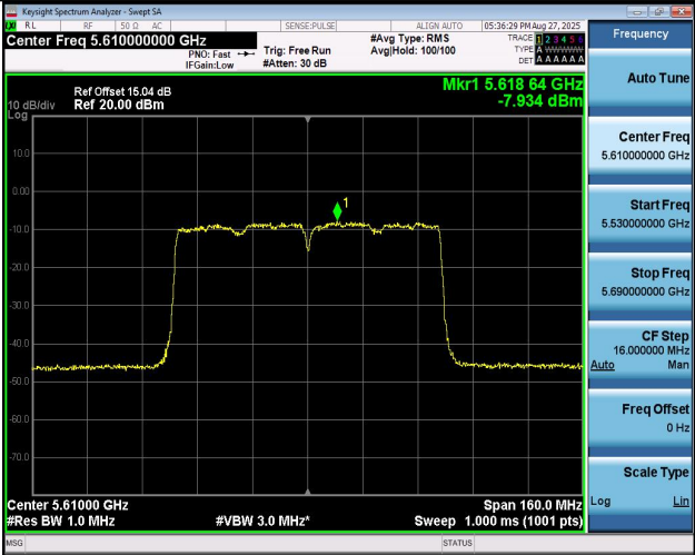
11AC80MIMO-Ant2-5610-PASS
