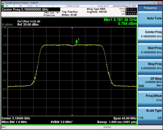
11AX20MIMO-Ant1-5180-PASS
