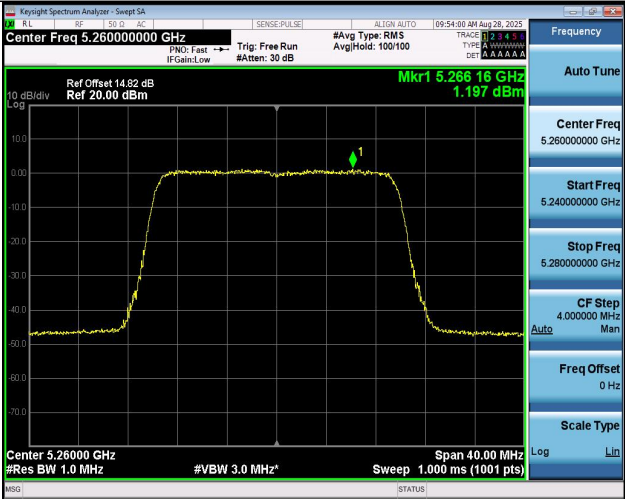
11AX20MIMO-Ant2-5260-PASS
