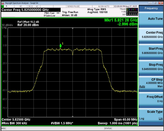
11AC20MIMO-Ant2-5825-PASS
