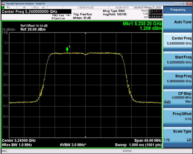
11AX20MIMO-Ant1-5240-PASS
