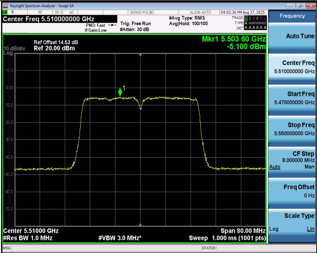
11AC40MIMO-Ant1-5510-PASS
