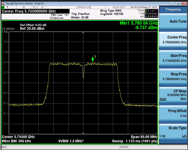
11AC40MIMO-Ant1-5755-PASS
