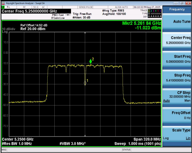
11AC160MIMO-Ant2-5250_UNII-2A-PASS
