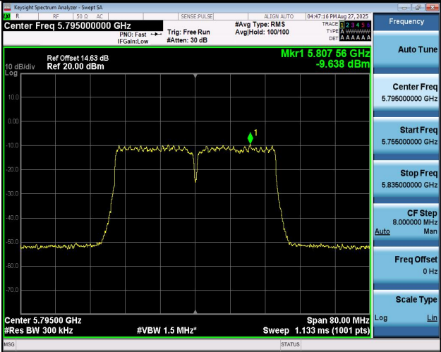
11AC40MIMO-Ant1-5795-PASS
