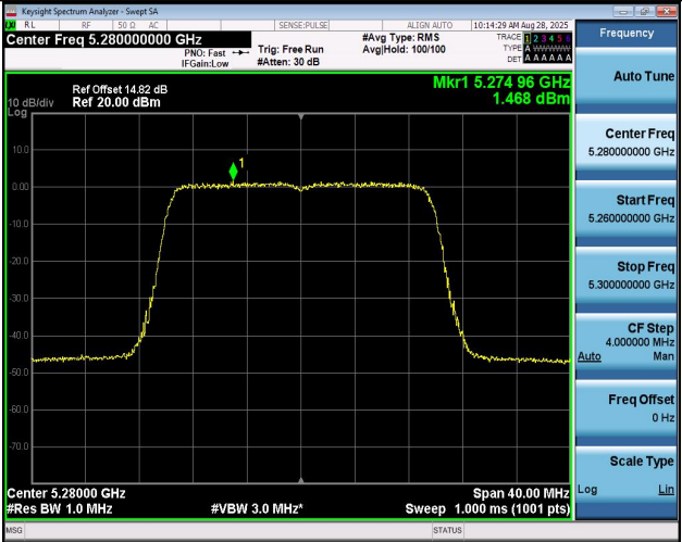
11AX20MIMO-Ant2-5280-PASS
