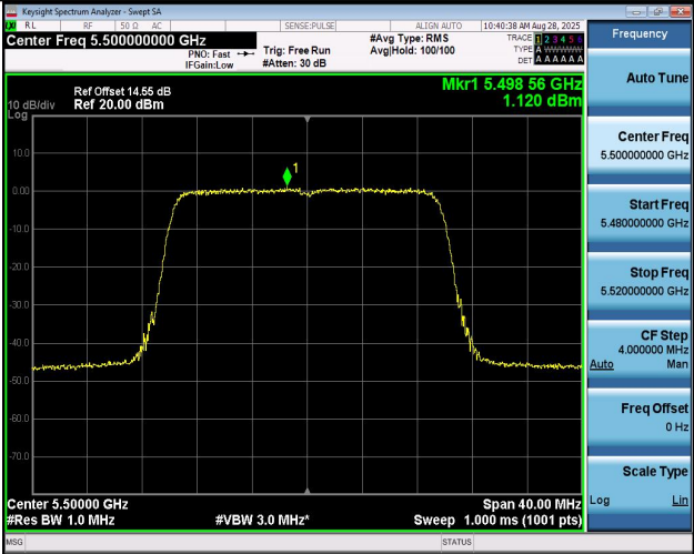
11AX20MIMO-Ant2-5500-PASS
