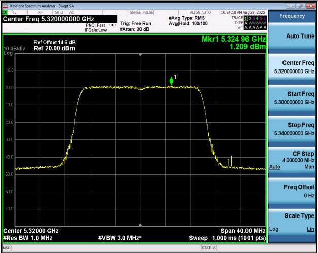
11AX20MIMO-Ant1-5320-PASS
