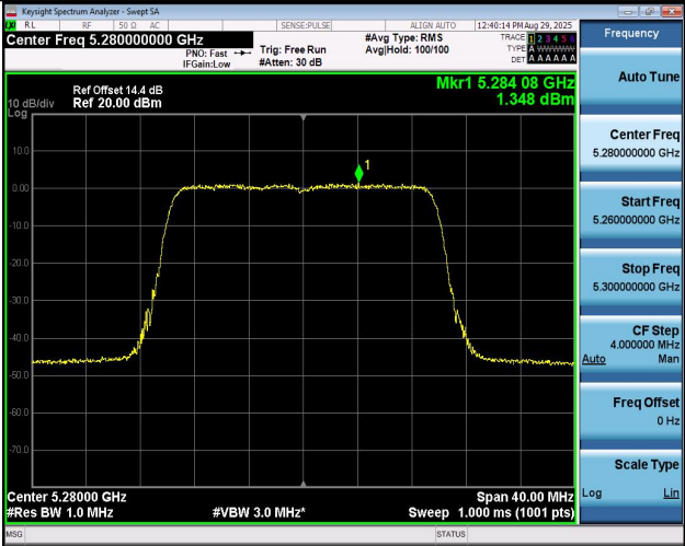
11B20MIMO-Ant1-5280-PASS
