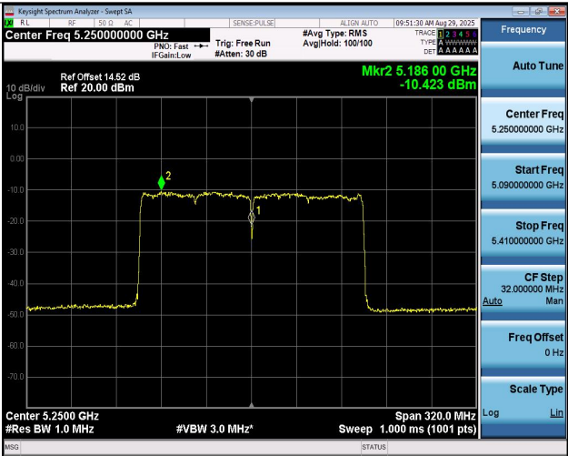
11AX160MIMO-Ant2-5250_UNII-1-PASS
