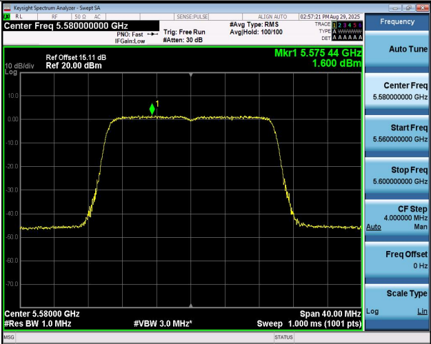
11B20MIMO-Ant2-5580-PASS
