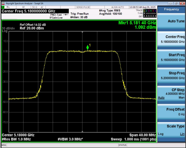
11BE20MIMO-Ant1-5180-PASS
