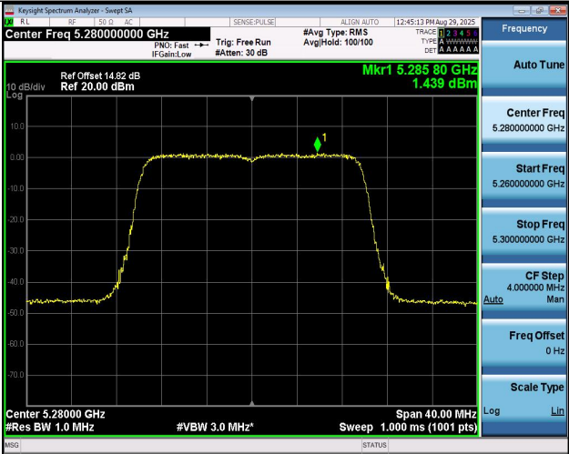
11B20MIMO-Ant2-5280-PASS
