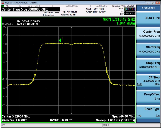
11B20MIMO-Ant2-5320-PASS
