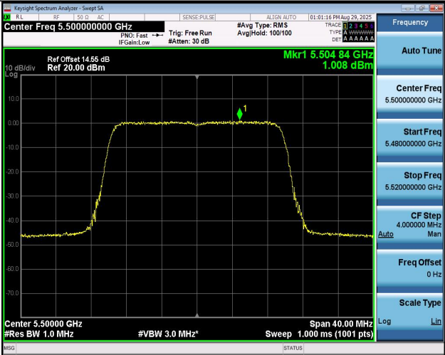
11B20MIMO-Ant1-5500-PASS
