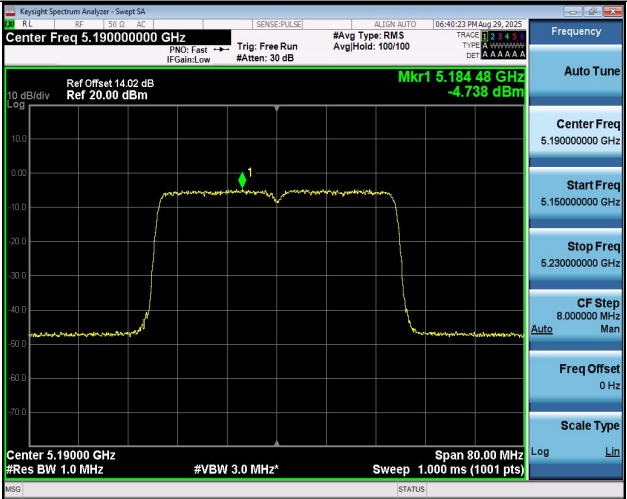
11BE40MIMO-Ant1-5190-PASS
