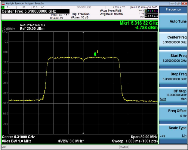
11BE40MIMO-Ant1-5310-PASS
