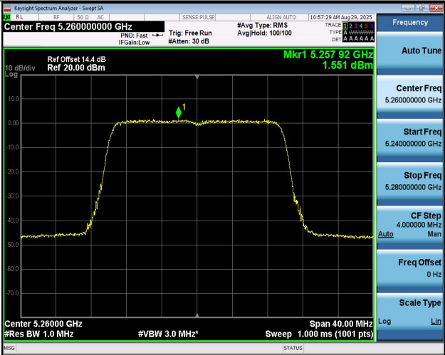
11BE20MIMO-Ant1-5260-PASS
