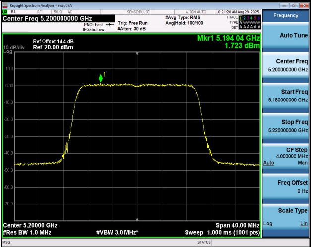
11B20MIMO-Ant2-5200-PASS
