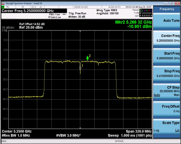
11AX160MIMO-Ant2-5250_UNII-2A-PASS
