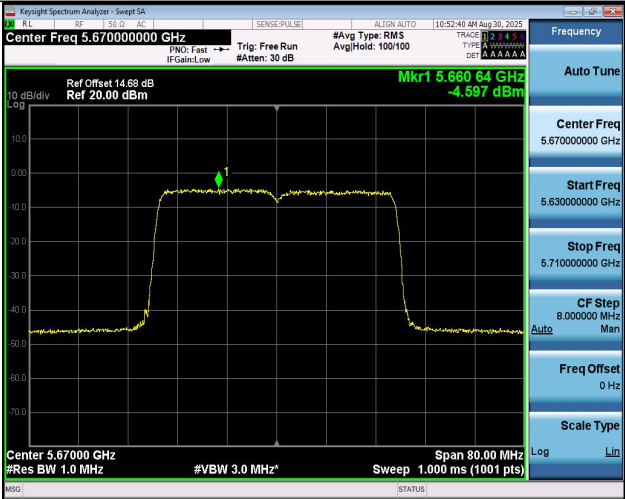
11BE40MIMO-Ant1-5670-PASS
