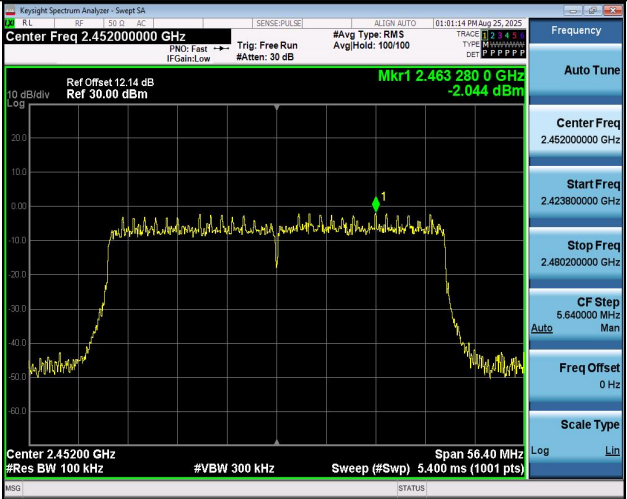
11BE40MIMO-Ant1-2452-PASS
