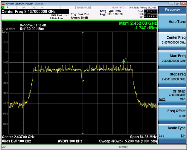
11N40MIMO-Ant2-2437-PASS
