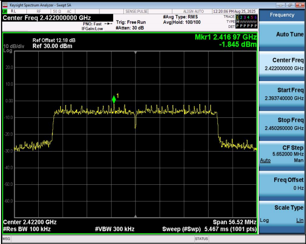
11BE40MIMO-Ant2-2422-PASS
