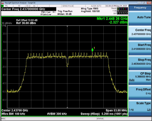
11N40MIMO-Ant1-2437-PASS
