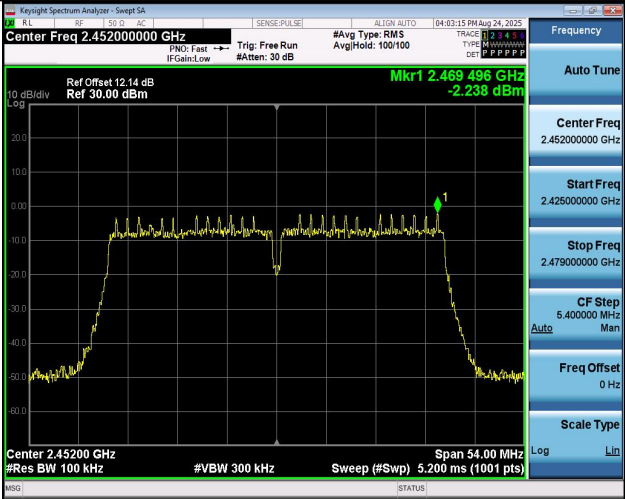
11N40MIMO-Ant1-2452-PASS
