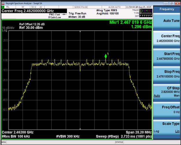
11B20MIMO-Ant2-2462-PASS
