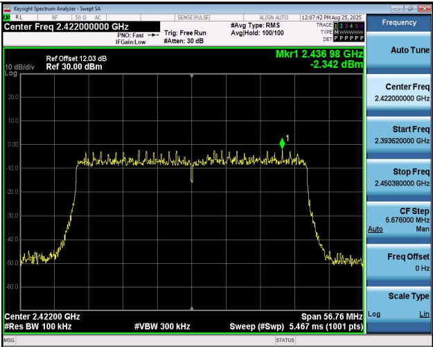
11BE40MIMO-Ant1-2422-PASS
