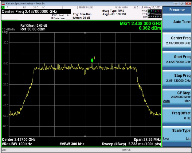
11B20MIMO-Ant1-2437-PASS
