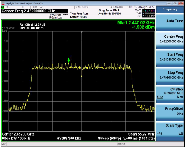
11BE40MIMO-Ant2-2452-PASS
