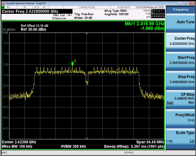
11N40MIMO-Ant2-2422-PASS
