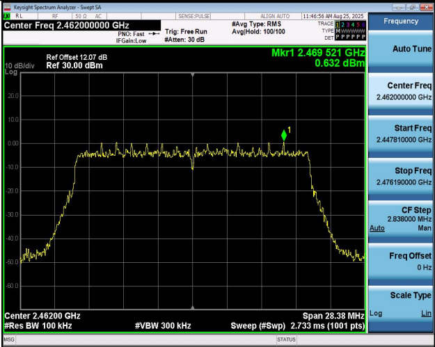
11B20MIMO-Ant1-2462-PASS
