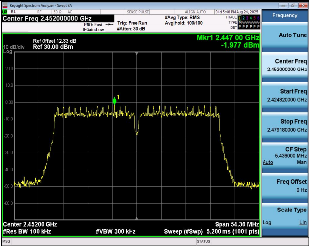
11N40MIMO-Ant2-2452-PASS
