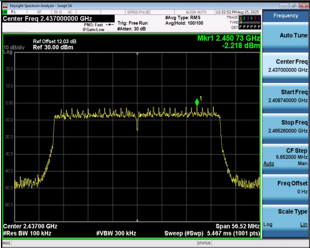
11BE40MIMO-Ant1-2437-PASS
