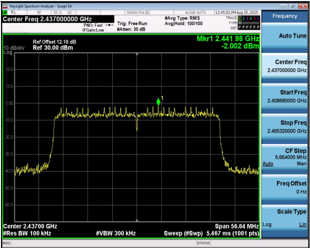
11BE40MIMO-Ant2-2437-PASS
