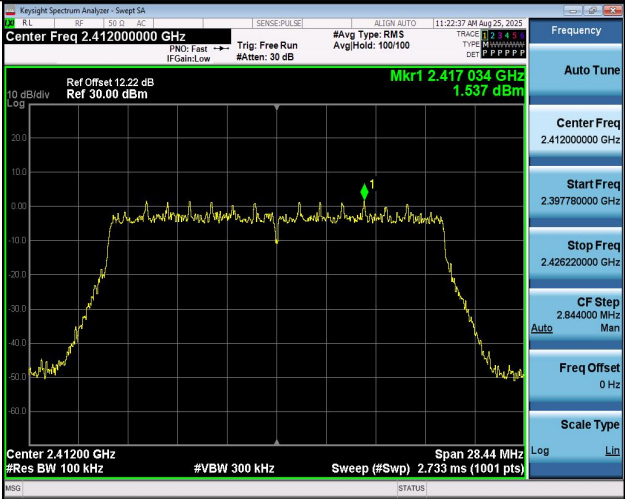
11B20MIMO-Ant2-2412-PASS
