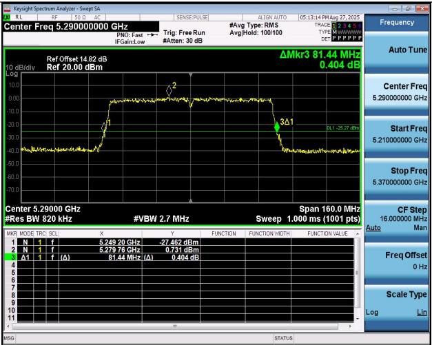
11AC80MIMO-Ant2-5290
