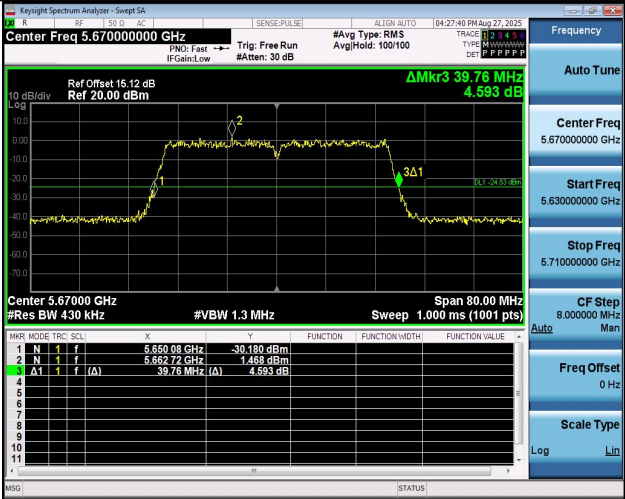
11AC40MIMO-Ant2-5670
