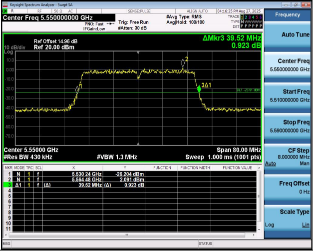
11AC40MIMO-Ant2-5550
