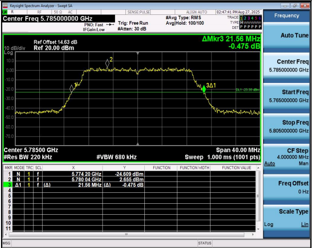
11AC20MIMO-Ant1-5785
