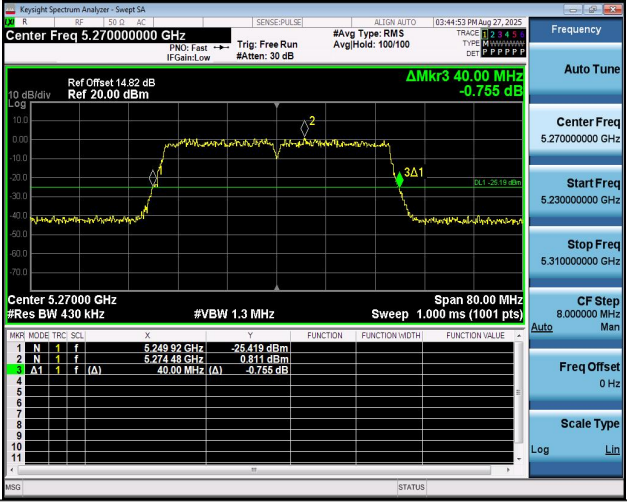
11AC40MIMO-Ant2-5270
