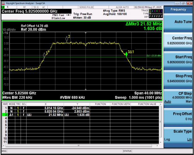
11AC20MIMO-Ant1-5825
