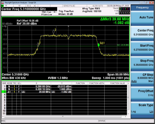
11AC40MIMO-Ant2-5310
