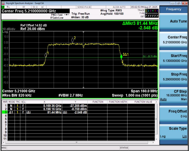
11AC80MIMO-Ant2-5210
