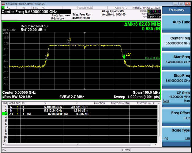
11AC80MIMO-Ant1-5530
