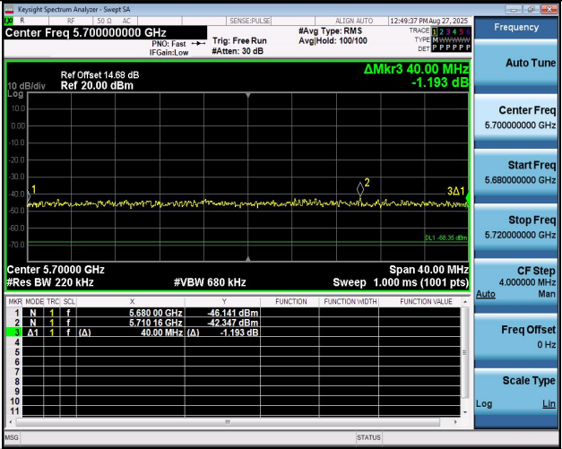
11AC20MIMO-Ant1-5700
