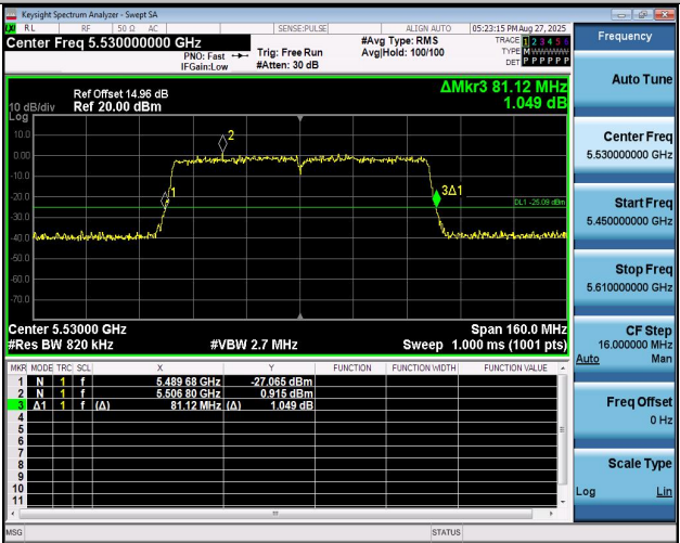
11AC80MIMO-Ant2-5530
