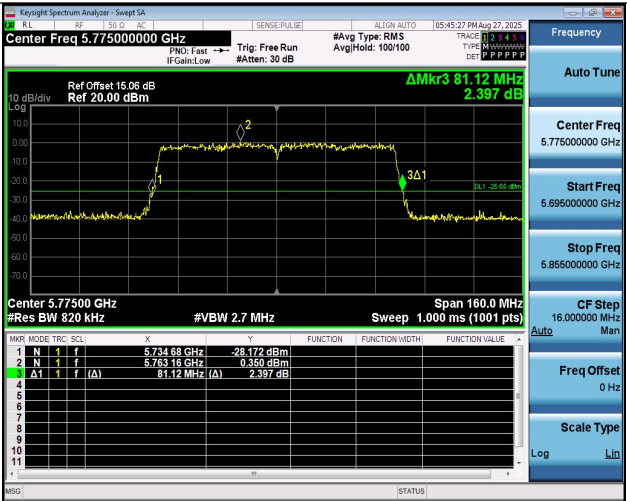
11AC80MIMO-Ant2-5775
