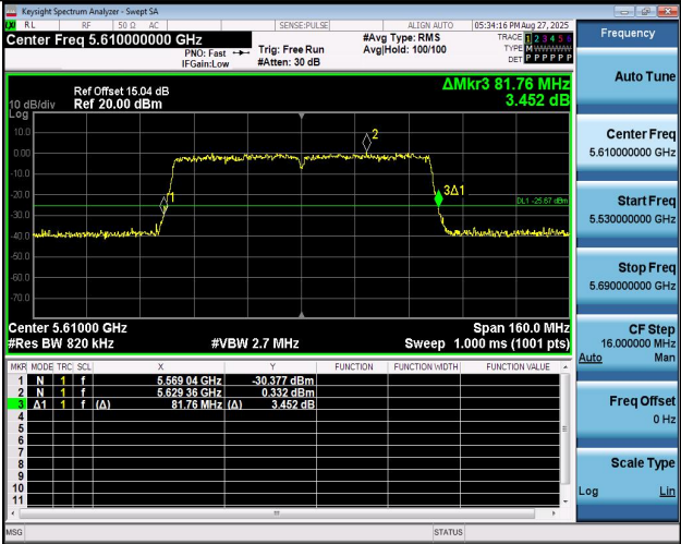
11AC80MIMO-Ant2-5610
