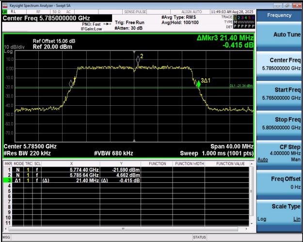
11AX20MIMO-Ant2-5785
