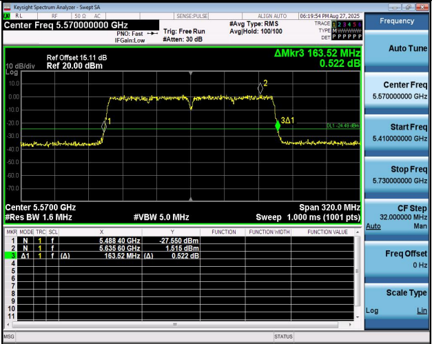
11AC160MIMO-Ant2-5570
