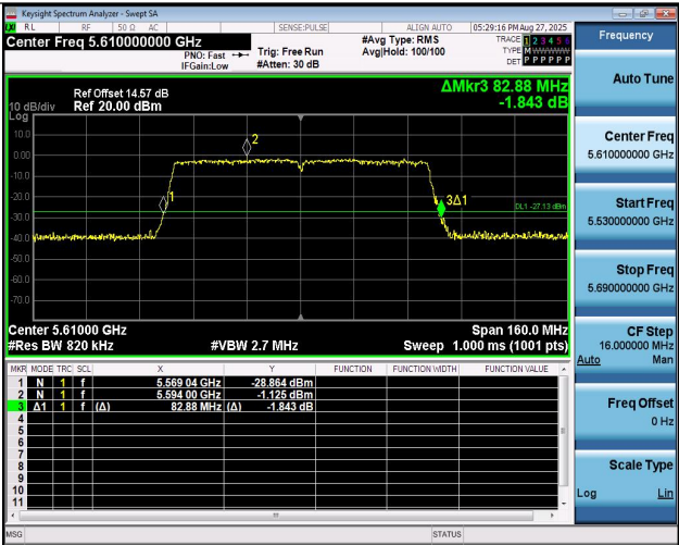
11AC80MIMO-Ant1-5610
