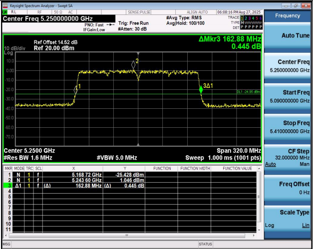
11AC160MIMO-Ant2-5250
