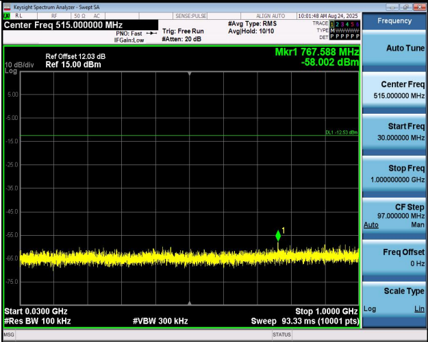
11B-Ant1-2437-30~1000-PASS
