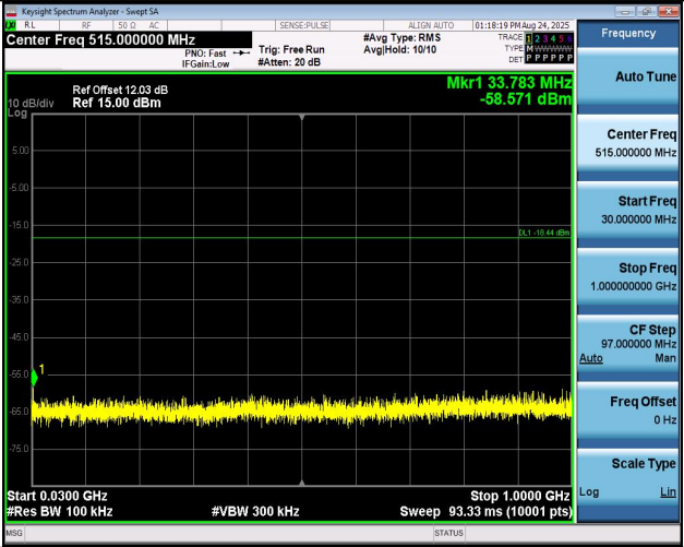
11N20MIMO-Ant1-2437-30~1000-PASS
