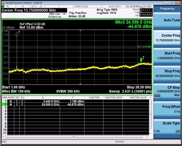
11N20MIMO-Ant1-2437-1000~26500-PASS
