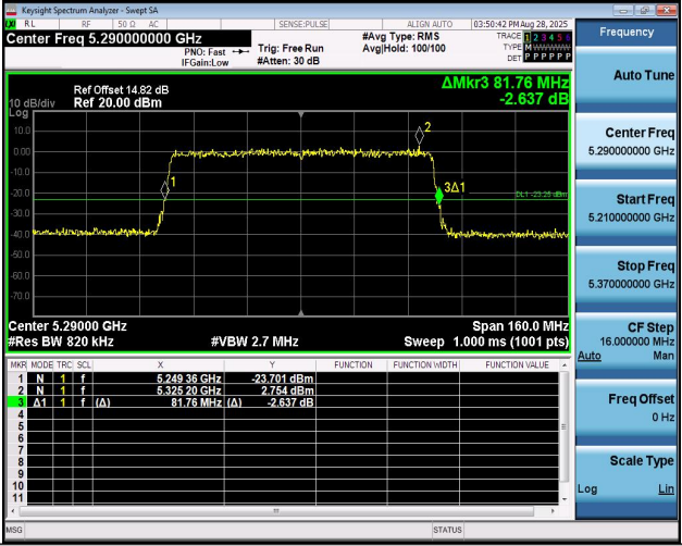
11AX80MIMO-Ant2-5290
