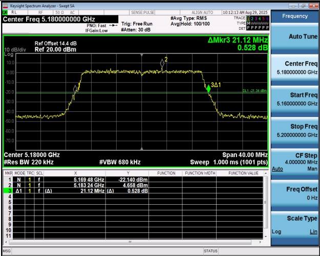
11BE20MIMO-Ant2-5180
