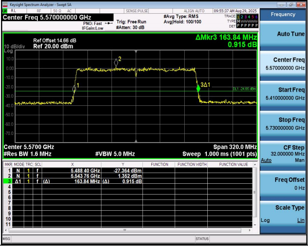
11AX160MIMO-Ant1-5570
