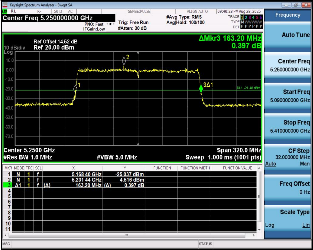
11AX160MIMO-Ant2-5250
