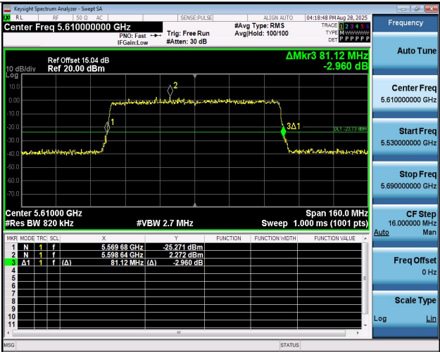
11AX80MIMO-Ant2-5610
