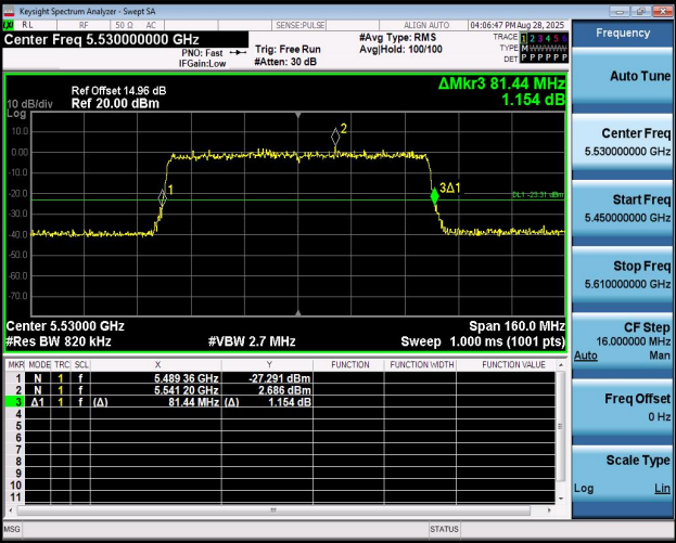
11AX80MIMO-Ant2-5530
