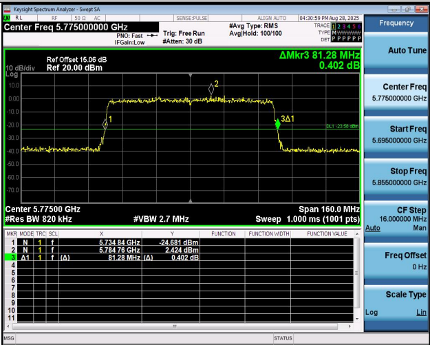
11AX80MIMO-Ant2-5775
