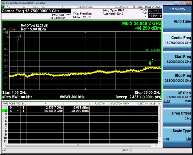
11AX20MIMO-Ant1-2437-1000~26500-PASS
