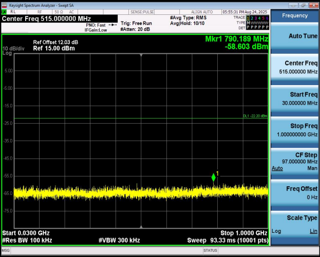
11AX40MIMO-Ant1-2437-30~1000-PASS
