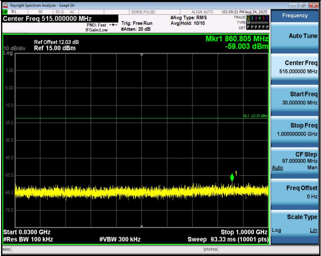
11N40MIMO-Ant1-2437-30~1000-PASS
