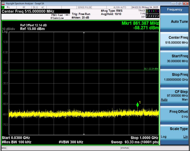
11N40MIMO-Ant1-2452-30~1000-PASS
