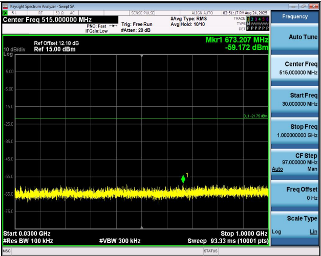
11N40MIMO-Ant2-2437-30~1000-PASS
