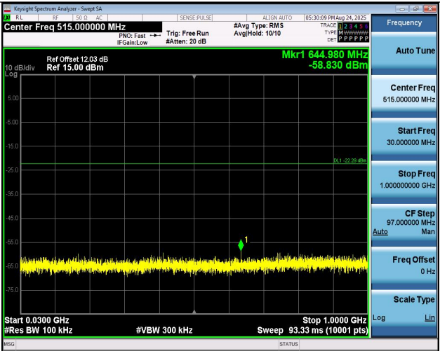
11AX40MIMO-Ant1-2422-30~1000-PASS
