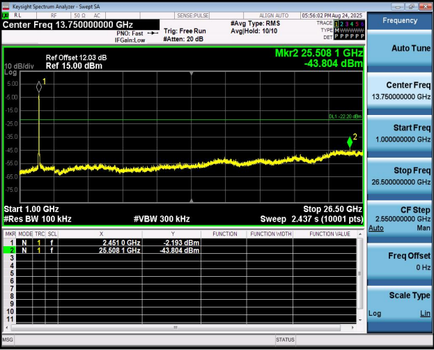
11AX40MIMO-Ant1-2437-1000~26500-PASS
