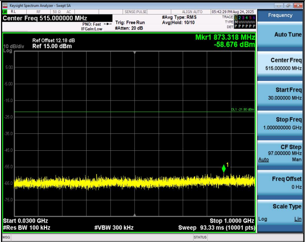
11AX40MIMO-Ant2-2422-30~1000-PASS
