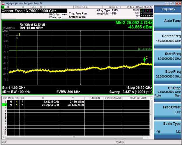
11N40MIMO-Ant2-2452-1000~26500-PASS
