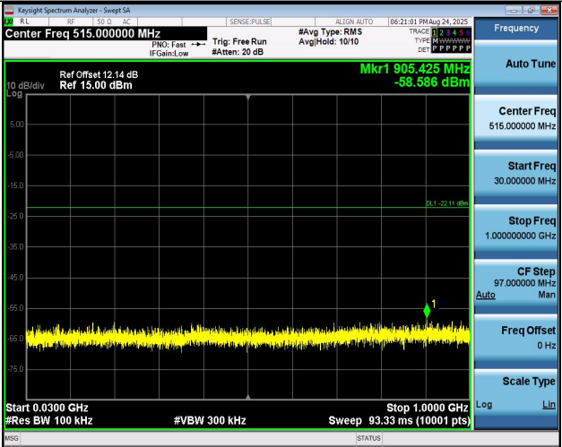
11AX40MIMO-Ant1-2452-30~1000-PASS
