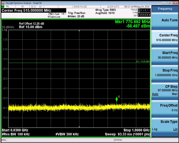
11AX20MIMO-Ant2-2462-30~1000-PASS
