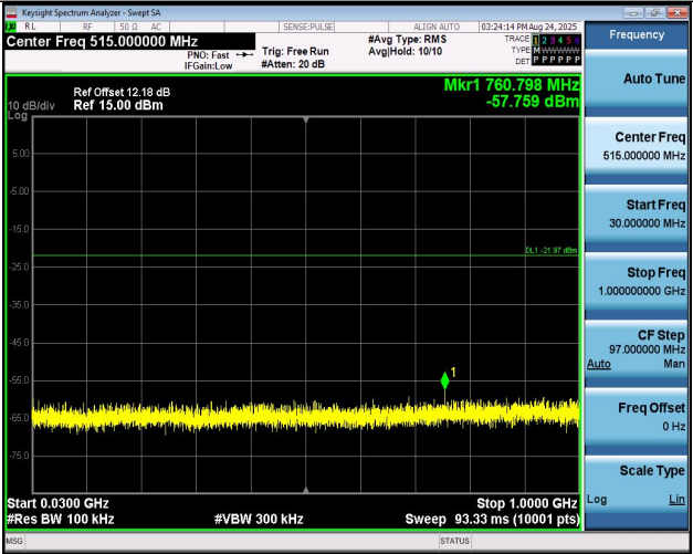
11N40MIMO-Ant2-2422-30~1000-PASS
