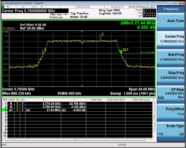
11BE20MIMO-Ant2-5785
