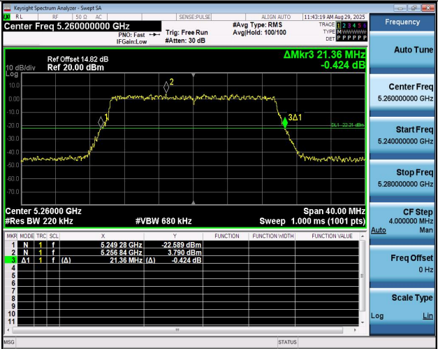
11BE20MIMO-Ant2-5260
