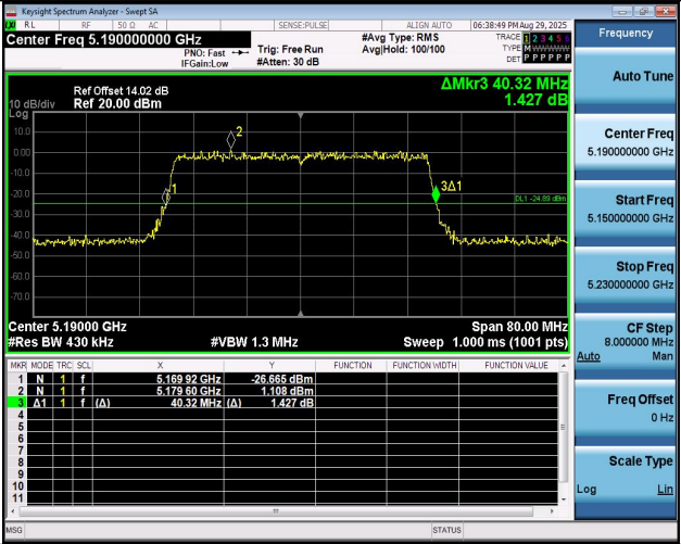
11BE40MIMO-Ant1-5190
