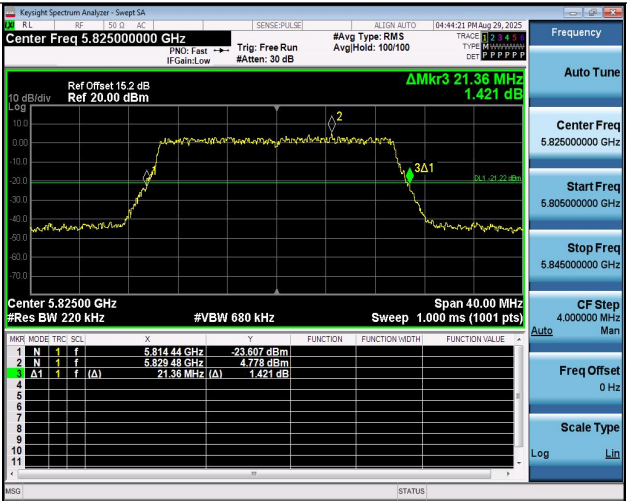
11BE20MIMO-Ant2-5825
