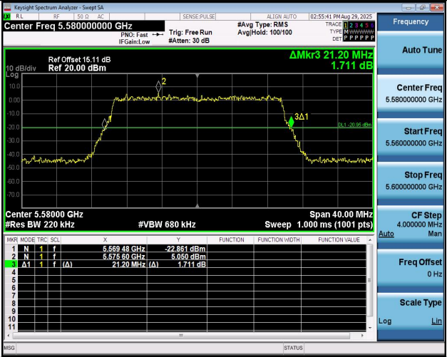
11BE20MIMO-Ant2-5580
