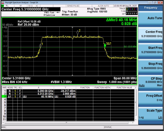
11BE40MIMO-Ant2-5310
