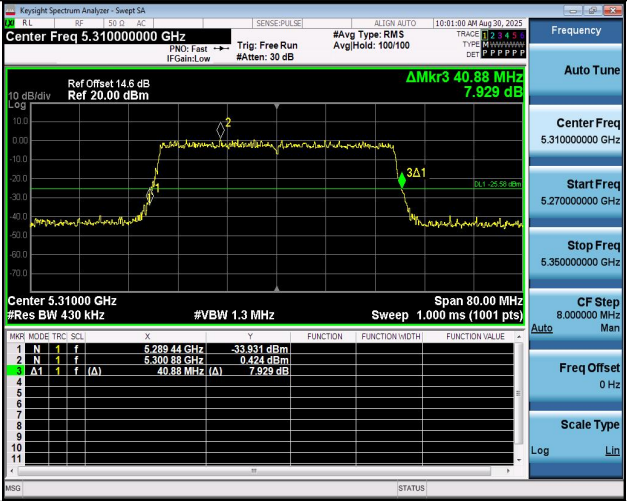
11BE40MIMO-Ant1-5310
