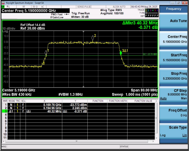
11BE40MIMO-Ant2-5190
