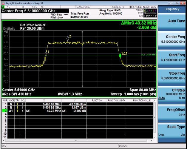
11BE40MIMO-Ant2-5510
