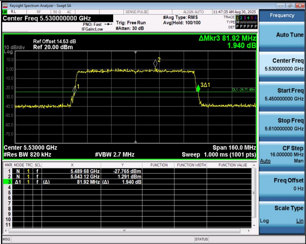
11BE80MIMO-Ant1-5530
