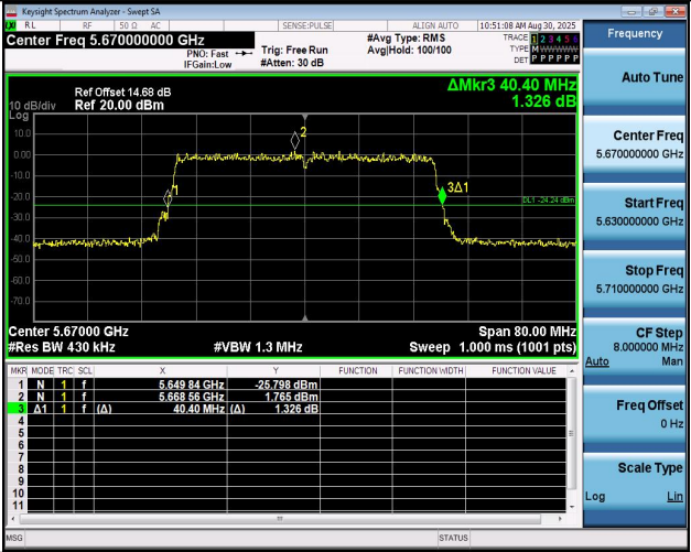
11BE40MIMO-Ant1-5670
