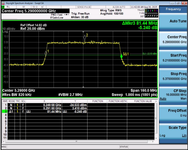
11BE80MIMO-Ant2-5290
