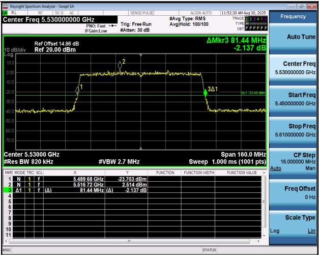
11BE80MIMO-Ant2-5530
