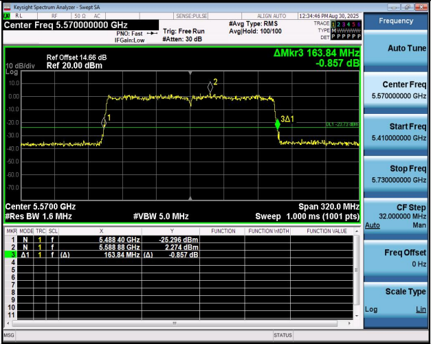
11BE160MIMO-Ant1-5570
