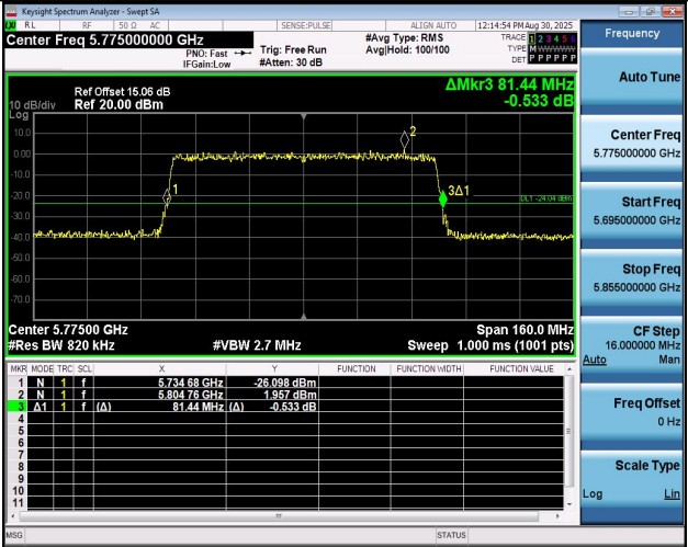
11BE80MIMO-Ant2-5775
