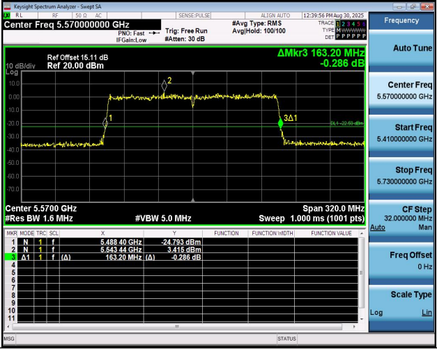
11BE160MIMO-Ant2-5570
