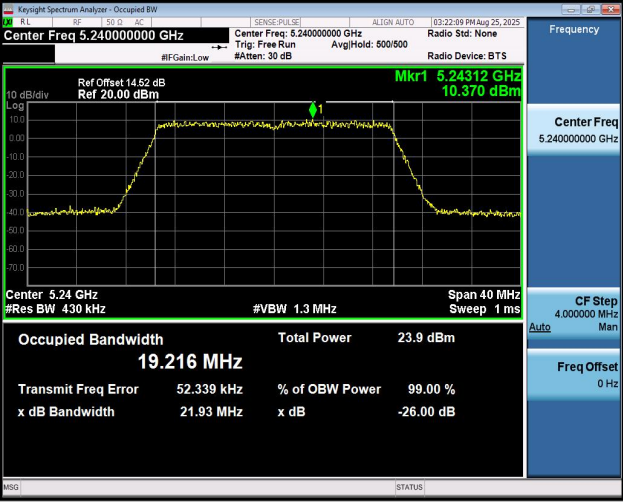
11A-Ant2-5240
