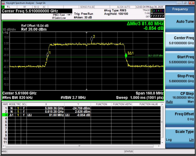
11BE80MIMO-Ant2-5610
