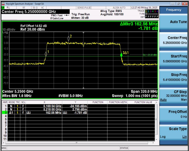
11BE160MIMO-Ant2-5250
