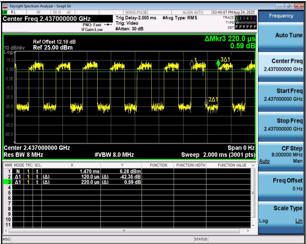
NTVN-11N40MIMO-Ant2-2437
