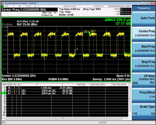
NTNV-11N40MIMO-Ant1-2422
