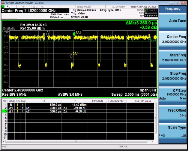
NTNV-11AX20MIMO-Ant2-2462
