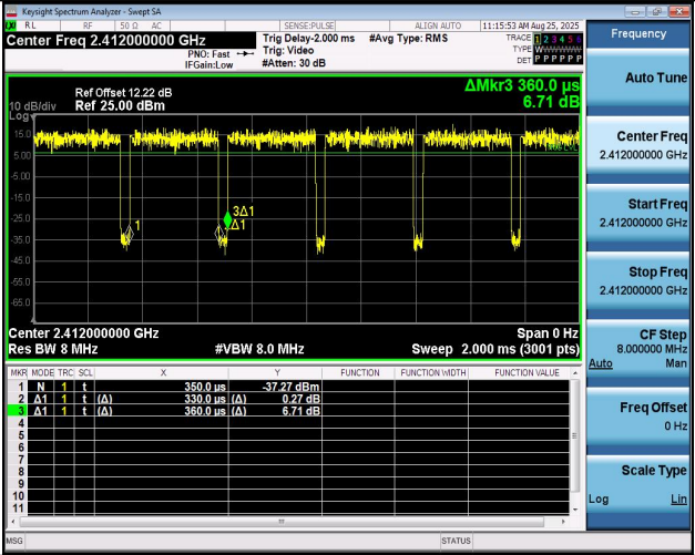
NTNV-11BE20MIMO-Ant2-2412
