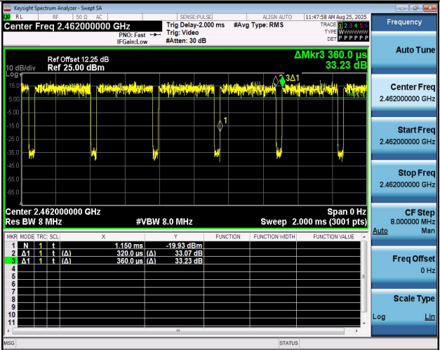
NTNV-11BE20MIMO-Ant2-2462
