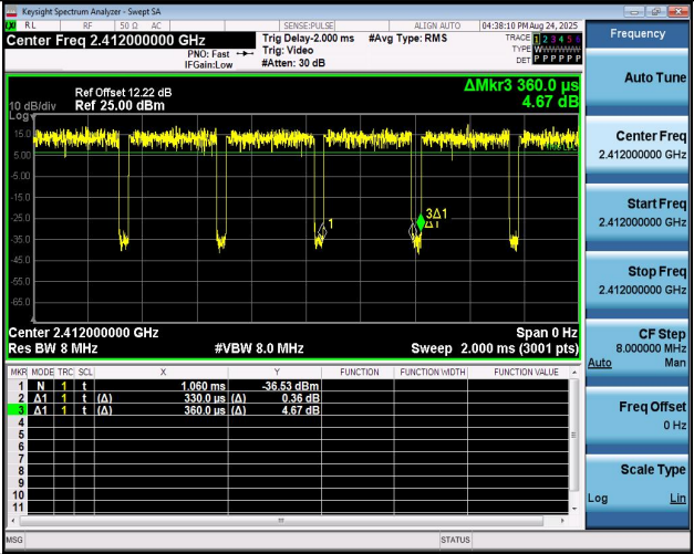
NTNV-11AX20MIMO-Ant2-2412
