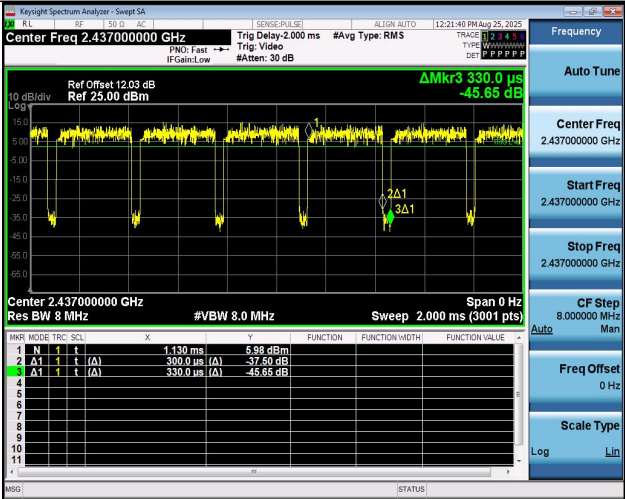
NTNV-11BE40MIMO-Ant1-2437
