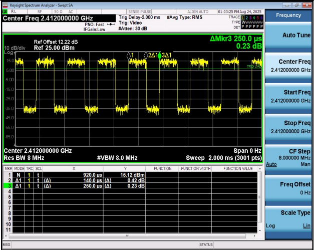
NTNV-11N20MIMO-Ant2-2412
