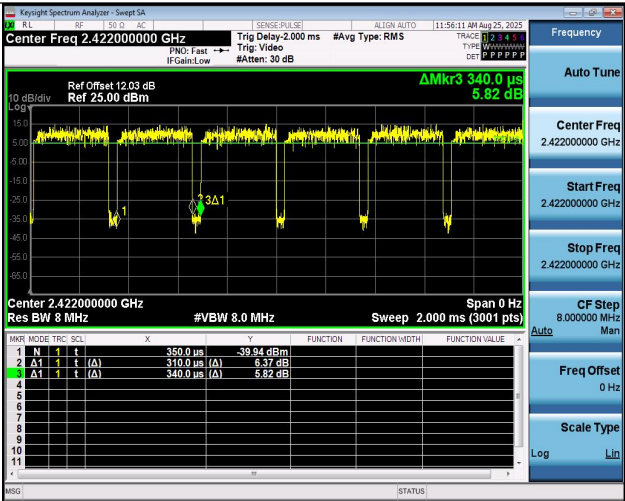
NTNV-11BE40MIMO-Ant1-2422
