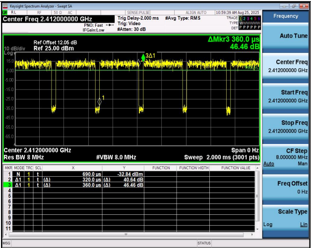
NTNV-11BE20MIMO-Ant1-2412
