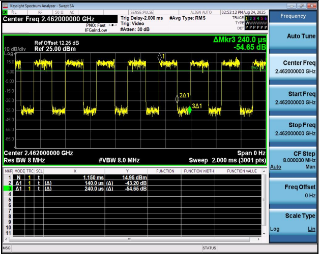
NTNV-11N20MIMO-Ant2-2462
