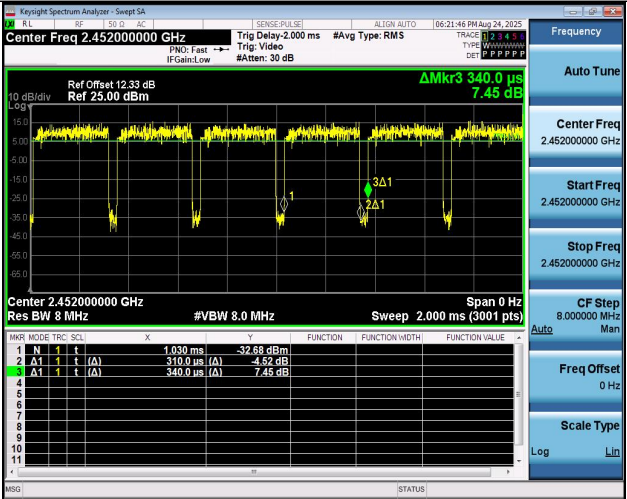
NTNV-11AX40MIMO-Ant2-2452
