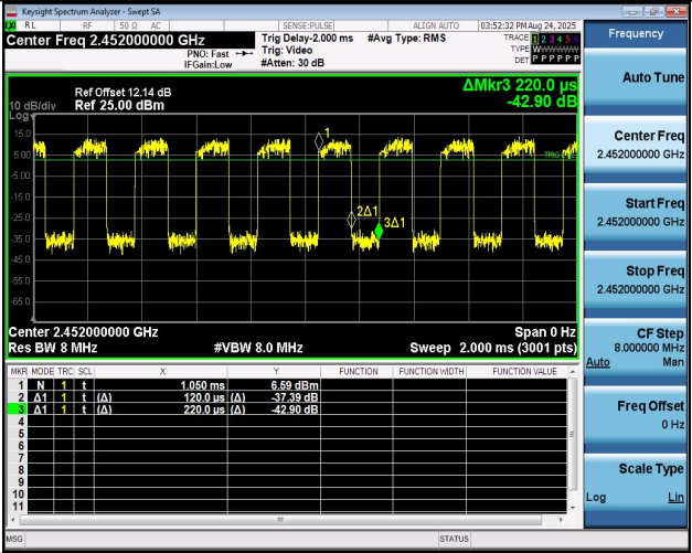
NTVN-11N40MIMO-Ant1-2452
