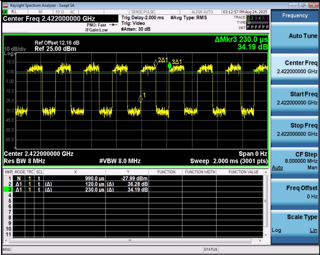
NTNV-11N40MIMO-Ant2-2422
