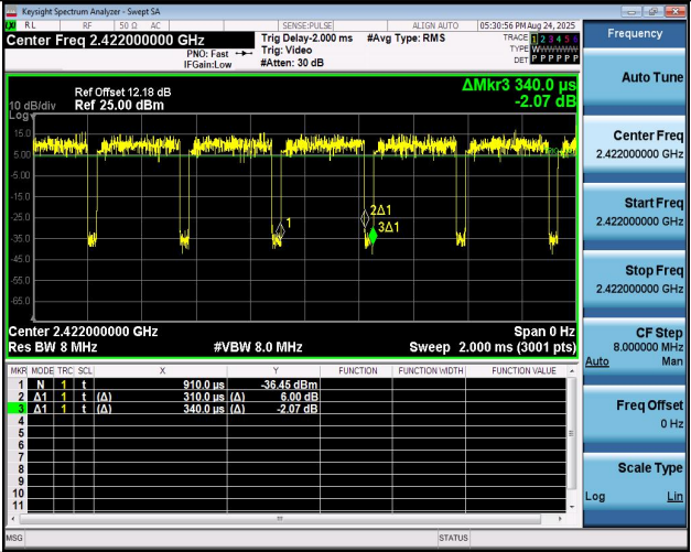
NTNV-11AX40MIMO-Ant2-2422
