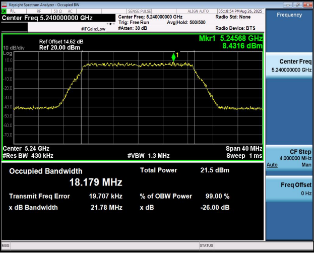
11N20MIMO-Ant2-5240
