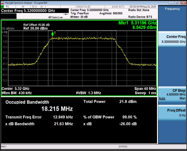
11N20MIMO-Ant2-5320
