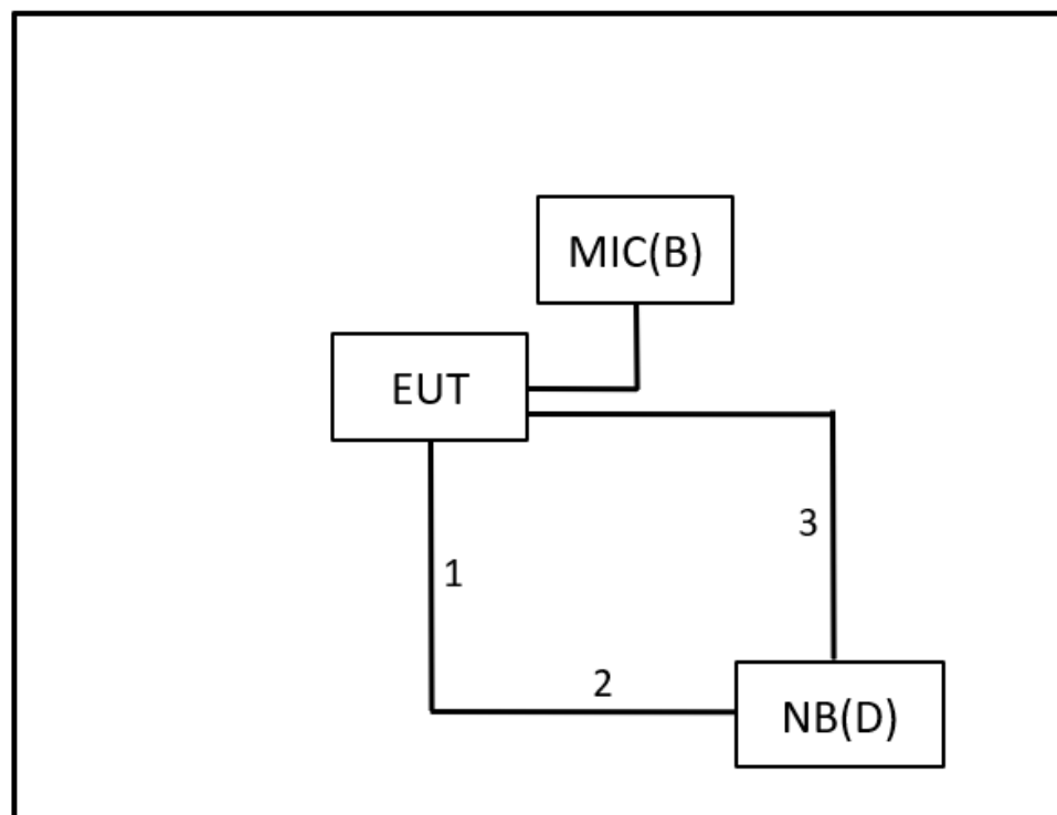
Radiated Emissions
