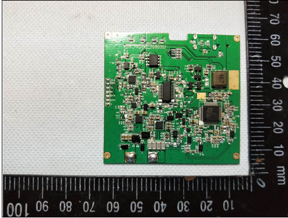
PCB
