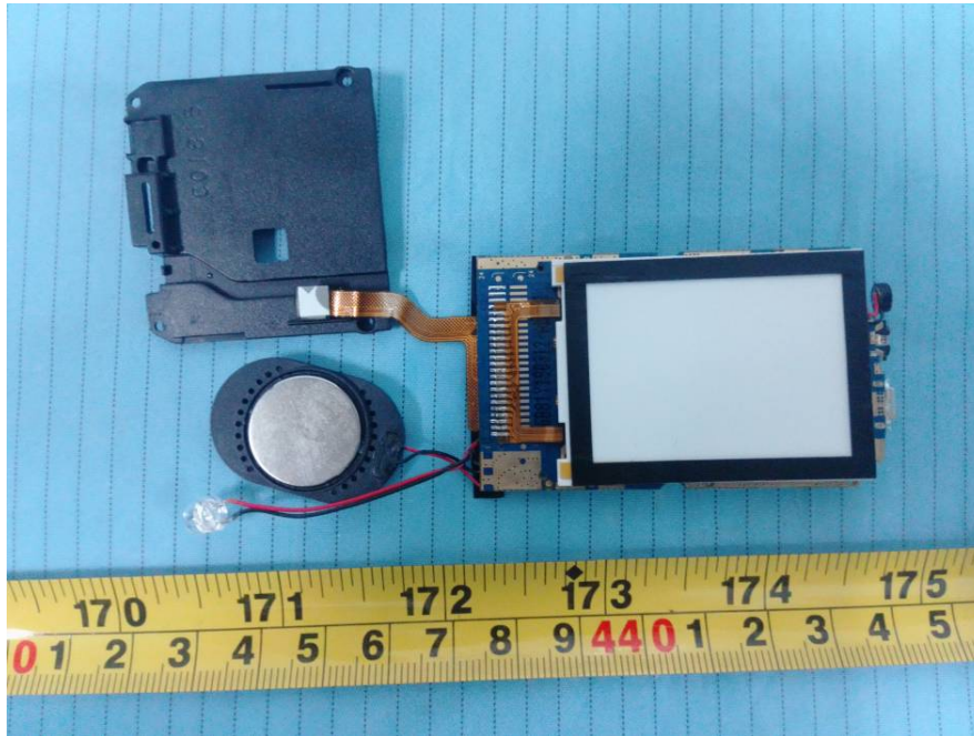
EUT – Main Board Top View 4
