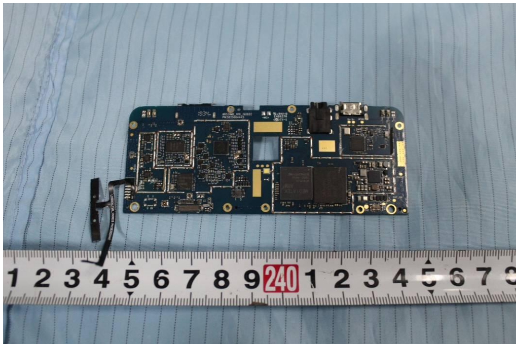
EUT –Main Board Bottom Shilding off View
