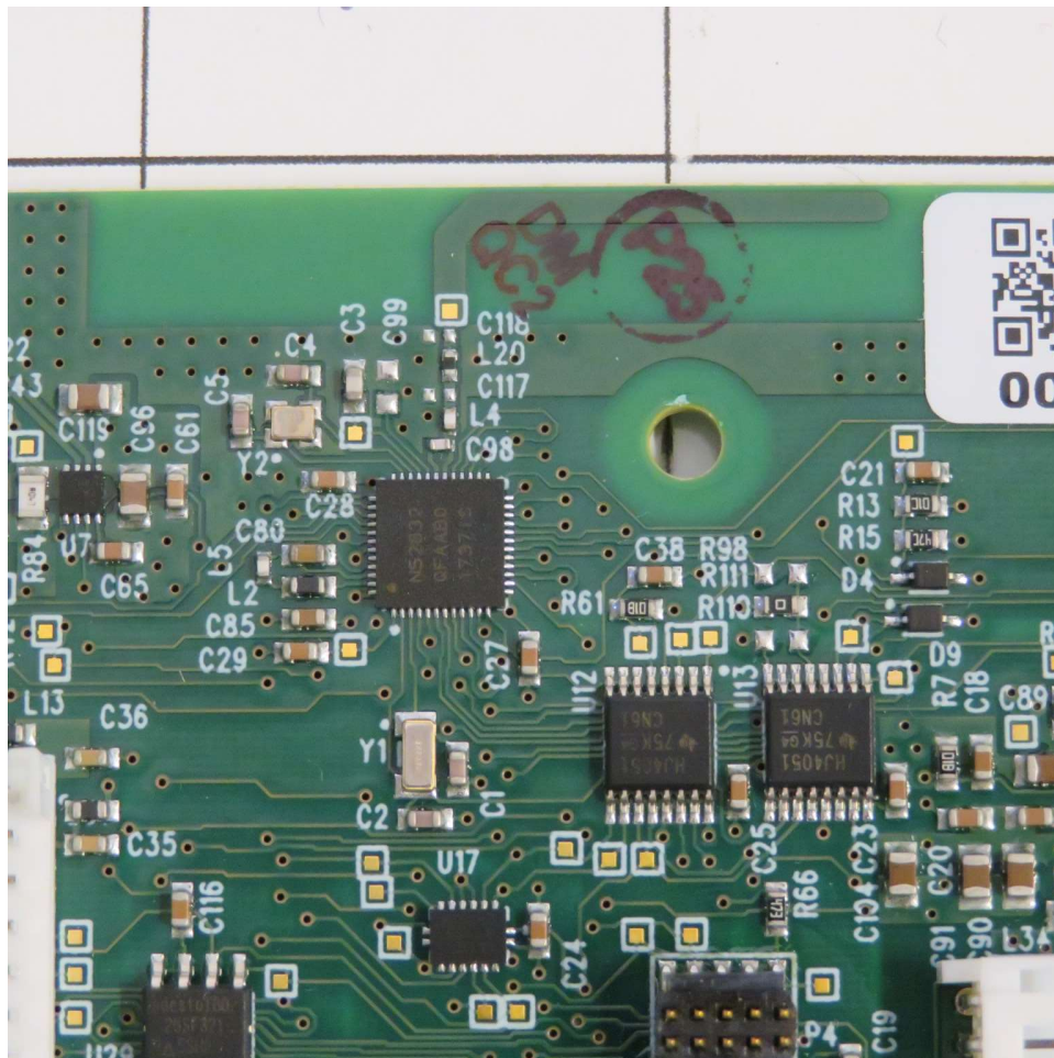
BLE Processor Board – Top View showing BLE processor and antenna
