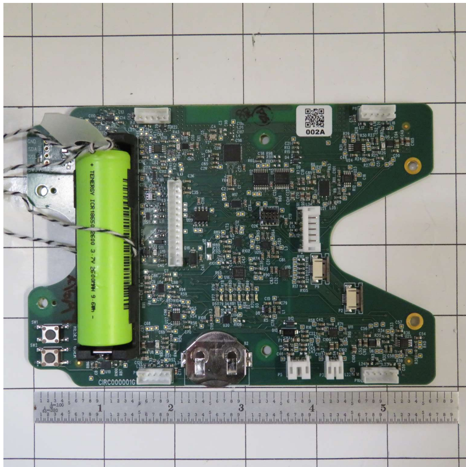
BLE Processor Board - Top View
