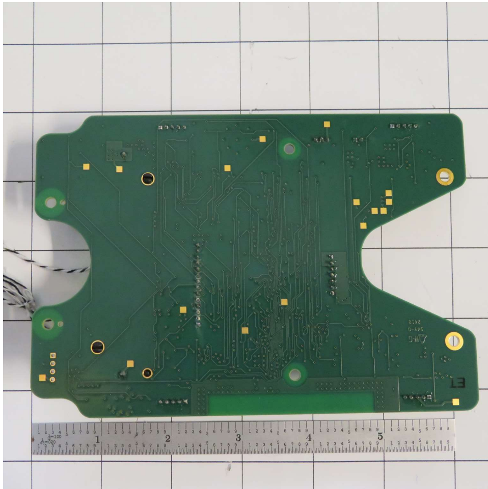
BLE Processor Board – Bottom View
