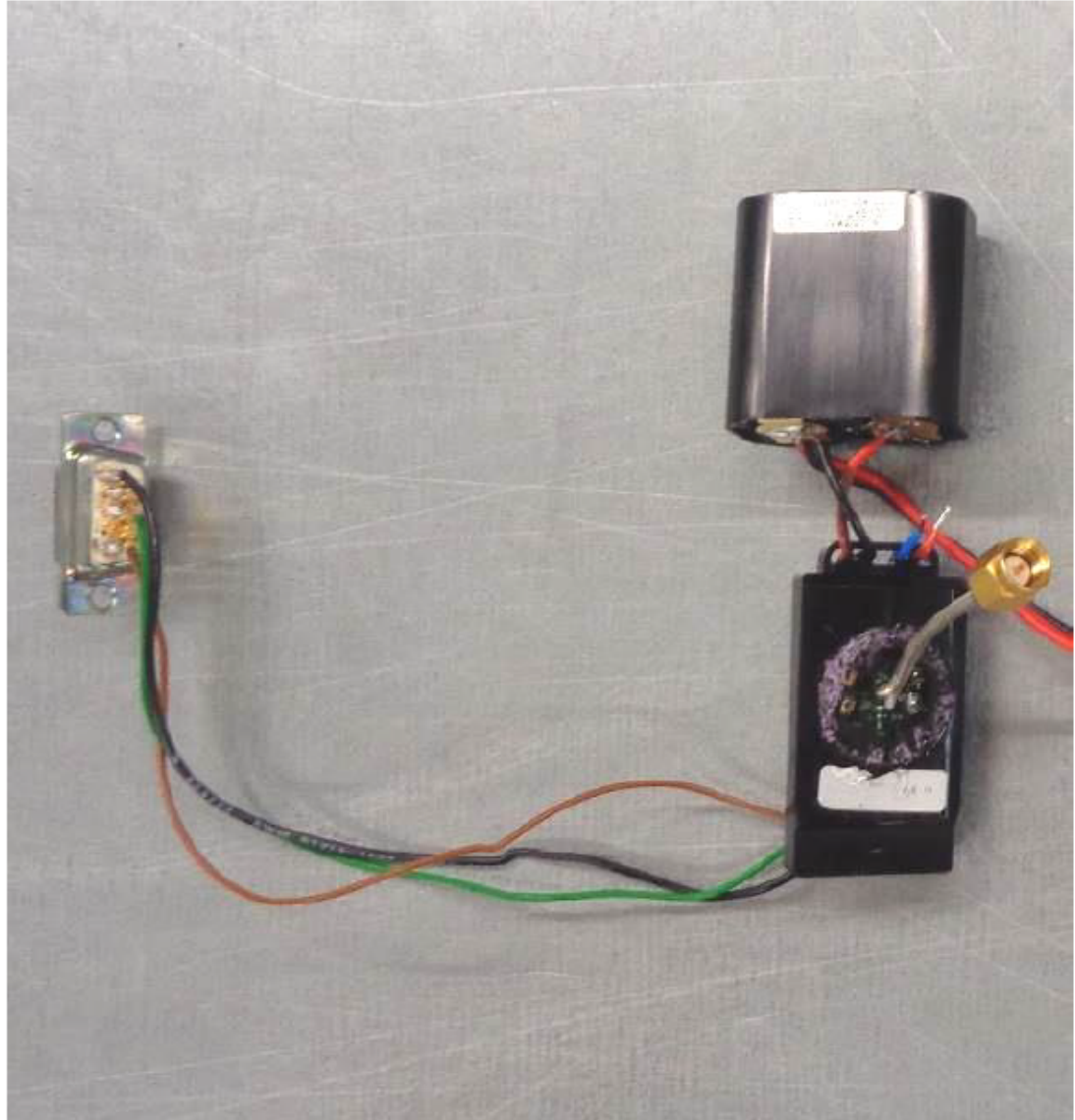
RF module (Prototype 2) with temporary antenna connector (top view)
