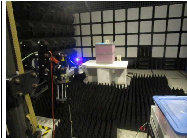
18-40 GHz
