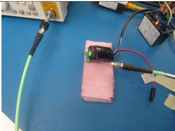
Conducted Bench Setup
