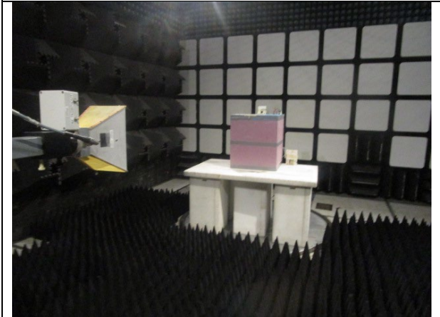
1-4 GHz
