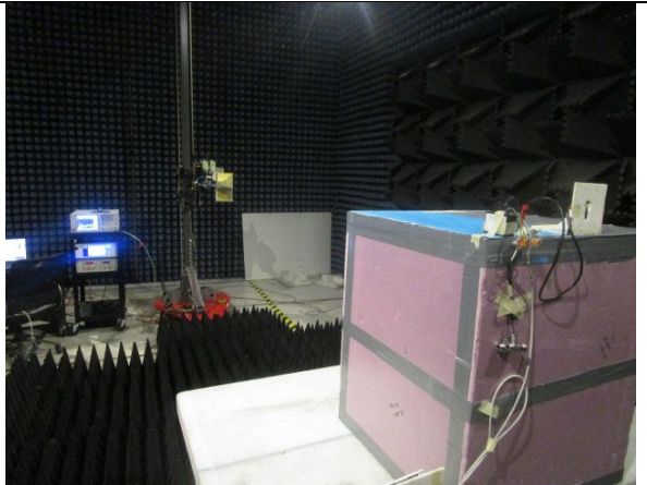
4-18 GHz
