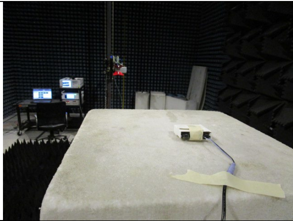
Spurious Emissions 4-18GHz
