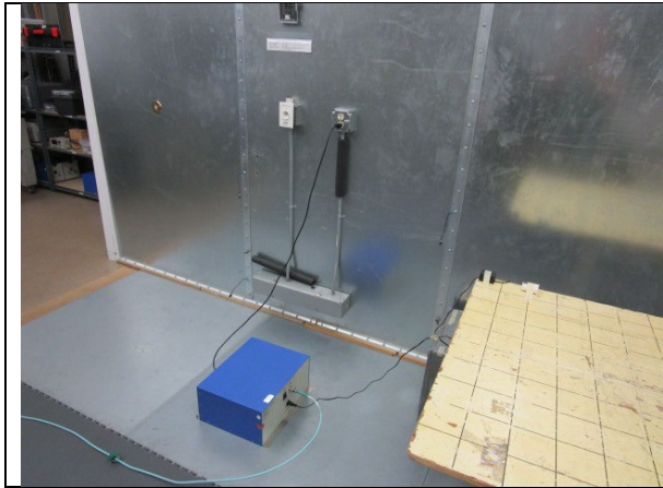
AC Mains Conducted Emissions 15.207
