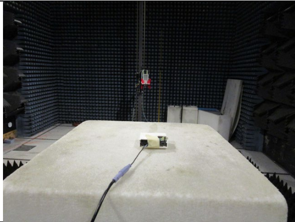
Spurious Emissions 1-4GHz
