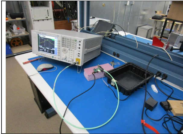
RF Conducted Bench Setup
