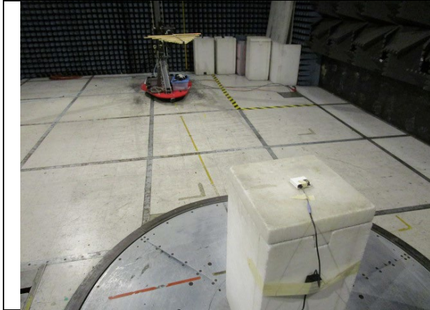
Spurious Emissions 200-1000 MHz
