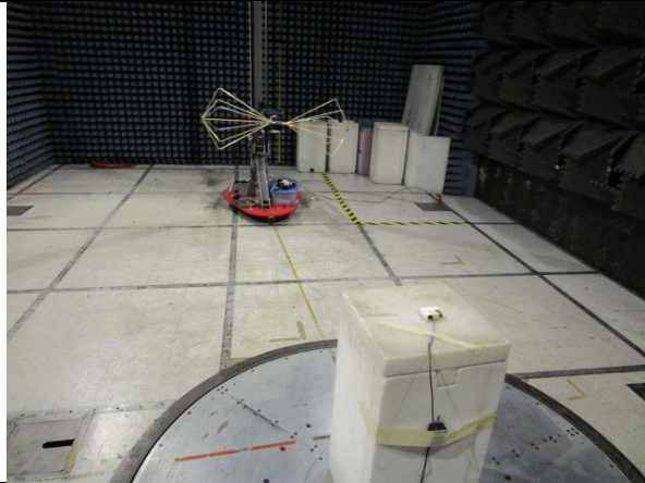
Spurious Emissions 30-200 MHz
