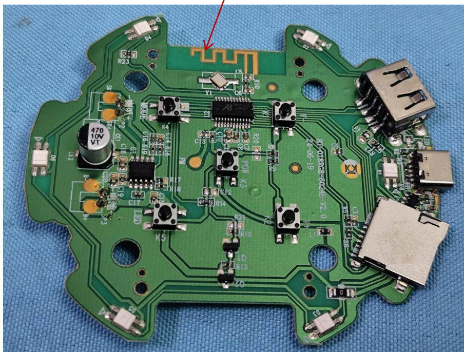
BT ANT+FM RX ANT
