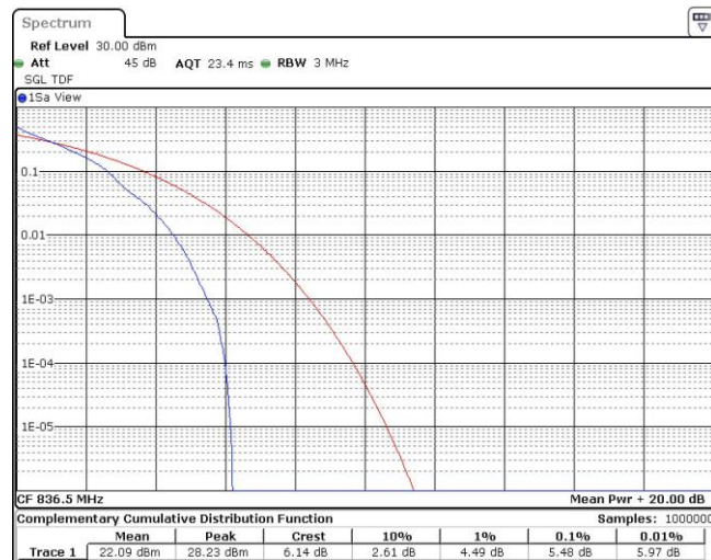
Band5-1.4MHz-QPSK-20525-6RB#0
