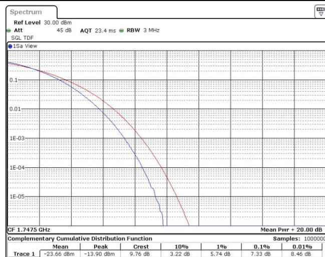
Band4-15MHz-16QAM-20325-75RB#0
