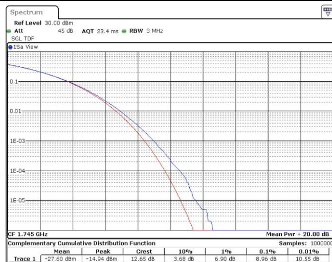
Band66-15MHz-QPSK-132322-75RB#0
