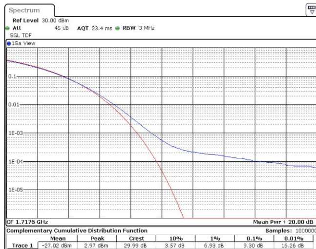
Band66-15MHz-16QAM-132047-75RB#0
