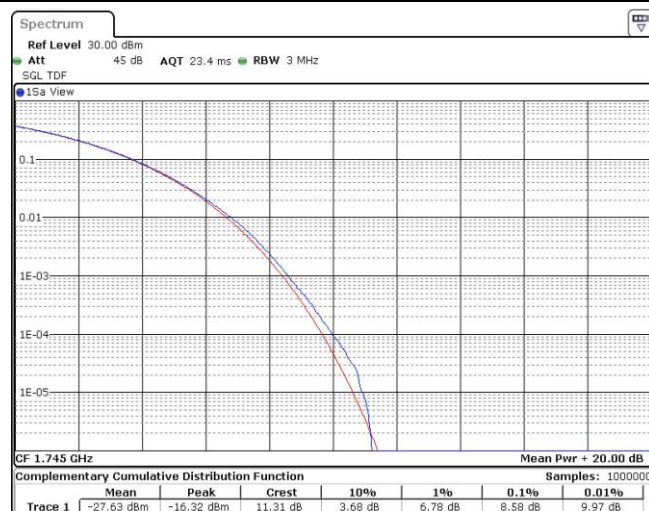
Band66-20MHz-16QAM-132322-1RB#0
