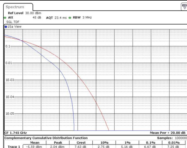
Band66-10MHz-16QAM-132322-1RB#0
