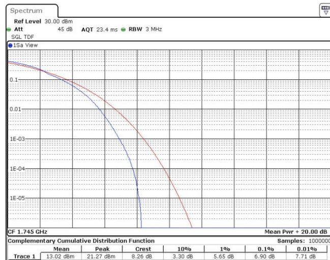
Band66-15MHz-16QAM-132597-1RB#0
