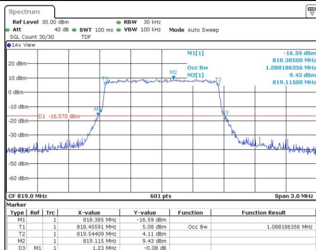
Band26-1.4MHz-QPSK-26783-6RB#0
