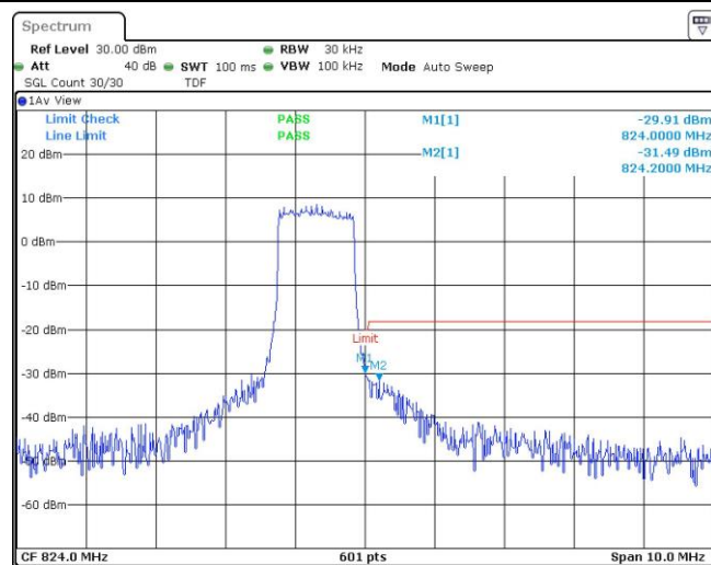
Band26-1.4MHz-16QAM-26797-1RB#0
