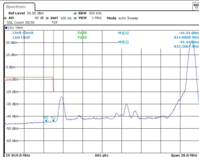
Band26-15MHz-QPSK-26765-75RB#0
