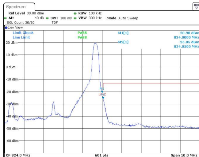
Band26-5MHz-QPSK-26765-25RB#0
