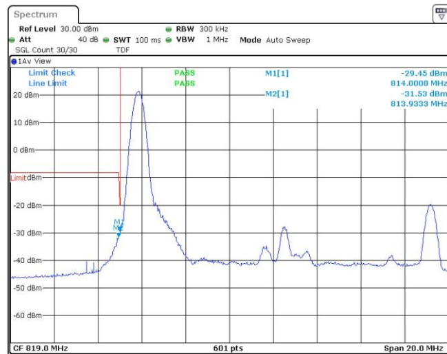
Band26-15MHz-QPSK-26765-1RB#74
