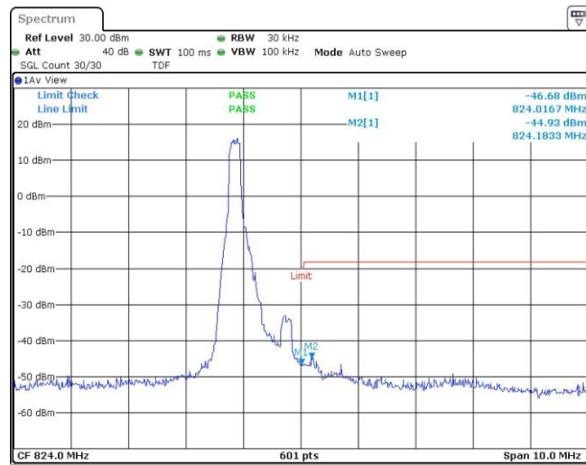
Band26-1.4MHz-16QAM-26783-1RB#5
