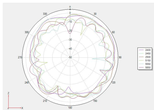
Phi 0 2D
