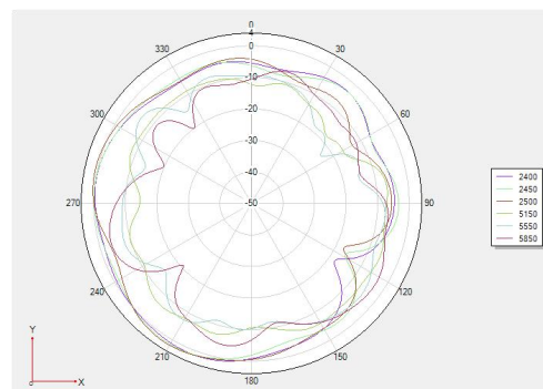
Theta 90 2D
