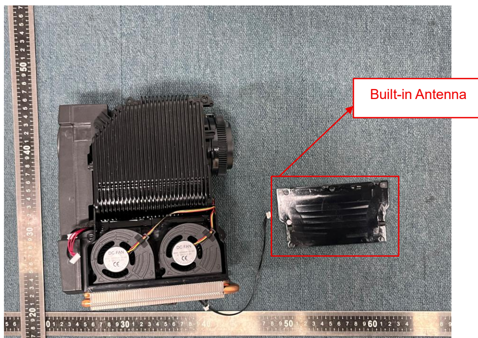
EUT UNCOVER VIEW 7
