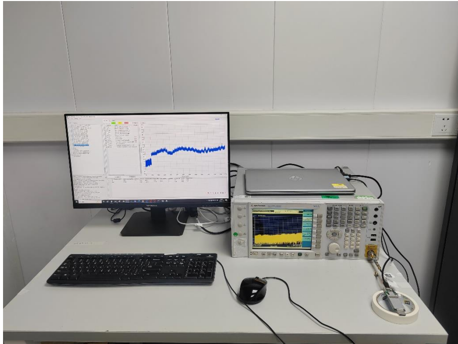
Conducted Test-BT/WIFI
