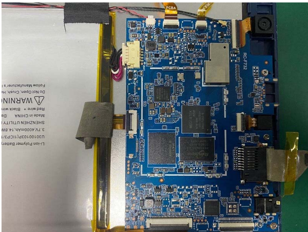
Mainboard Model No.: RS512M32LM4D2BDS-53BT 2GB & EMMC32G-TA28 32GB
