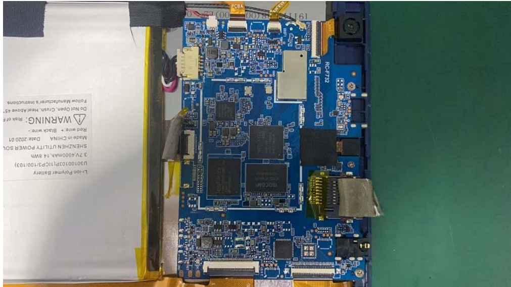
Mainboard Model No.: MDXC1016G-M2 2GB & LTMZ0007HF-DAB1-SM
