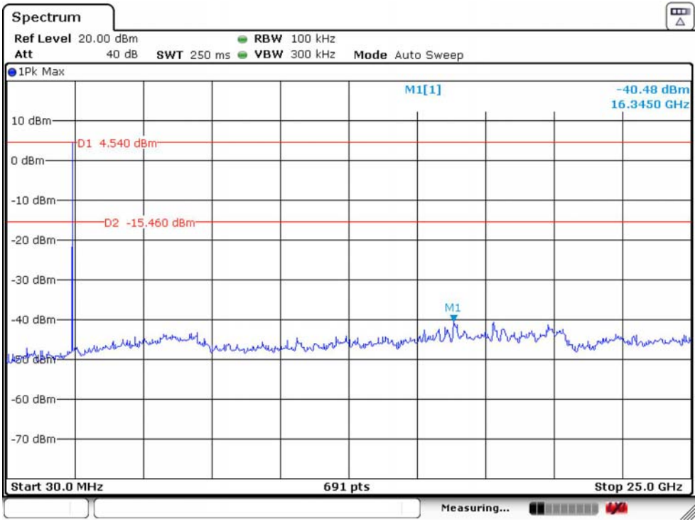
GFSK 2402 MHz 2M
