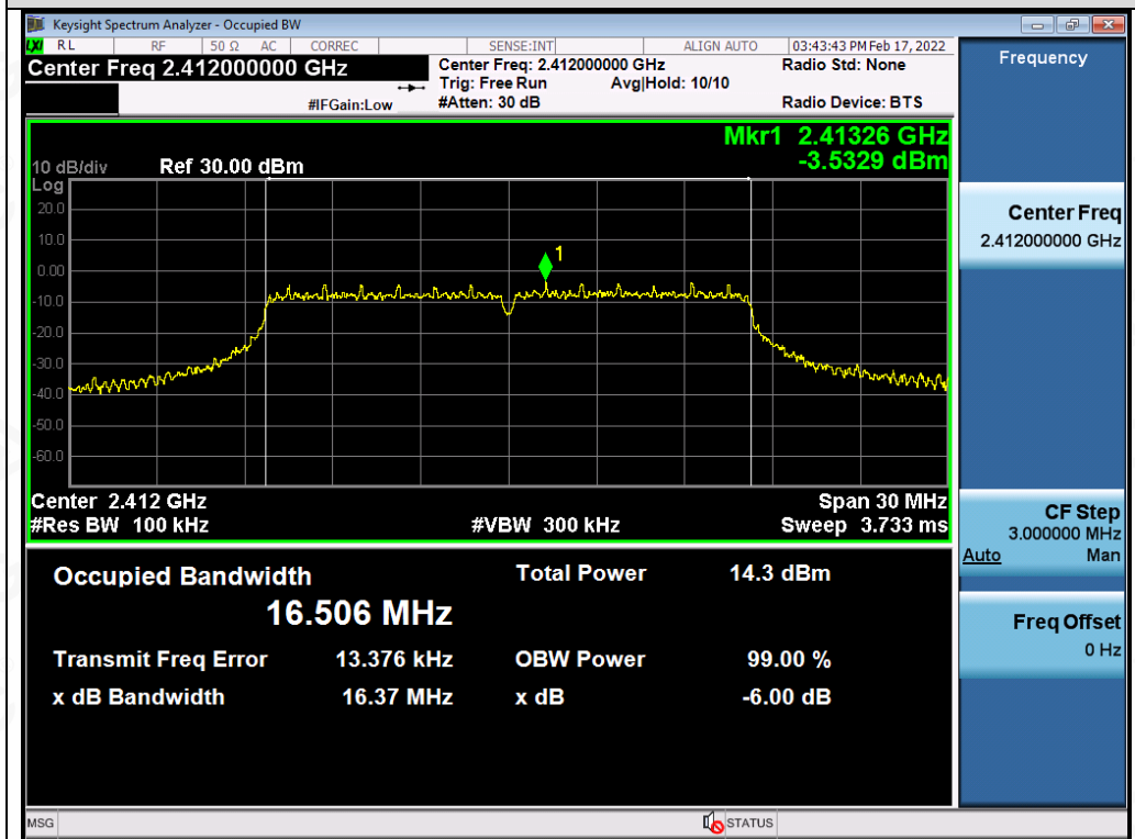
Test_Graph_802.11g_ANT1_2412_6Mbps_DTSSBW
