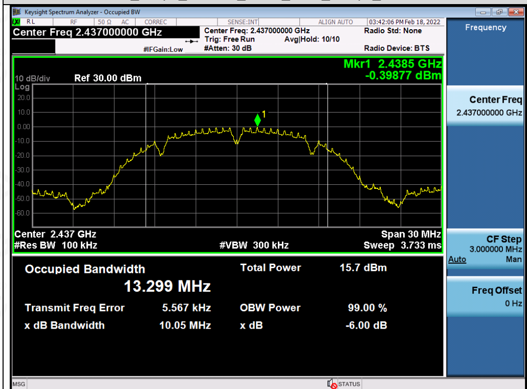
Test_Graph_802.11b_ANT1_2437_1Mbps_DTSBW
