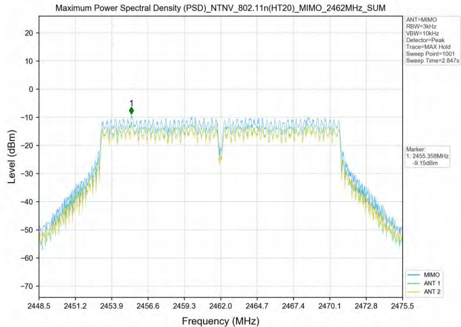
802.11n(HT20)_2462MHz_MIMO_Total
