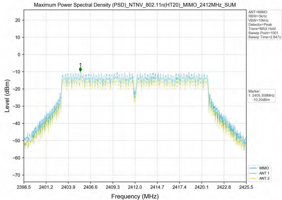
802.11n(HT20)_2412MHz_MIMO_Total
