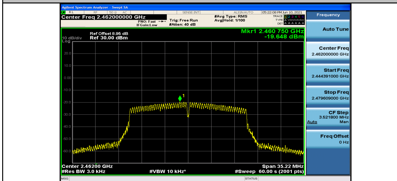
Maximum(average) power spectral density_11N20MIMO_2462_Ant2
