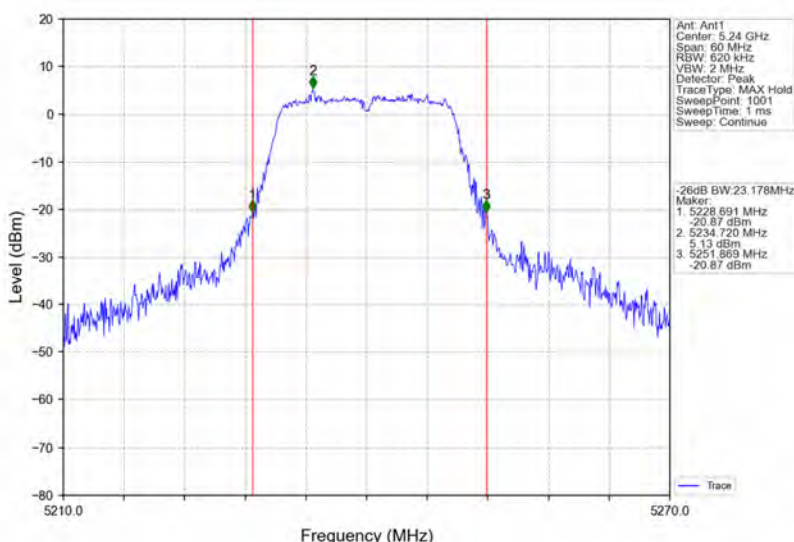
802.11n(HT20)_HCH_5240MHz_Ant1_NTNV
