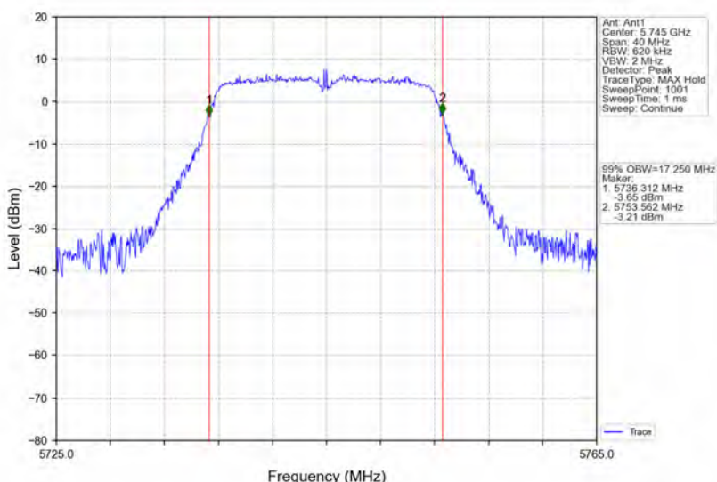
802.11a_LCH_5745MHz_Ant1_NTNV
