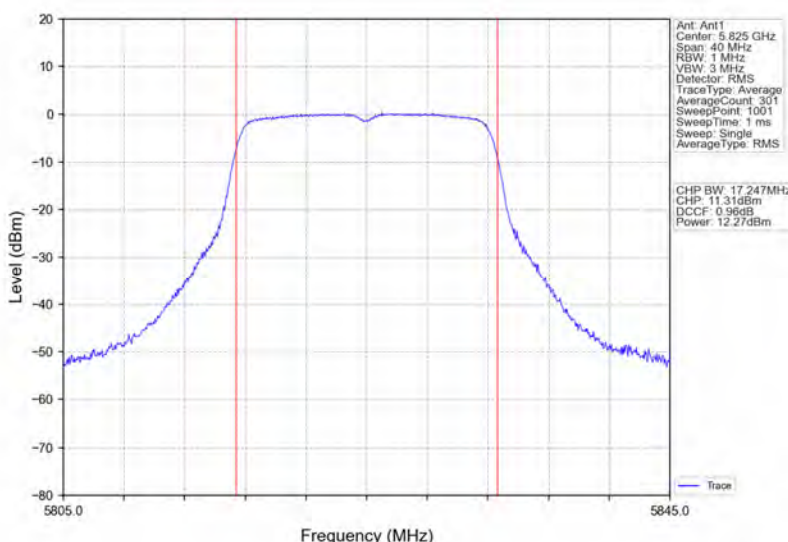
802.11a_HCH_5825MHz_Ant1_NTNV
