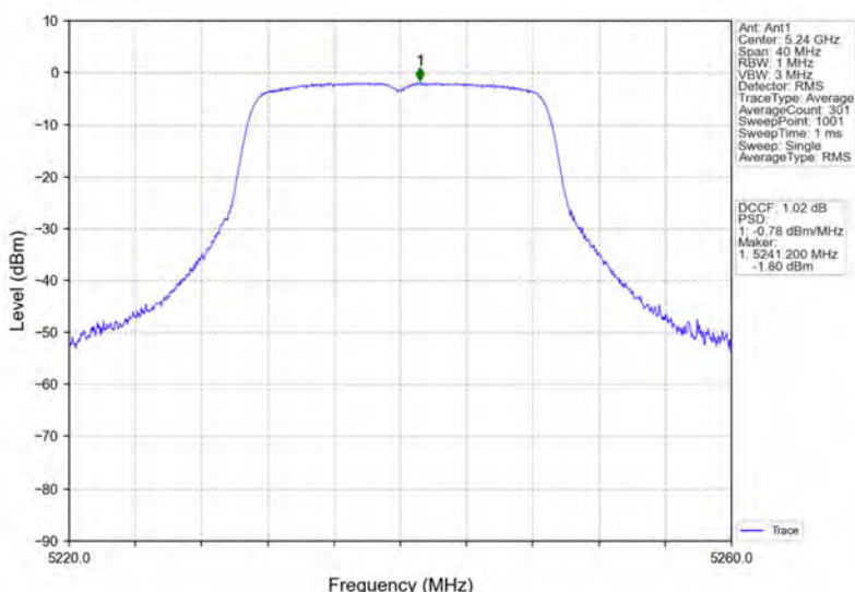
802.11n(HT20)_HCH_5240MHz_Ant1_NTNV
