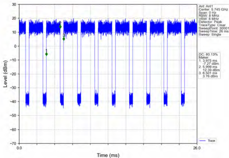
802.11a_LCH_5745MHz_Ant1_NTNV
