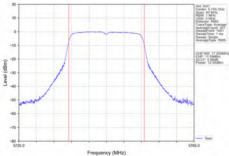
802.11a_LCH_5745MHz_Ant1_NTNV
