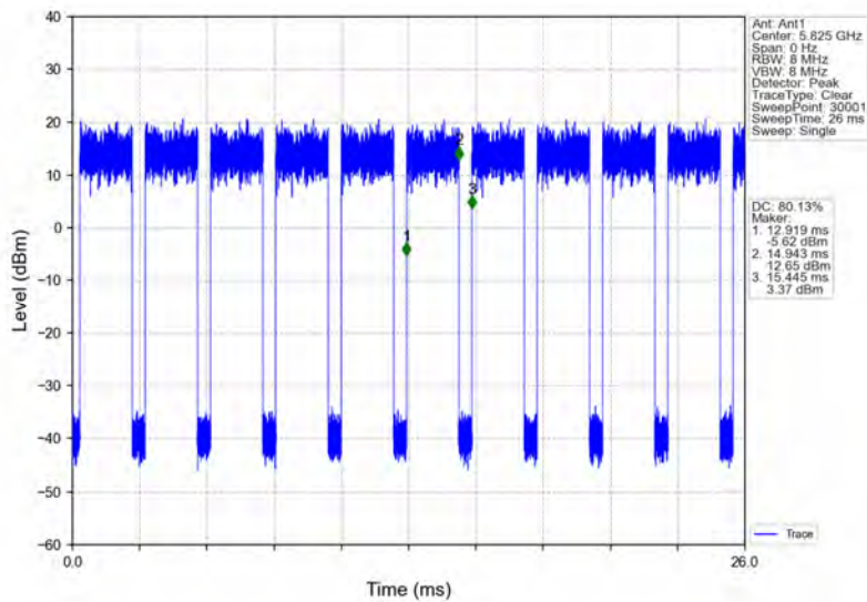
802.11a_HCH_5825MHz_Ant1_NTNV
