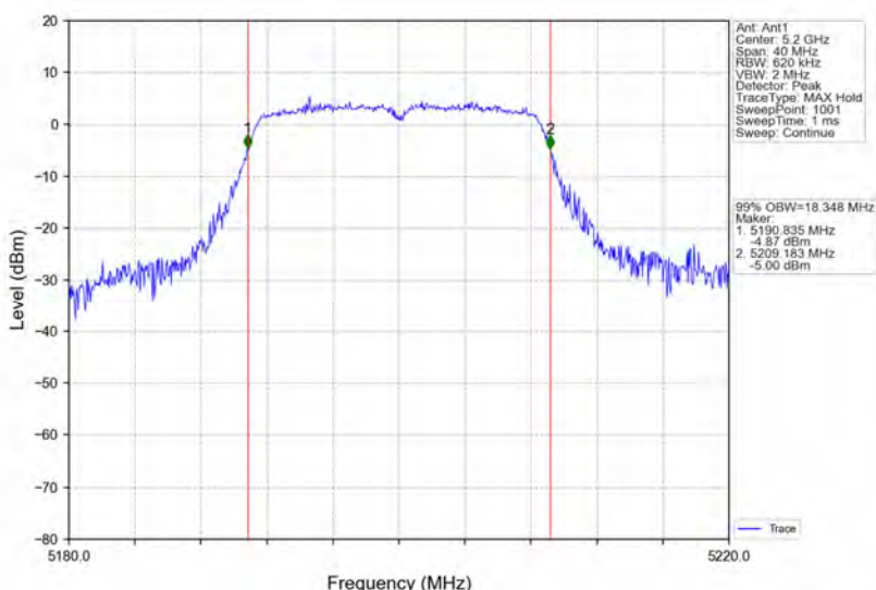
802.11n(HT20)_MCH_5200MHz_Ant1_NTNV
