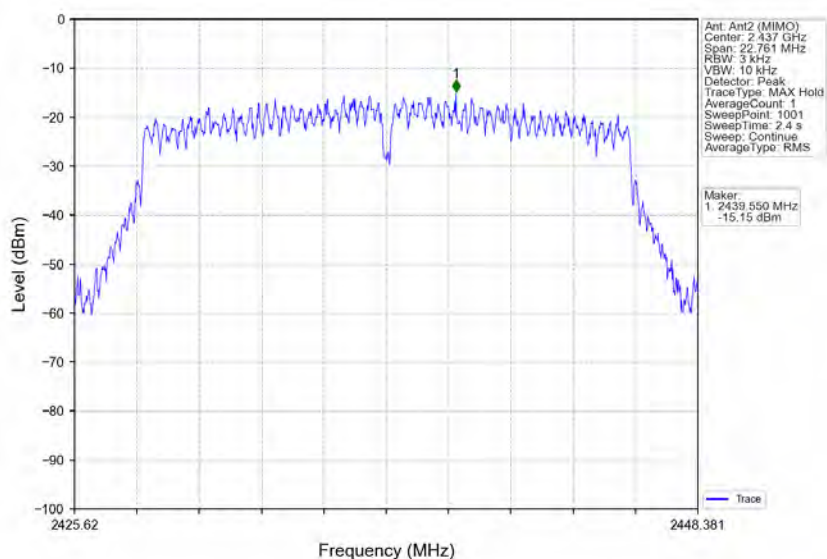
802.11n(HT20)_MCH_2437MHz_MIMO NTN
